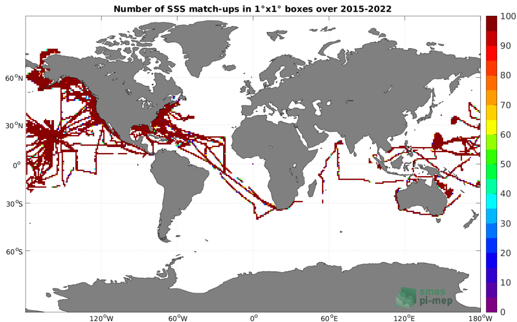
Figure 4: Number of SSS match-ups between TSG (SAMOS) SSS and the SMAP SSS L3 v5 - 8-Day running (RSS) SSS product for the Global Ocean Pi-MEP region over 1^\circ \times 1^\circ boxes and for the full satellite product period.
