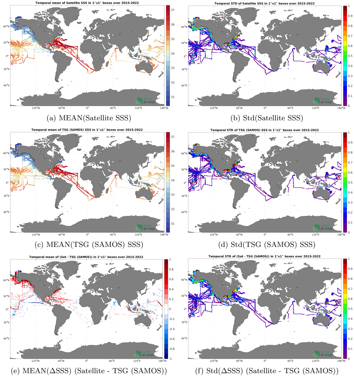
Figure 6: Temporal mean (left) and Std (right) of SSS from SMAP SSS L3 v5 - 8-Day running (RSS) (top), TSG (SAMOS) (middle), and of \Delta SSS (Satellite - TSG (SAMOS)). Only match-up pairs are used to generate these maps.
