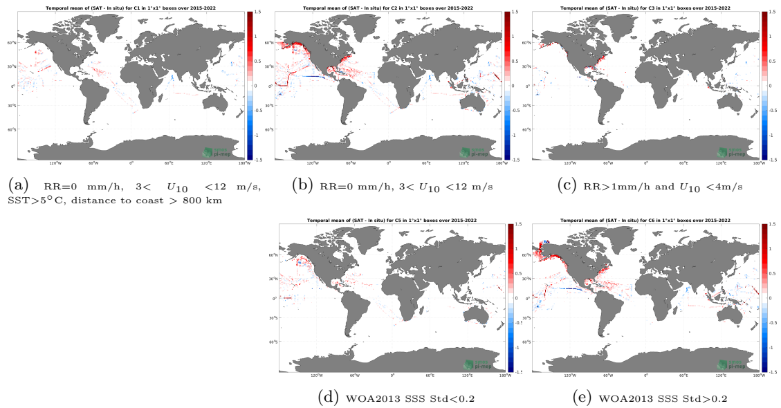
Figure 12: Temporal mean gridded over spatial boxes of size 1^\circ \times 1^\circ of \Delta SSS (SMAP SSS L3 v5 - 8-Day running (RSS) - TSG (SAMOS)) for 5 different subdatasets corresponding to:RR=0 mm/h, 3 < U_{10} < 12 m/s, SST > 5^\circ\text{C} , distance to coast > 800 km (a), RR=0 mm/h, 3 < U_{10} < 12 m/s (b), RR > 1 mm/h and U_{10} < 4 m/s (c), WOA2013 SSS Std < 0.2 (d), WOA2013 SSS Std > 0.2 (e).
