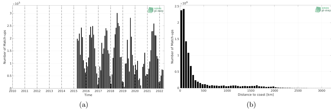
Figure 1: Number of match-ups between TSG (SAMOS) and SMAP SSS L3 v5 - 8-Day running (RSS) SSS as a function of time (a) and as function of the distance to coast (b) over the Global Ocean Pi-MEP region and for the full satellite product period.
