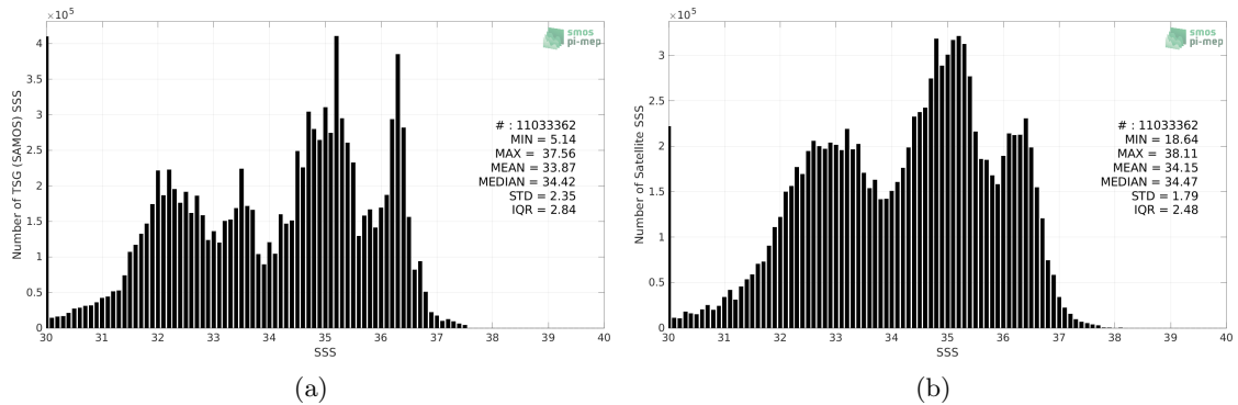
Figure 2: Histograms of SSS from TSG (SAMOS) (a) and SMAP SSS L3 v5 - 8-Day running (RSS) (b) considering all match-up pairs per bins of 0.1 over the Global Ocean Pi-MEP region and for the full satellite product period.
