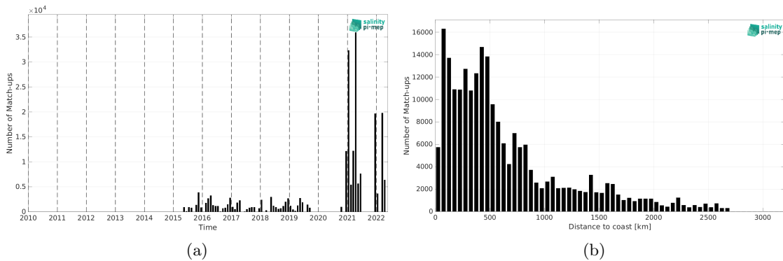
Figure 1: Number of match-ups between TSG (Polarstern) and SMAP SSS L3 v5 - 8-Day running (RSS) SSS as a function of time (a) and as function of the distance to coast (b) over the Global Ocean Pi-MEP region and for the full satellite product period.
