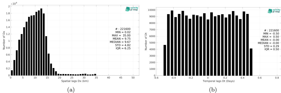
Figure 5: Histograms of the spatial (a) and temporal (b) lags between the location/time of the TSG (Polarstern) measurement and the date of the corresponding SMAP SSS L3 v5 - 8-Day running (RSS) SSS pixel.
