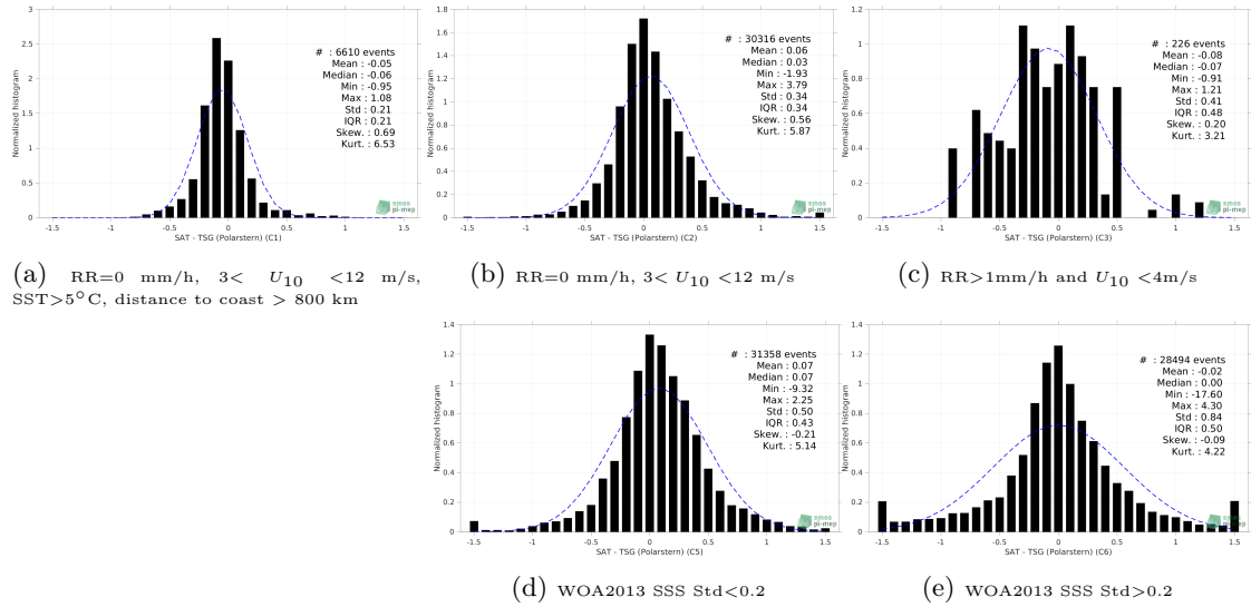
Figure 13: Normalized histogram of \Delta SSS (SMAP SSS L3 v5 - 8-Day running (RSS) - TSG (Polarstern)) for 5 different subdatasets corresponding to: RR=0 mm/h, 3 < U_{10} < 12 m/s, SST > 5°C, distance to coast > 800 km (a), RR=0 mm/h, 3 < U_{10} < 12 m/s (b), RR > 1mm/h and U_{10} < 4 m/s (c), WOA2013 SSS Std < 0.2 (d), WOA2013 SSS Std > 0.2 (e).
