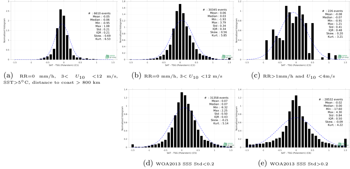
Figure 13: Normalized histogram of \Delta\text{SSS} (SMAP SSS L3 v5 - 8-Day running (RSS) - TSG (Polarstern)) for 5 different subdatasets corresponding to: RR=0 mm/h, 3 < U_{10} < 12 m/s, SST > 5^\circ\text{C} , distance to coast > 800 km (a), RR=0 mm/h, 3 < U_{10} < 12 m/s (b), RR > 1 mm/h and U_{10} < 4 m/s (c), WOA2013 SSS Std < 0.2 (d), WOA2013 SSS Std > 0.2 (e).
