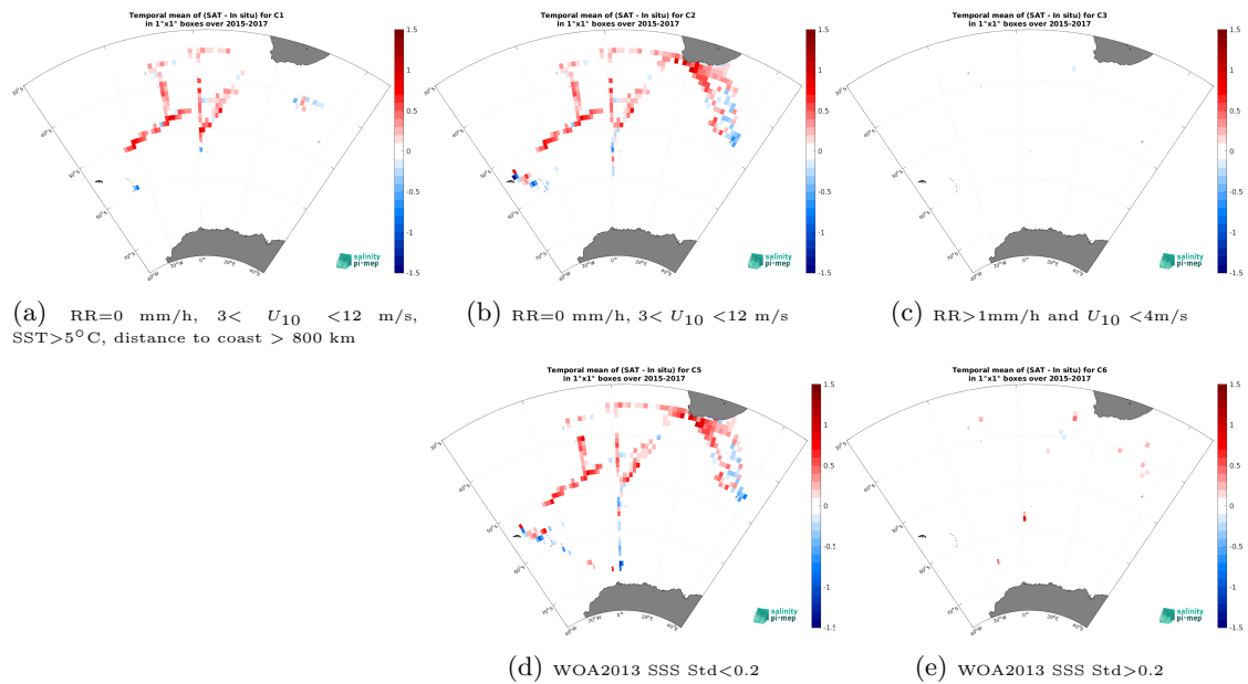
Figure 12: Temporal mean gridded over spatial boxes of size 1^\circ \times 1^\circ of \Delta\text{SSS} (SMAP SSS L3 v5 - 8-Day running (RSS) - TSG (NCEI-0170743)) for 5 different subdatasets corresponding to:RR=0 mm/h, 3 < U_{10} < 12 m/s, SST >5^\circ\text{C} , distance to coast > 800 km (a), RR=0 mm/h, 3 < U_{10} < 12 m/s (b), RR >1 mm/h and U_{10} < 4 m/s (c), WOA2013 SSS Std <0.2 (d), WOA2013 SSS Std >0.2 (e).
