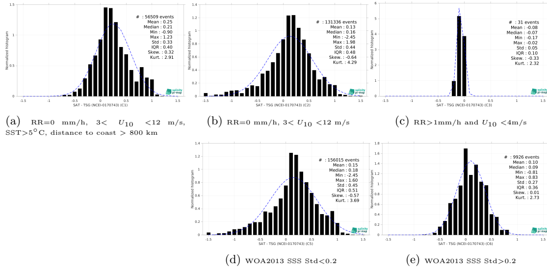
Figure 13: Normalized histogram of \Delta SSS (SMAP SSS L3 v5 - 8-Day running (RSS) - TSG (NCEI-0170743)) for 5 different subdatasets corresponding to: RR=0 mm/h, 3 < U_{10} < 12 m/s, SST>5°C, distance to coast > 800 km (a), RR=0 mm/h, 3 < U_{10} < 12 m/s (b), RR>1mm/h and U_{10} < 4 m/s (c), WOA2013 SSS Std<0.2 (d), WOA2013 SSS Std>0.2 (e).
