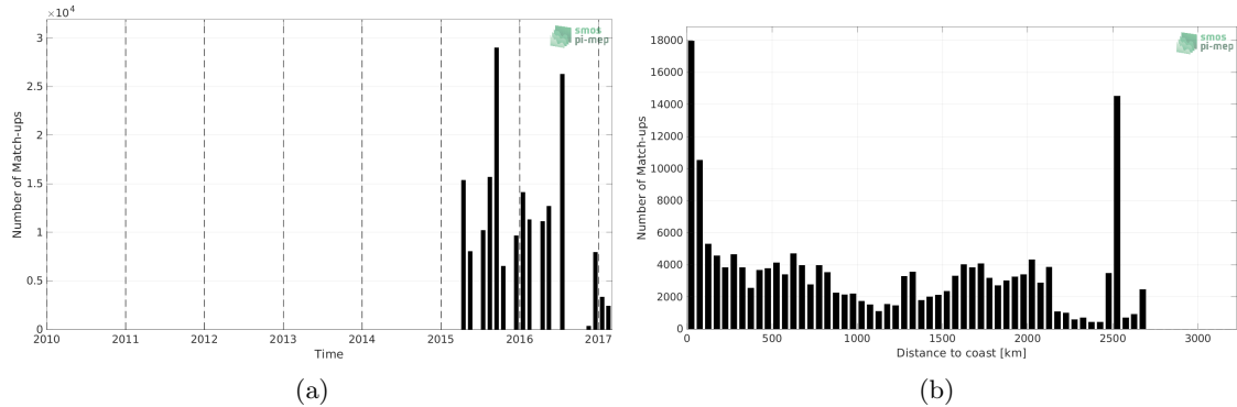
Figure 1: Number of match-ups between TSG (NCEI-0170743) and SMAP SSS L3 v5 - 8-Day running (RSS) SSS as a function of time (a) and as function of the distance to coast (b) over the Global Ocean Pi-MEP region and for the full satellite product period.
