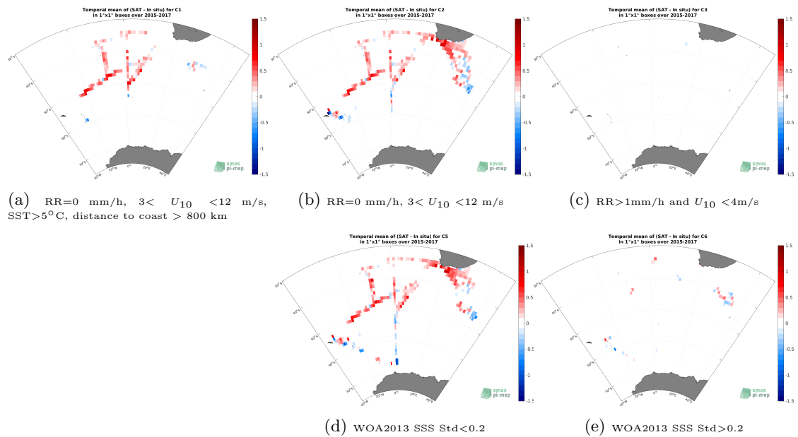
Figure 12: Temporal mean gridded over spatial boxes of size 1^\circ \times 1^\circ of \Delta SSS (SMAP SSS L3 v5 - 8-Day running (RSS) - TSG (NCEI-0170743)) for 5 different subdatasets corresponding to:RR=0 mm/h, 3 < U_{10} < 12 m/s, SST >5^\circ C, distance to coast > 800 km (a), RR=0 mm/h, 3 < U_{10} < 12 m/s (b), RR >1 mm/h and U_{10} < 4 m/s (c), WOA2013 SSS Std <0.2 (d), WOA2013 SSS Std >0.2 (e).
