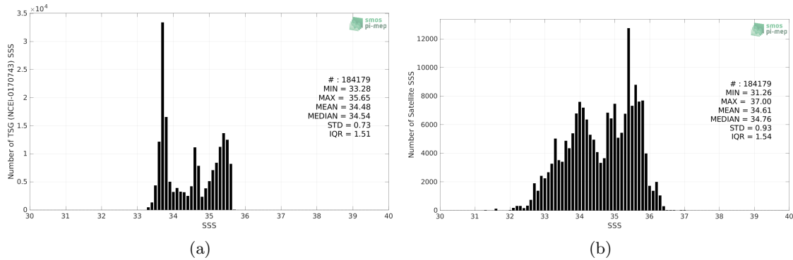
Figure 2: Histograms of SSS from TSG (NCEI-0170743) (a) and SMAP SSS L3 v5 - 8-Day running (RSS) (b) considering all match-up pairs per bins of 0.1 over the Global Ocean Pi-MEP region and for the full satellite product period.
