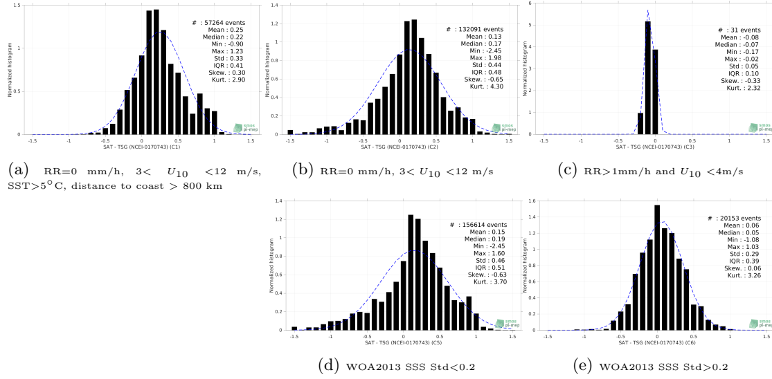
Figure 13: Normalized histogram of \Delta SSS (SMAP SSS L3 v5 - 8-Day running (RSS) - TSG (NCEI-0170743)) for 5 different subdatasets corresponding to: RR=0 mm/h, 3 < U_{10} < 12 m/s, SST > 5°C, distance to coast > 800 km (a), RR=0 mm/h, 3 < U_{10} < 12 m/s (b), RR > 1mm/h and U_{10} < 4 m/s (c), WOA2013 SSS Std < 0.2 (d), WOA2013 SSS Std > 0.2 (e).
