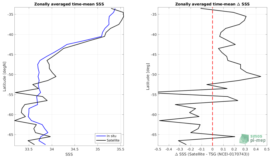
Figure 8: Left panel: Zonal mean SSS from SMAP SSS L3 v5 - 8-Day running (RSS) satellite product (black) and from TSG (NCEI-0170743) (blue). Right panel: Zonal mean of \Delta SSS (Satellite - TSG (NCEI-0170743)) for all the collected Pi-MEP match-up pairs estimated over the full satellite product period.
