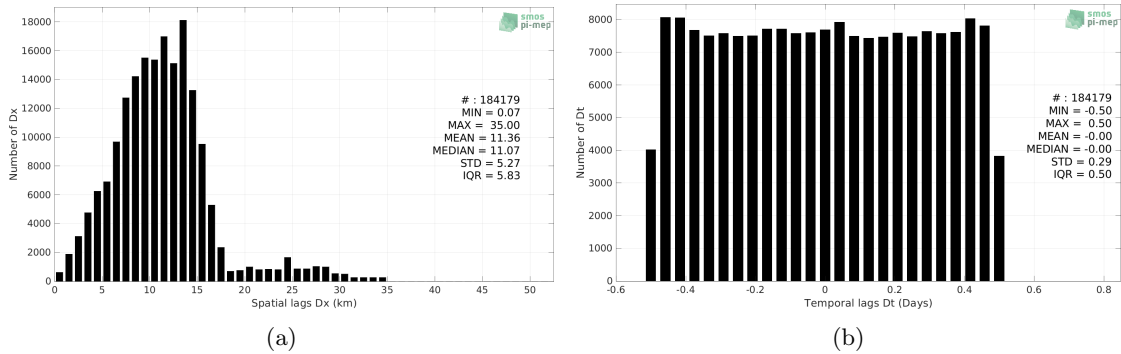
Figure 5: Histograms of the spatial (a) and temporal (b) lags between the location/time of the TSG (NCEI-0170743) measurement and the date of the corresponding SMAP SSS L3 v5 - 8-Day running (RSS) SSS pixel.
