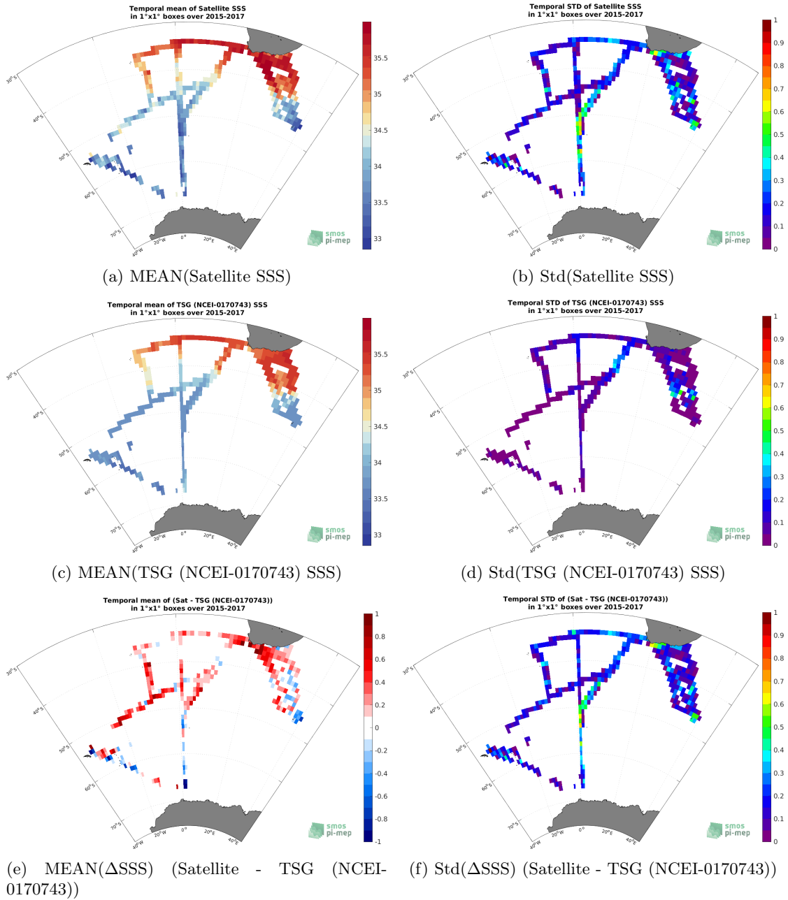
Figure 6: Temporal mean (left) and Std (right) of SSS from SMAP SSS L3 v5 - 8-Day running (RSS) (top), TSG (NCEI-0170743) (middle), and of \Delta SSS (Satellite - TSG (NCEI-0170743)). Only match-up pairs are used to generate these maps.
