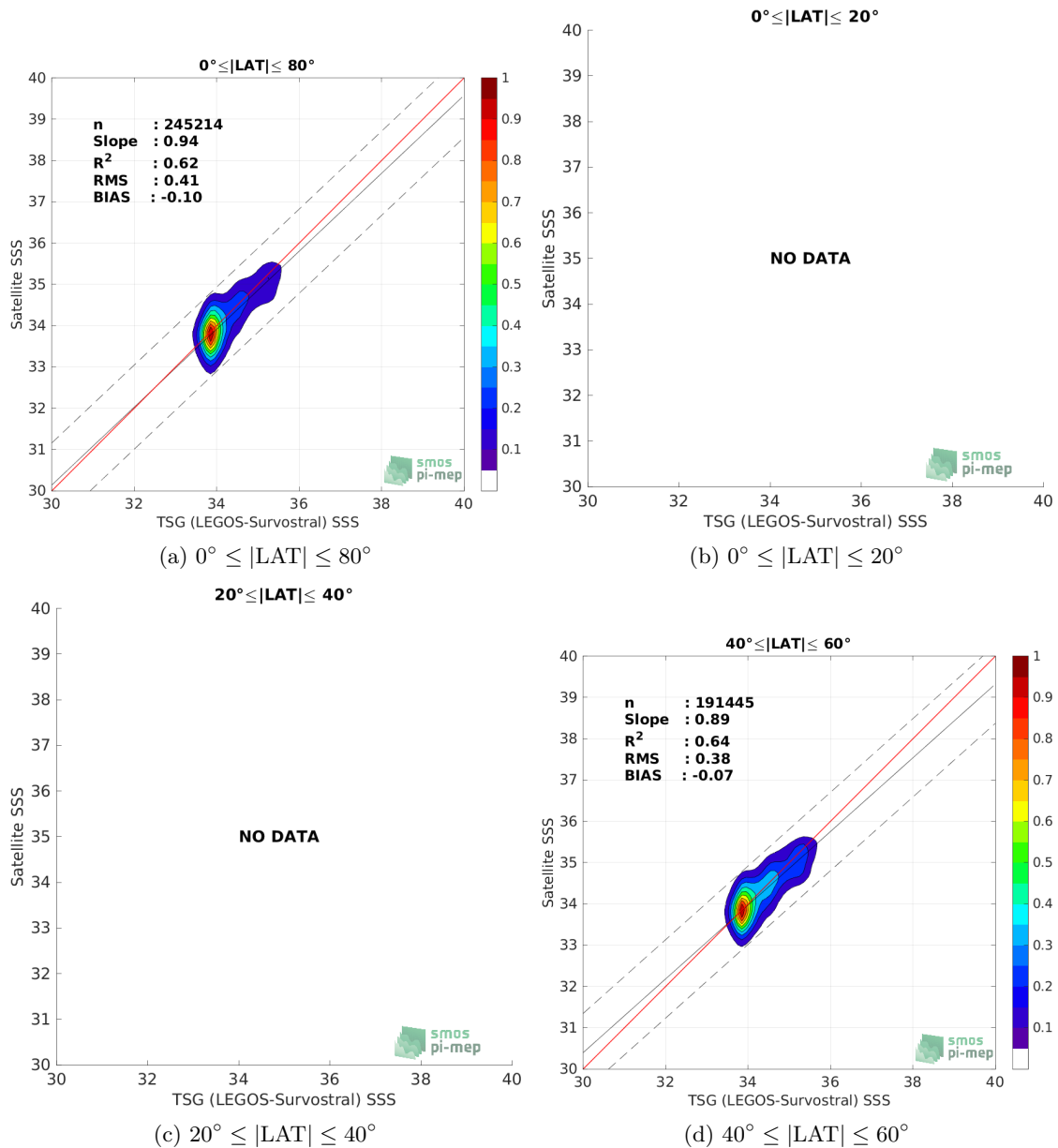
Figure 9: Contour maps of the concentration of SMAP SSS L3 v5 - 8-Day running (RSS) SSS (y-axis) versus TSG (LEGOS-Survostral) SSS (x-axis) at match-up pairs for different latitude bands. For each plot, the red line shows x=y . The black thin and dashed lines indicate a linear fit through the data cloud and the \pm 95\% confidence levels, respectively. The number match-up pairs n , the slope and R^2 coefficient of the linear fit, the root mean square (RMS) and the mean bias between satellite and in situ data are indicated for each latitude band in each plots.
