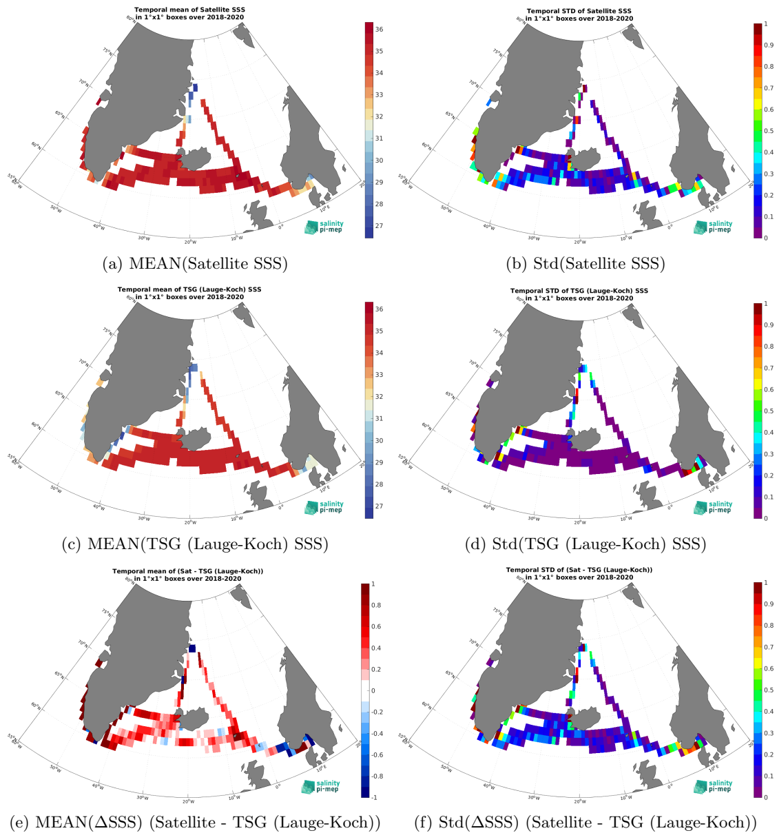
Figure 6: Temporal mean (left) and Std (right) of SSS from SMAP SSS L3 v5 - 8-Day running (RSS) (top), TSG (Lauge-Koch) (middle), and of \Delta SSS (Satellite - TSG (Lauge-Koch)). Only match-up pairs are used to generate these maps.
