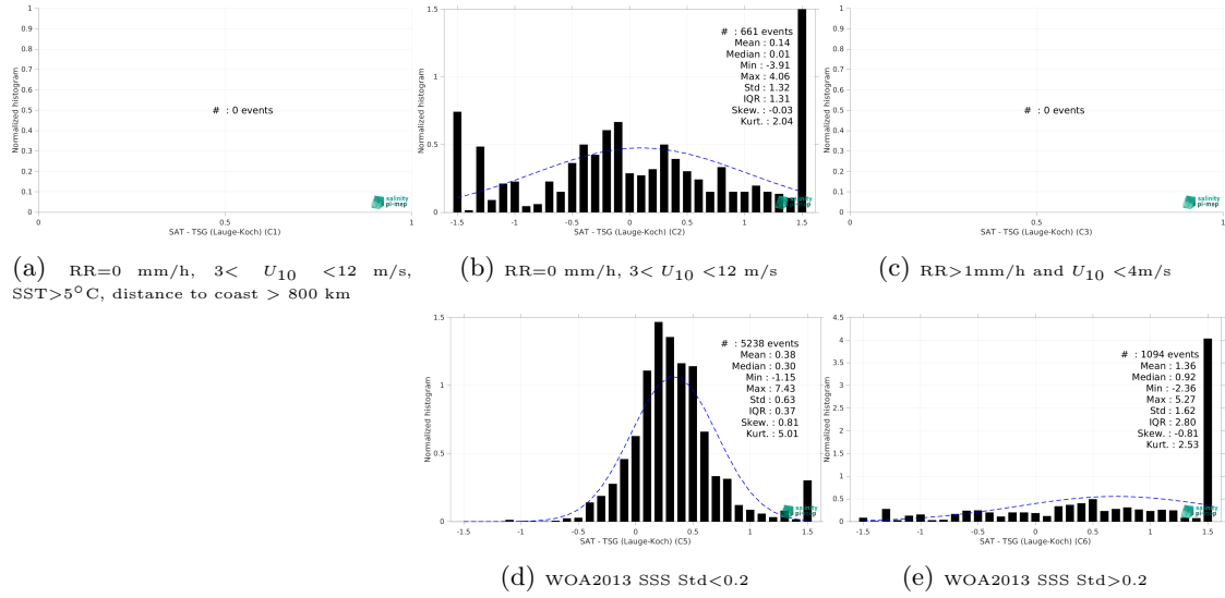
Figure 13: Normalized histogram of \Delta SSS (SMAP SSS L3 v5 - 8-Day running (RSS) - TSG (Lauge-Koch)) for 5 different subdatasets corresponding to: RR=0 mm/h, 3 < U_{10} < 12 m/s, SST > 5°C, distance to coast > 800 km (a), RR=0 mm/h, 3 < U_{10} < 12 m/s (b), RR > 1mm/h and U_{10} < 4 m/s (c), WOA2013 SSS Std < 0.2 (d), WOA2013 SSS Std > 0.2 (e).
