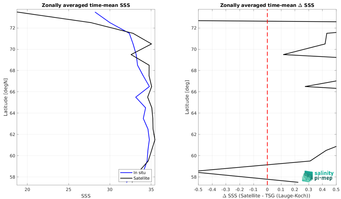
Figure 8: Left panel: Zonal mean SSS from SMAP SSS L3 v5 - 8-Day running (RSS) satellite product (black) and from TSG (Lauge-Koch) (blue). Right panel: Zonal mean of \Delta SSS (Satellite - TSG (Lauge-Koch)) for all the collected Pi-MEP match-up pairs estimated over the full satellite product period.
