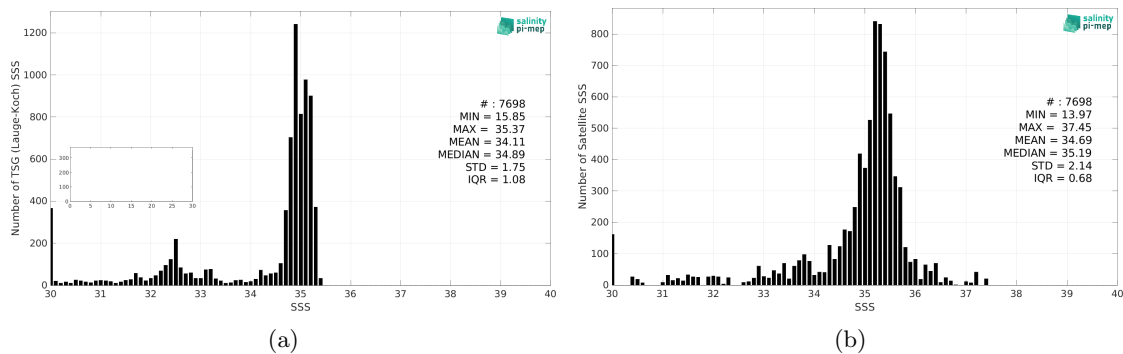
Figure 2: Histograms of SSS from TSG (Lauge-Koch) (a) and SMAP SSS L3 v5 - 8-Day running (RSS) (b) considering all match-up pairs per bins of 0.1 over the Global Ocean Pi-MEP region and for the full satellite product period.
