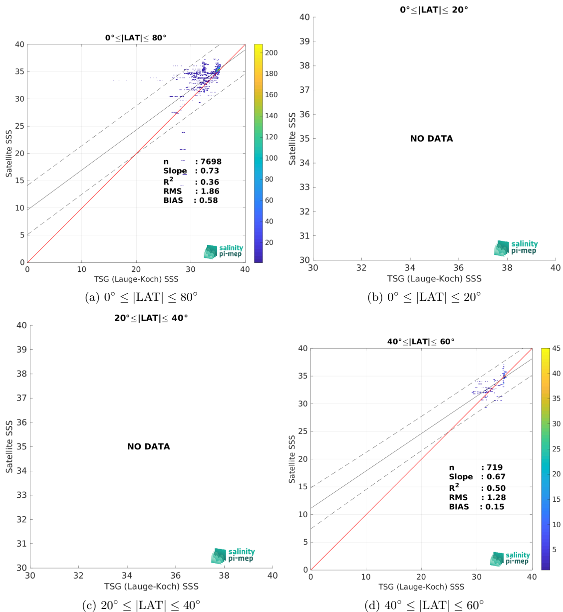
Figure 9: Contour maps of the concentration of SMAP SSS L3 v5 - 8-Day running (RSS) SSS (y-axis) versus TSG (Lauge-Koch) SSS (x-axis) at match-up pairs for different latitude bands. For each plot, the red line shows x=y . The black thin and dashed lines indicate a linear fit through the data cloud and the \pm 95\% confidence levels, respectively. The number match-up pairs n , the slope and R^2 coefficient of the linear fit, the root mean square (RMS) and the mean bias between satellite and in situ data are indicated for each latitude band in each plots.
