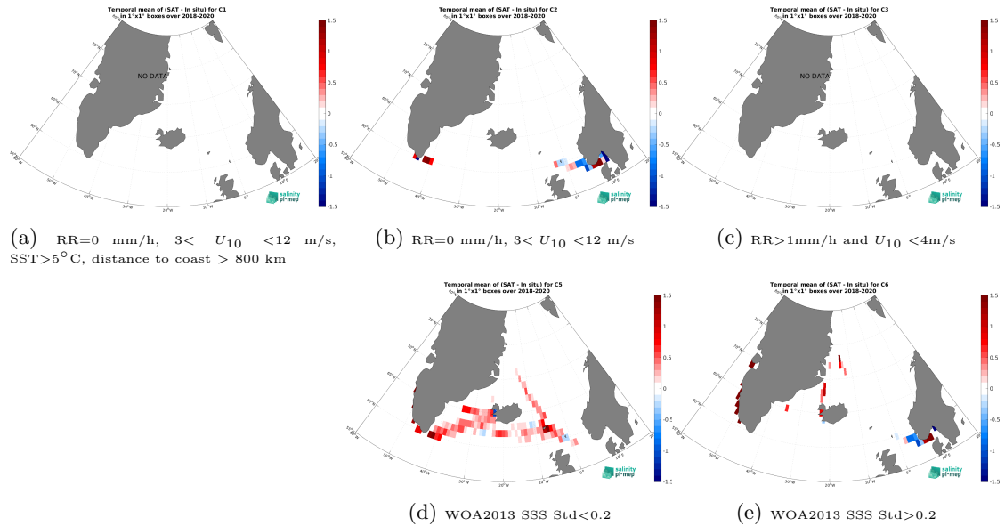
Figure 12: Temporal mean gridded over spatial boxes of size 1^{\circ}\times 1^{\circ} of \Delta\text{SSS} (SMAP SSS L3 v5 - 8-Day running (RSS) - TSG (Lauge-Koch)) for 5 different subdatasets corresponding to:RR=0 mm/h, 3 < U_{10} < 12 m/s, SST >5^{\circ}\text{C} , distance to coast > 800 km (a), RR=0 mm/h, 3 < U_{10} < 12 m/s (b), RR >1 mm/h and U_{10} < 4 m/s (c), WOA2013 SSS Std <0.2 (d), WOA2013 SSS Std >0.2 (e).
