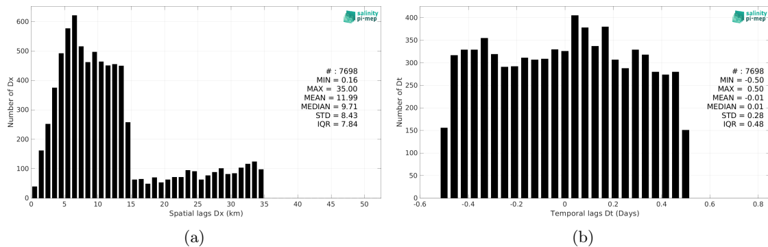
Figure 5: Histograms of the spatial (a) and temporal (b) lags between the location/time of the TSG (Lauge-Koch) measurement and the date of the corresponding SMAP SSS L3 v5 - 8-Day running (RSS) SSS pixel.
