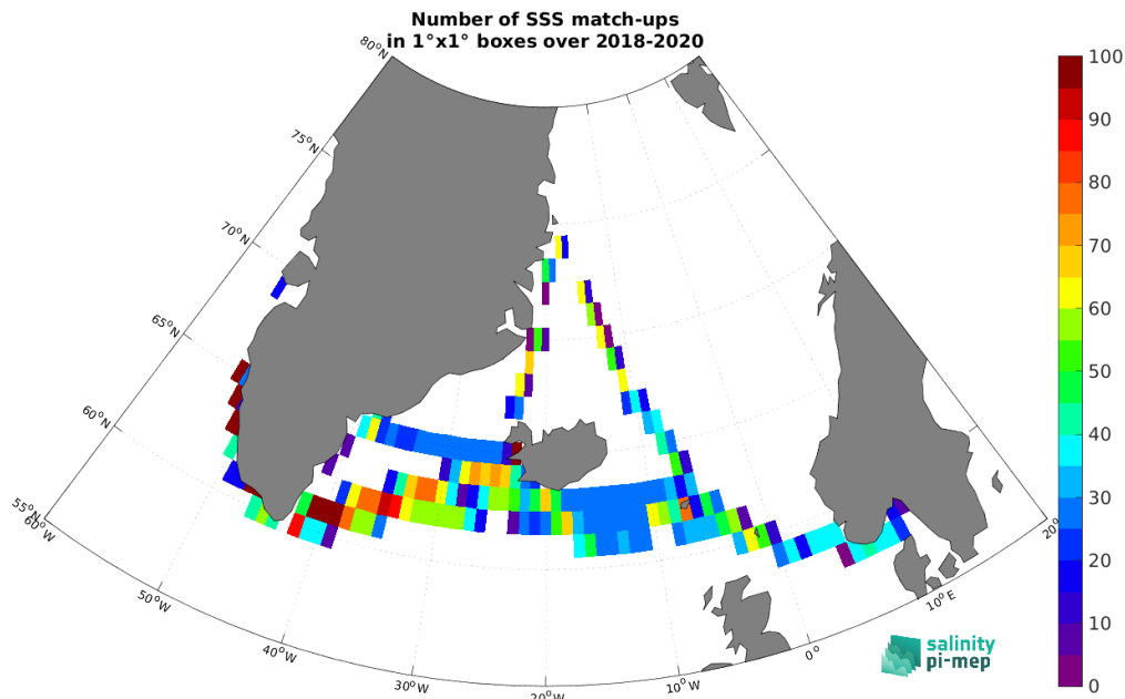
Figure 4: Number of SSS match-ups between TSG (Lauge-Koch) SSS and the SMAP SSS L3 v5 - 8-Day running (RSS) SSS product for the Global Ocean Pi-MEP region over 1^\circ \times 1^\circ boxes and for the full satellite product period.
