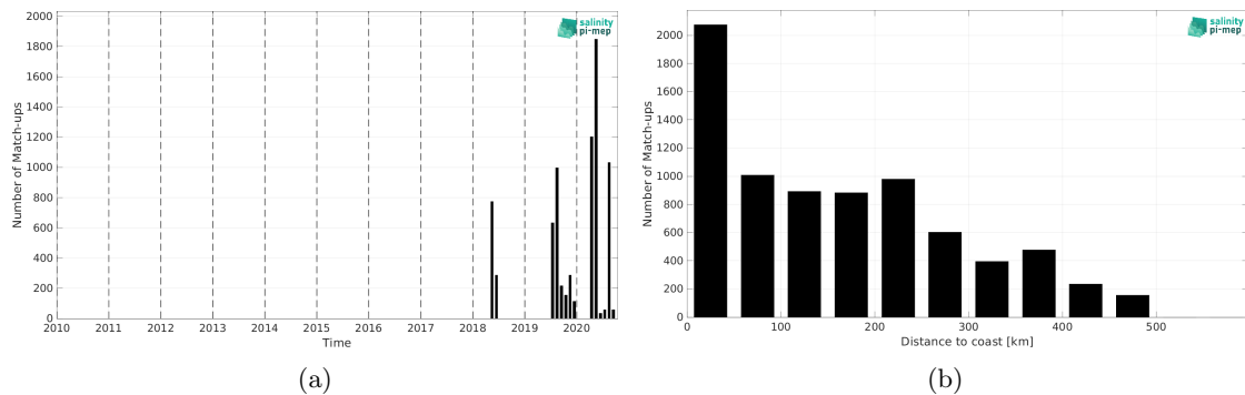
Figure 1: Number of match-ups between TSG (Lauge-Koch) and SMAP SSS L3 v5 - 8-Day running (RSS) SSS as a function of time (a) and as function of the distance to coast (b) over the Global Ocean Pi-MEP region and for the full satellite product period.
