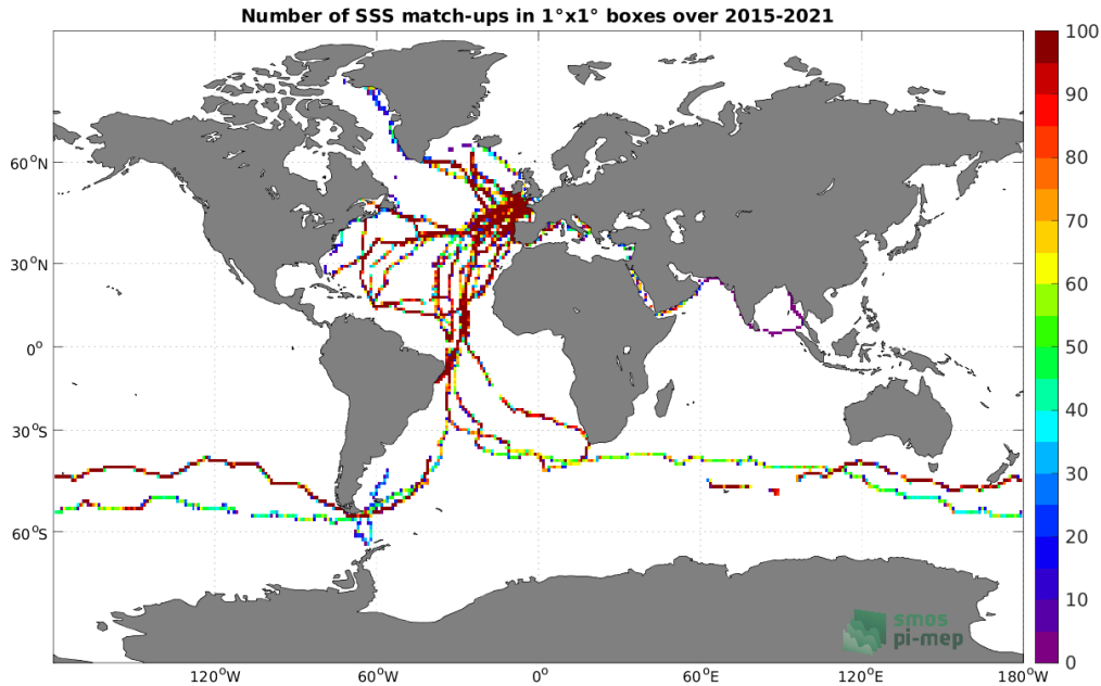
Figure 4: Number of SSS match-ups between TSG (GOSUD-Sailing-ship) SSS and the SMAP SSS L3 v5 - 8-Day running (RSS) SSS product for the Global Ocean Pi-MEP region over 1°x1° boxes and for the full satellite product period.
