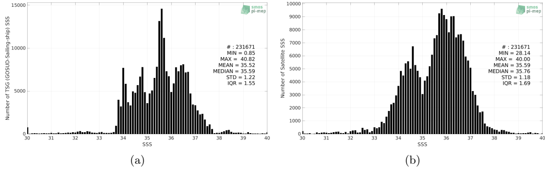
Figure 2: Histograms of SSS from TSG (GOSUD-Sailing-ship) (a) and SMAP SSS L3 v5 - 8-Day running (RSS) (b) considering all match-up pairs per bins of 0.1 over the Global Ocean Pi-MEP region and for the full satellite product period.
