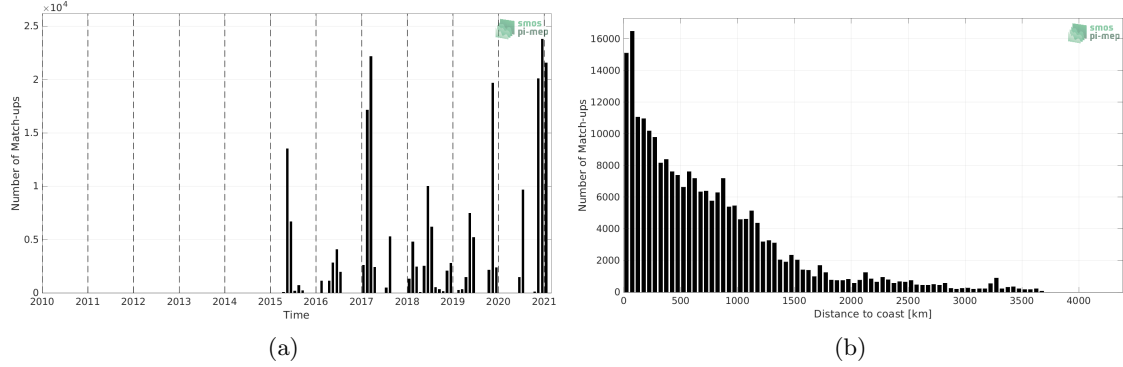
Figure 1: Number of match-ups between TSG (GOSUD-Sailing-ship) and SMAP SSS L3 v5 - 8-Day running (RSS) SSS as a function of time (a) and as function of the distance to coast (b) over the Global Ocean Pi-MEP region and for the full satellite product period.
