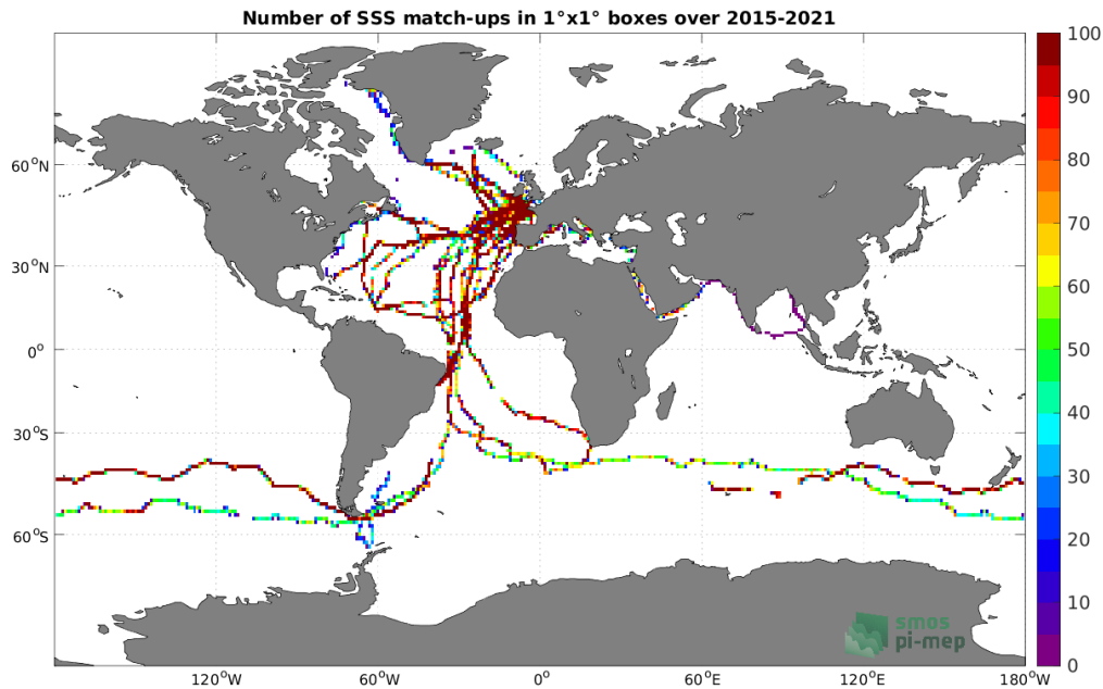
Figure 4: Number of SSS match-ups between TSG (GOSUD-Sailing-ship) SSS and the SMAP SSS L3 v5 - 8-Day running (RSS) SSS product for the Global Ocean Pi-MEP region over 1^\circ \times 1^\circ boxes and for the full satellite product period.
