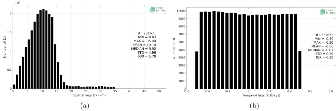
Figure 5: Histograms of the spatial (a) and temporal (b) lags between the location/time of the TSG (GOSUD-Sailing-ship) measurement and the date of the corresponding SMAP SSS L3 v5 - 8-Day running (RSS) SSS pixel.
