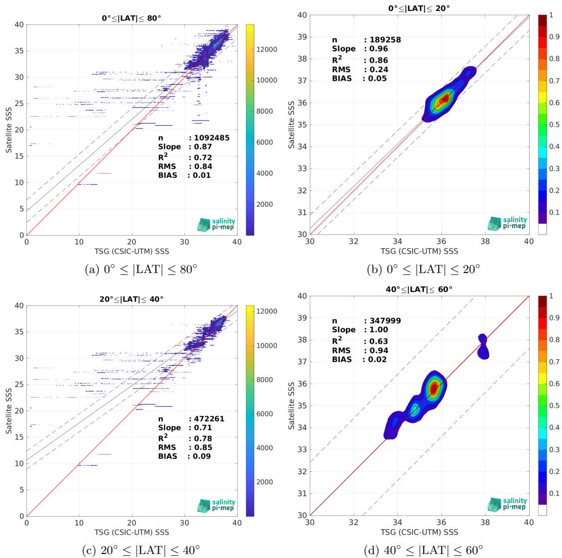
Figure 9: Contour maps of the concentration of SMAP SSS L3 v5 - 8-Day running (RSS) SSS (y-axis) versus TSG (CSIC-UTM) SSS (x-axis) at match-up pairs for different latitude bands. For each plot, the red line shows x=y . The black thin and dashed lines indicate a linear fit through the data cloud and the \pm 95\% confidence levels, respectively. The number match-up pairs n , the slope and R^2 coefficient of the linear fit, the root mean square (RMS) and the mean bias between satellite and in situ data are indicated for each latitude band in each plots.
