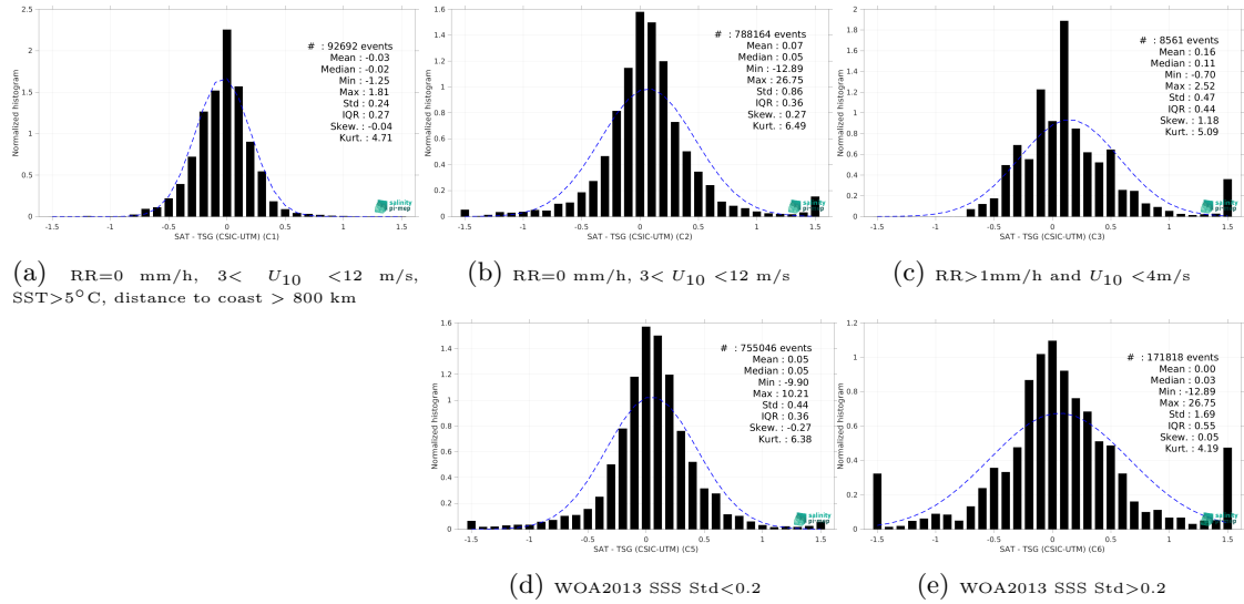
Figure 13: Normalized histogram of \Delta\text{SSS} (SMAP SSS L3 v5 - 8-Day running (RSS) - TSG (CSIC-UTM)) for 5 different subdatasets corresponding to: RR=0 mm/h, 3 < U_{10} < 12 m/s, SST > 5^\circ\text{C} , distance to coast > 800 km (a), RR=0 mm/h, 3 < U_{10} < 12 m/s (b), RR > 1 mm/h and U_{10} < 4 m/s (c), WOA2013 SSS Std < 0.2 (d), WOA2013 SSS Std > 0.2 (e).
