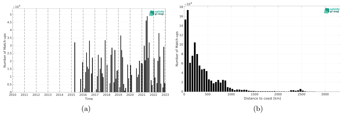
Figure 1: Number of match-ups between TSG (CSIC-UTM) and SMAP SSS L3 v5 - 8-Day running (RSS) SSS as a function of time (a) and as function of the distance to coast (b) over the Global Ocean Pi-MEP region and for the full satellite product period.
