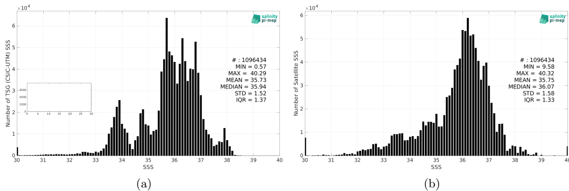
Figure 2: Histograms of SSS from TSG (CSIC-UTM) (a) and SMAP SSS L3 v5 - 8-Day running (RSS) (b) considering all match-up pairs per bins of 0.1 over the Global Ocean Pi-MEP region and for the full satellite product period.
