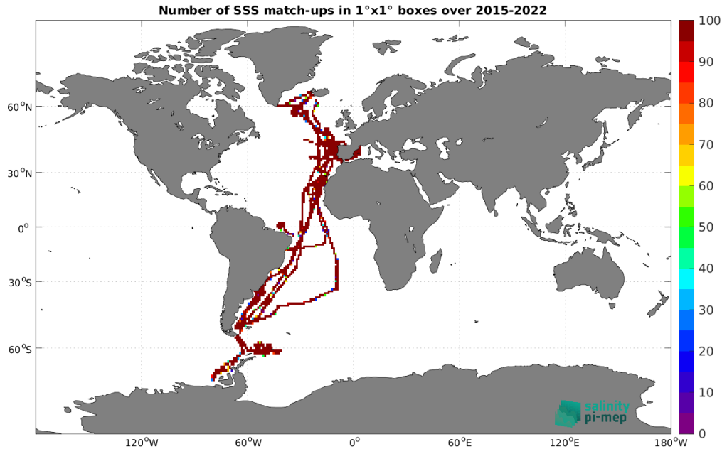
Figure 4: Number of SSS match-ups between TSG (CSIC-UTM) SSS and the SMAP SSS L3 v5 - 8-Day running (RSS) SSS product for the Global Ocean Pi-MEP region over 1°×1° boxes and for the full satellite product period.
