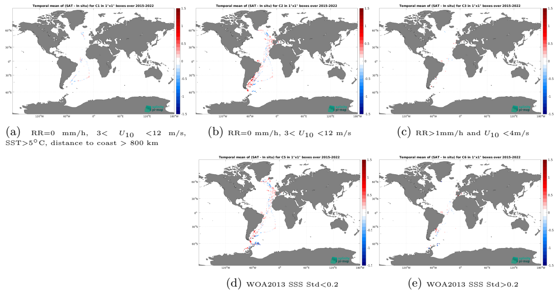
Figure 12: Temporal mean gridded over spatial boxes of size 1^\circ \times 1^\circ of \Delta SSS (SMAP SSS L3 v5 - 8-Day running (RSS) - TSG (CSIC-UTM)) for 5 different subdatasets corresponding to:RR=0 mm/h, 3 < U_{10} < 12 m/s, SST >5^\circ\text{C} , distance to coast > 800 km (a), RR=0 mm/h, 3 < U_{10} < 12 m/s (b), RR >1 mm/h and U_{10} < 4 m/s (c), WOA2013 SSS Std <0.2 (d), WOA2013 SSS Std >0.2 (e).
