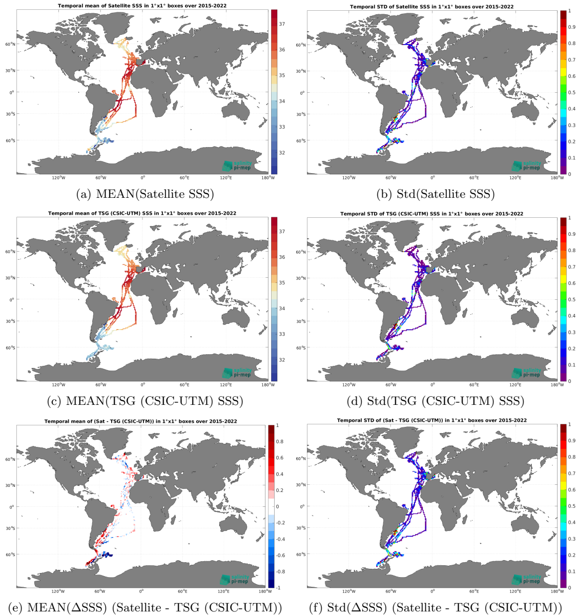
Figure 6: Temporal mean (left) and Std (right) of SSS from SMAP SSS L3 v5 - 8-Day running (RSS) (top), TSG (CSIC-UTM) (middle), and of \Delta SSS (Satellite - TSG (CSIC-UTM)). Only match-up pairs are used to generate these maps.
