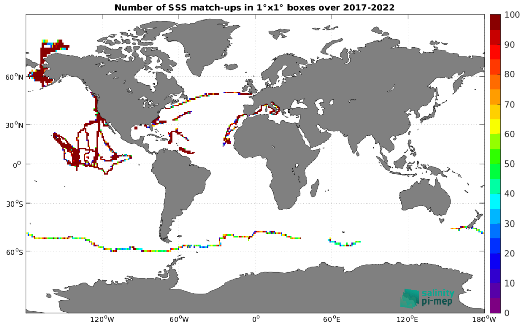
Figure 4: Number of SSS match-ups between Saildrone SSS and the SMAP SSS L3 v5 - 8-Day running (RSS) SSS product for the Global Ocean Pi-MEP region over 1^\circ \times 1^\circ boxes and for the full satellite product period.
