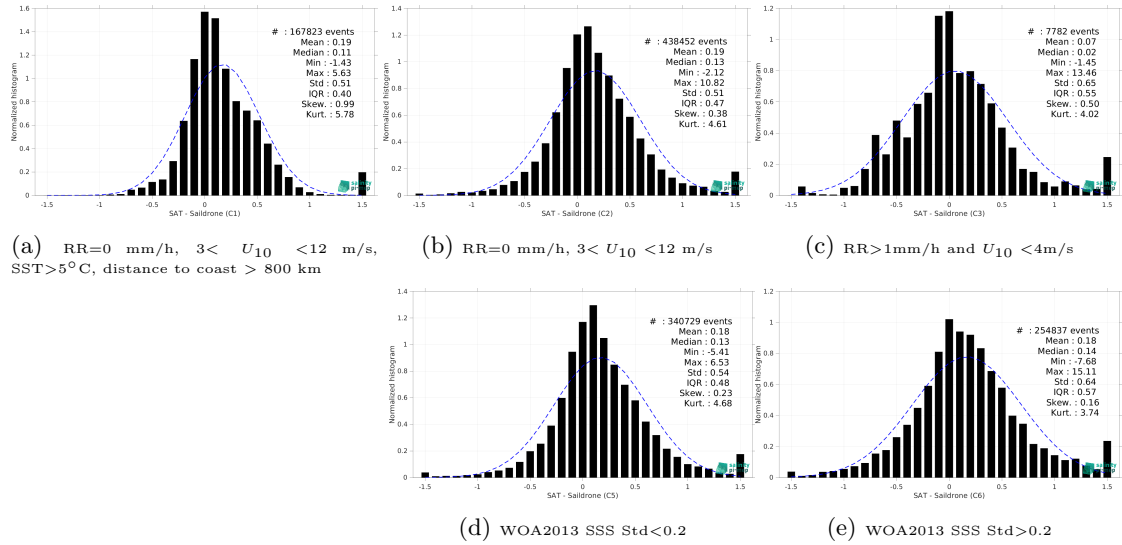
Figure 13: Normalized histogram of \Delta\text{SSS} (SMAP SSS L3 v5 - 8-Day running (RSS) - Saldrone) for 5 different subdatasets corresponding to: RR=0 mm/h, 3 < U_{10} < 12 m/s, SST > 5^\circ\text{C} , distance to coast > 800 km (a), RR=0 mm/h, 3 < U_{10} < 12 m/s (b), RR > 1 mm/h and U_{10} < 4 m/s (c), WOA2013 SSS Std < 0.2 (d), WOA2013 SSS Std > 0.2 (e).
