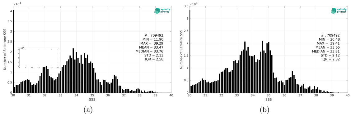
Figure 2: Histograms of SSS from Saildrone (a) and SMAP SSS L3 v5 - 8-Day running (RSS) (b) considering all match-up pairs per bins of 0.1 over the Global Ocean Pi-MEP region and for the full satellite product period.
