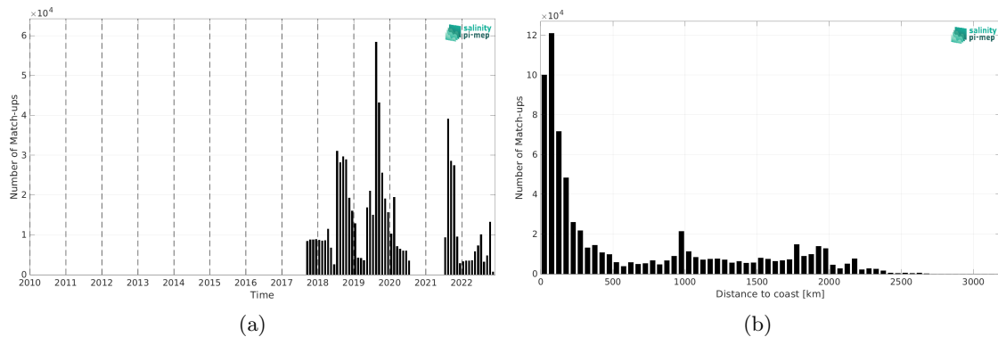
Figure 1: Number of match-ups between Saildrone and SMAP SSS L3 v5 - 8-Day running (RSS) SSS as a function of time (a) and as function of the distance to coast (b) over the Global Ocean Pi-MEP region and for the full satellite product period.
