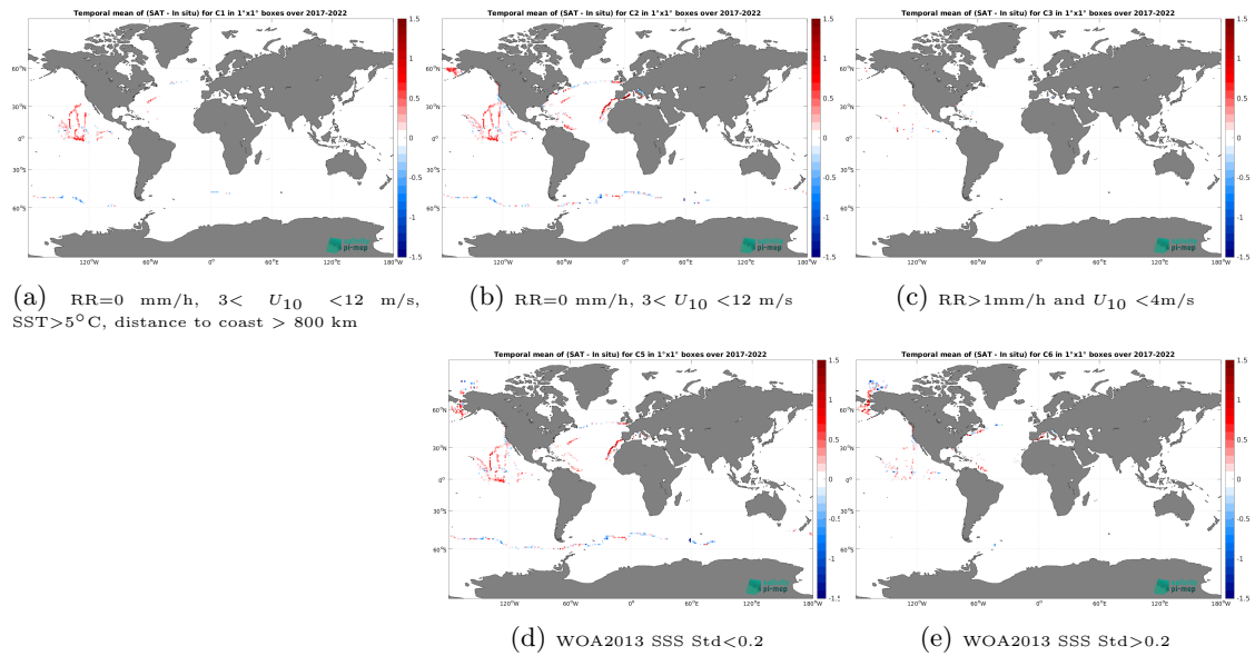
Figure 12: Temporal mean gridded over spatial boxes of size 1^\circ \times 1^\circ of \Delta SSS (SMAP SSS L3 v5 - 8-Day running (RSS) - Sairdrone) for 5 different subdatasets corresponding to:RR=0 mm/h, 3 < U_{10} < 12 m/s, SST > 5^\circ\text{C} , distance to coast > 800 km (a), RR=0 mm/h, 3 < U_{10} < 12 m/s (b), RR > 1 mm/h and U_{10} < 4 m/s (c), WOA2013 SSS Std < 0.2 (d), WOA2013 SSS Std > 0.2 (e).
