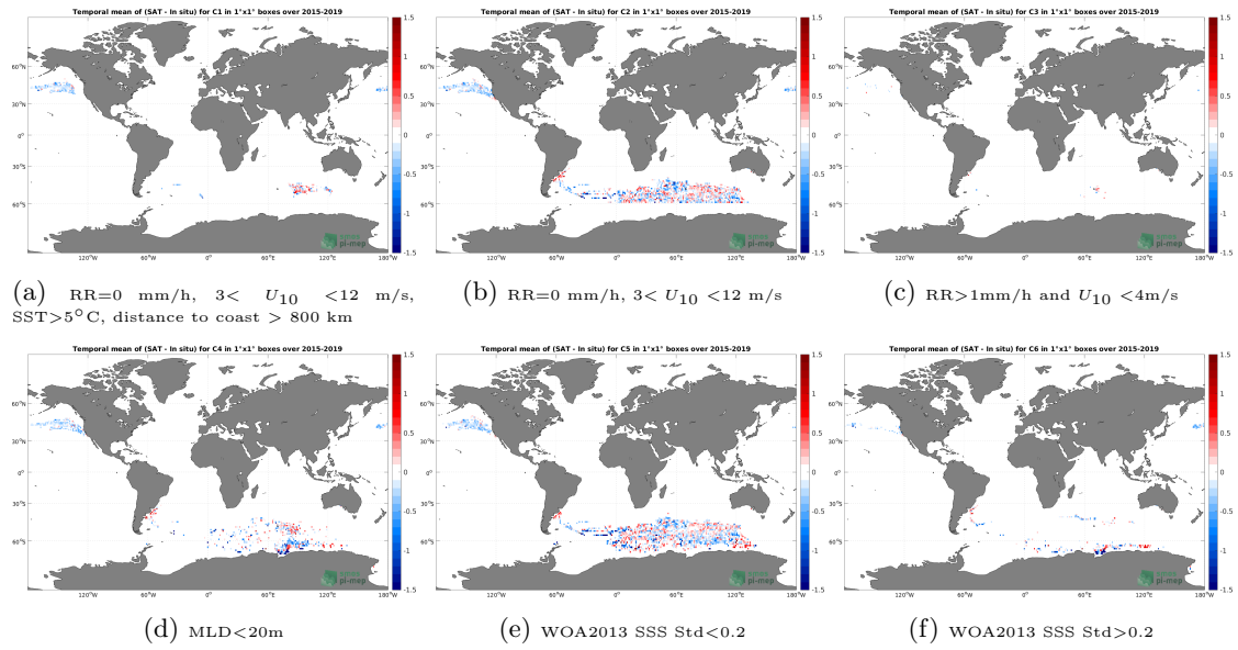
Figure 12: Temporal mean gridded over spatial boxes of size 1^\circ \times 1^\circ of \Delta SSS (SMAP SSS L3 v5 - 8-Day running (RSS) - Marine mammals) for 6 different subdatasets corresponding to:RR=0 mm/h, 3 < U_{10} < 12 m/s, SST > 5^\circ\text{C} , distance to coast > 800 km (a), RR=0 mm/h, 3 < U_{10} < 12 m/s (b), RR > 1 mm/h and U_{10} < 4 m/s (c),MLD < 20 m (d),WOA2013 SSS Std < 0.2 (e),WOA2013 SSS Std > 0.2 (f).
