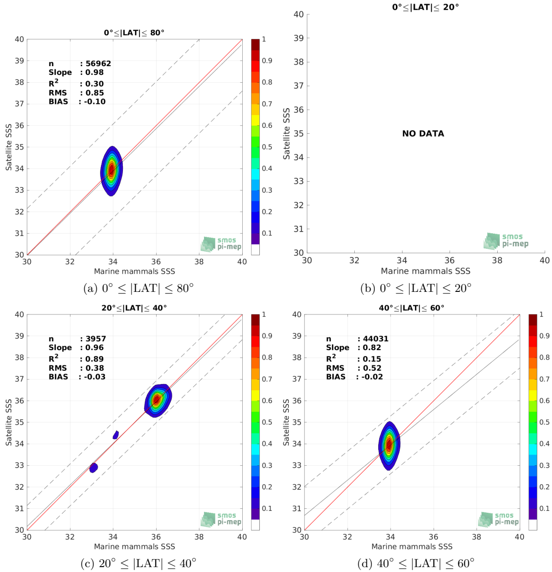
Figure 9: Contour maps of the concentration of SMAP SSS L3 v5 - 8-Day running (RSS) SSS (y-axis) versus Marine mammals SSS (x-axis) at match-up pairs for different latitude bands. For each plot, the red line shows x=y . The black thin and dashed lines indicate a linear fit through the data cloud and the \pm 95\% confidence levels, respectively. The number match-up pairs n , the slope and R^2 coefficient of the linear fit, the root mean square (RMS) and the mean bias between satellite and in situ data are indicated for each latitude band in each plots.
