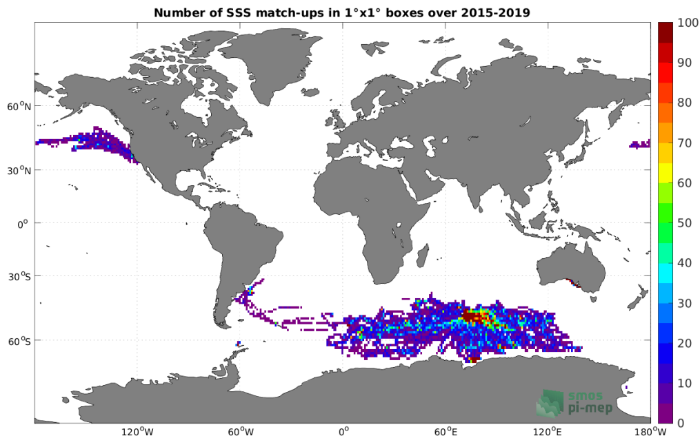
Figure 4: Number of SSS match-ups between Marine mammals SSS and the SMAP SSS L3 v5 - 8-Day running (RSS) SSS product for the Global Ocean Pi-MEP region over 1^\circ \times 1^\circ boxes and for the full satellite product period.
