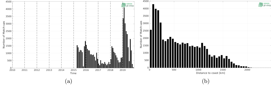
Figure 1: Number of match-ups between Marine mammals and SMAP SSS L3 v5 - 8-Day running (RSS) SSS as a function of time (a) and as function of the distance to coast (b) over the Global Ocean Pi-MEP region and for the full satellite product period.
