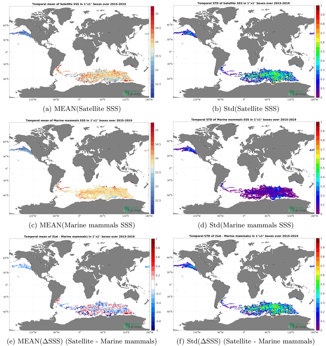
Figure 6: Temporal mean (left) and Std (right) of SSS from SMAP SSS L3 v5 - 8-Day running (RSS) (top), Marine mammals (middle), and of \Delta SSS (Satellite - Marine mammals). Only match-up pairs are used to generate these maps.
