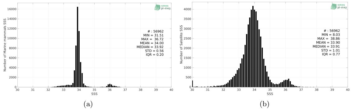
Figure 2: Histograms of SSS from Marine mammals (a) and SMAP SSS L3 v5 - 8-Day running (RSS) (b) considering all match-up pairs per bins of 0.1 over the Global Ocean Pi-MEP region and for the full satellite product period.
