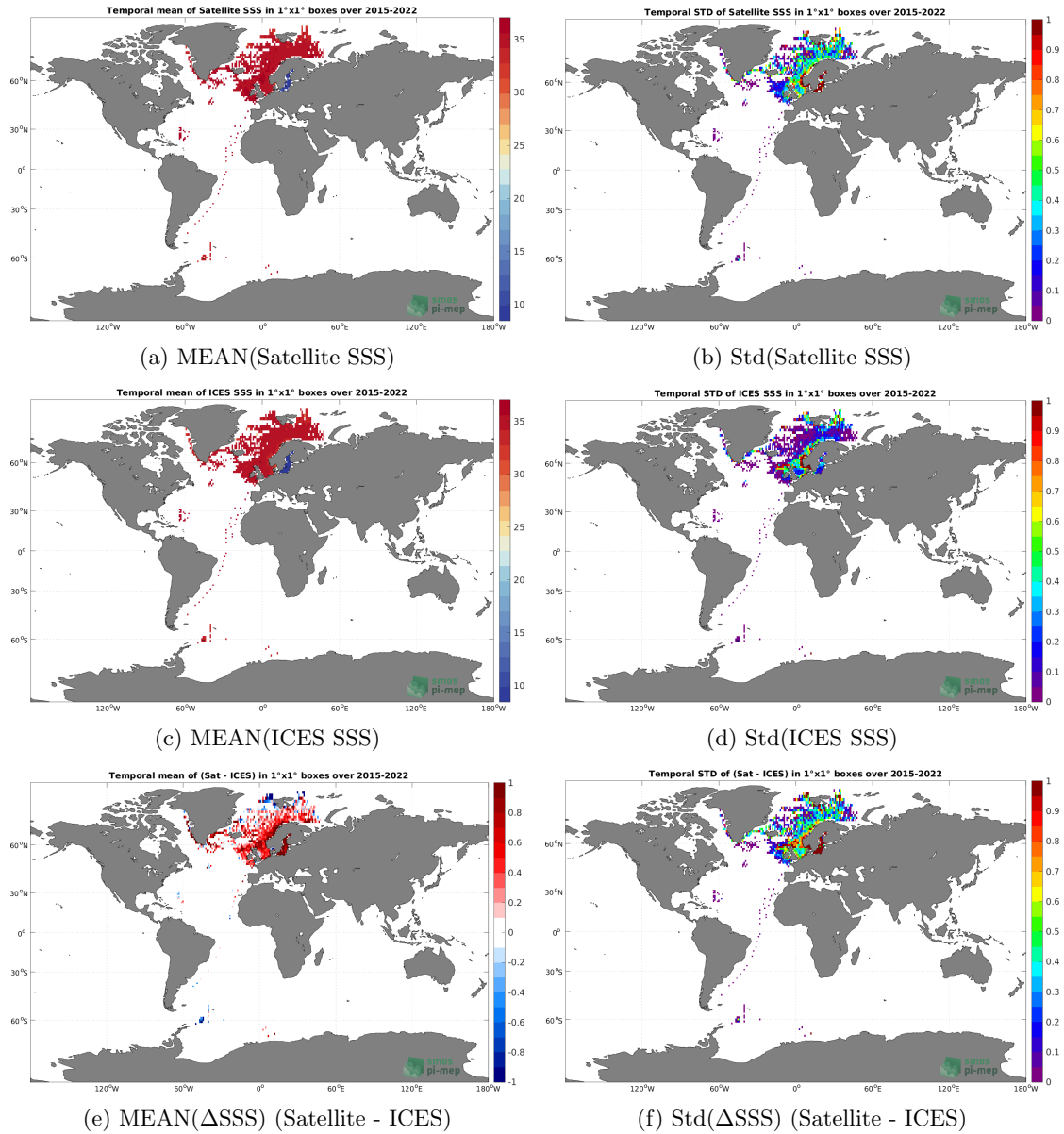
Figure 6: Temporal mean (left) and Std (right) of SSS from SMAP SSS L3 v5 - 8-Day running (RSS) (top), ICES (middle), and of \Delta SSS (Satellite - ICES). Only match-up pairs are used to generate these maps.
