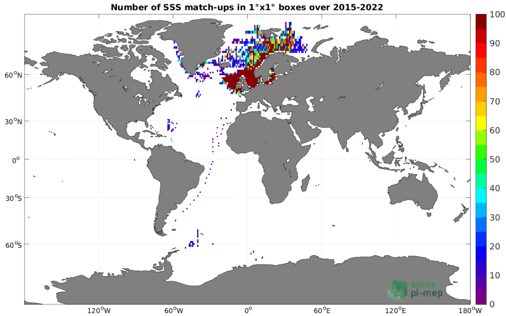
Figure 4: Number of SSS match-ups between ICES SSS and the SMAP SSS L3 v5 - 8-Day running (RSS) SSS product for the Global Ocean Pi-MEP region over 1^\circ \times 1^\circ boxes and for the full satellite product period.
