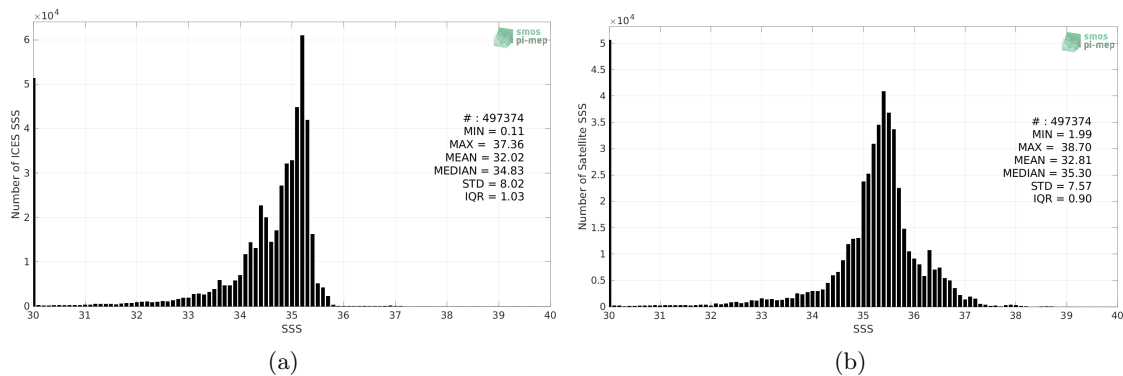
Figure 2: Histograms of SSS from ICES (a) and SMAP SSS L3 v5 - 8-Day running (RSS) (b) considering all match-up pairs per bins of 0.1 over the Global Ocean Pi-MEP region and for the full satellite product period.
