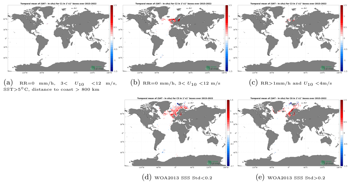
Figure 12: Temporal mean gridded over spatial boxes of size 1^\circ \times 1^\circ of \Delta SSS (SMAP SSS L3 v5 - 8-Day running (RSS) - ICES) for 5 different subdatasets corresponding to:RR=0 mm/h, 3 < U_{10} < 12 m/s, SST > 5^\circ\text{C} , distance to coast > 800 km (a), RR=0 mm/h, 3 < U_{10} < 12 m/s (b), RR > 1 mm/h and U_{10} < 4 m/s (c), WOA2013 SSS Std < 0.2 (d), WOA2013 SSS Std > 0.2 (e).
