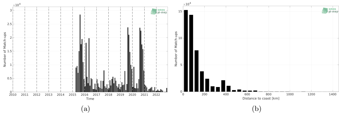
Figure 1: Number of match-ups between ICES and SMAP SSS L3 v5 - 8-Day running (RSS) SSS as a function of time (a) and as function of the distance to coast (b) over the Global Ocean Pi-MEP region and for the full satellite product period.
