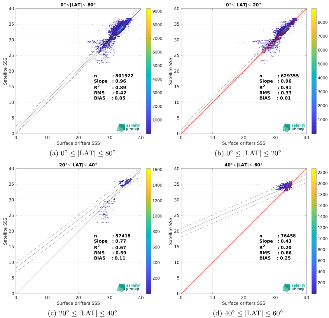
Figure 8: Contour maps of the concentration of SMAP SSS L3 v5 - 8-Day running (RSS) SSS (y-axis) versus Surface drifters SSS (x-axis) at match-up pairs for different latitude bands. For each plot, the red line shows x=y . The black thin and dashed lines indicate a linear fit through the data cloud and the \pm 95\% confidence levels, respectively. The number match-up pairs n , the slope and R^2 coefficient of the linear fit, the root mean square (RMS) and the mean bias between satellite and in situ data are indicated for each latitude band in each plots.
