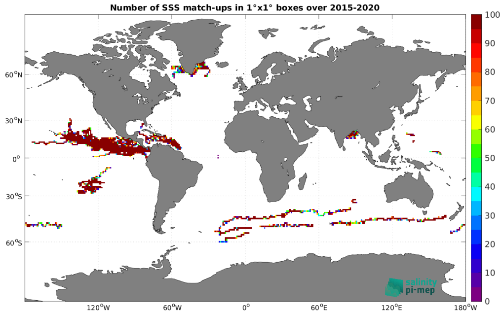
Figure 3: Number of SSS match-ups between Surface drifters SSS and the SMAP SSS L3 v5 - 8-Day running (RSS) SSS product for the Global Ocean Pi-MEP region over 1^\circ \times 1^\circ boxes and for the full satellite product period.
