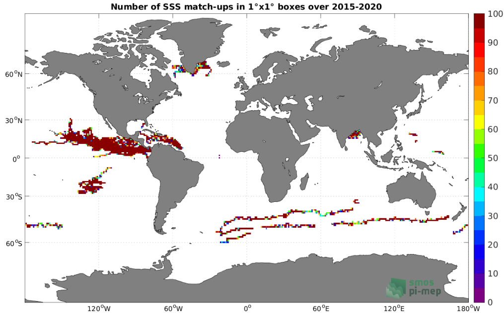
Figure 3: Number of SSS match-ups between Surface drifters SSS and the SMAP SSS L3 v5 - 8-Day running (RSS) SSS product for the Global Ocean Pi-MEP region over 1^\circ \times 1^\circ boxes and for the full satellite product period.
