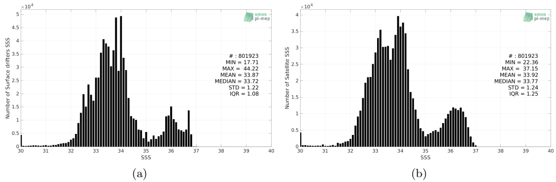
Figure 2: Histograms of SSS from Surface drifters (a) and SMAP SSS L3 v5 - 8-Day running (RSS) (b) considering all match-up pairs per bins of 0.1 over the Global Ocean Pi-MEP region and for the full satellite product period.
