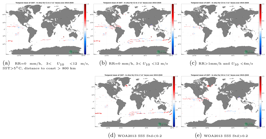
Figure 11: Temporal mean gridded over spatial boxes of size 1^\circ \times 1^\circ of \Delta SSS (SMAP SSS L3 v5 - 8-Day running (RSS) - Surface drifters) for 5 different subdatasets corresponding to:RR=0 mm/h, 3 < U_{10} < 12 m/s, SST > 5^\circ\text{C} , distance to coast > 800 km (a), RR=0 mm/h, 3 < U_{10} < 12 m/s (b), RR > 1 mm/h and U_{10} < 4 m/s (c), WOA2013 SSS Std < 0.2 (d), WOA2013 SSS Std > 0.2 (e).
