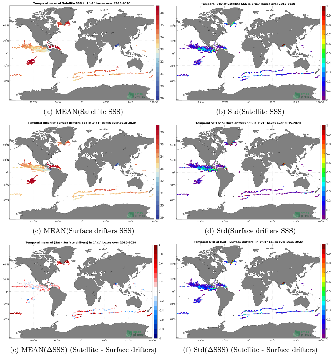
Figure 5: Temporal mean (left) and Std (right) of SSS from SMAP SSS L3 v5 - 8-Day running (RSS) (top), Surface drifters (middle), and of \Delta SSS (Satellite - Surface drifters). Only match-up pairs are used to generate these maps.
