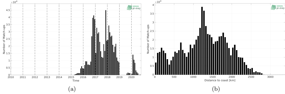
Figure 1: Number of match-ups between Surface drifters and SMAP SSS L3 v5 - 8-Day running (RSS) SSS as a function of time (a) and as function of the distance to coast (b) over the Global Ocean Pi-MEP region and for the full satellite product period.
