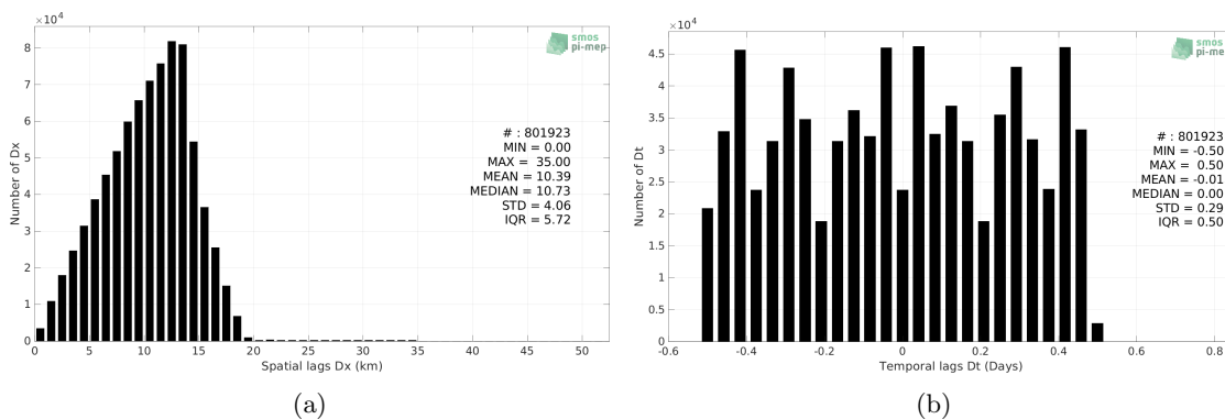
Figure 4: Histograms of the spatial (a) and temporal (b) lags between the location/time of the Surface drifters measurement and the date of the corresponding SMAP SSS L3 v5 - 8-Day running (RSS) SSS pixel.
