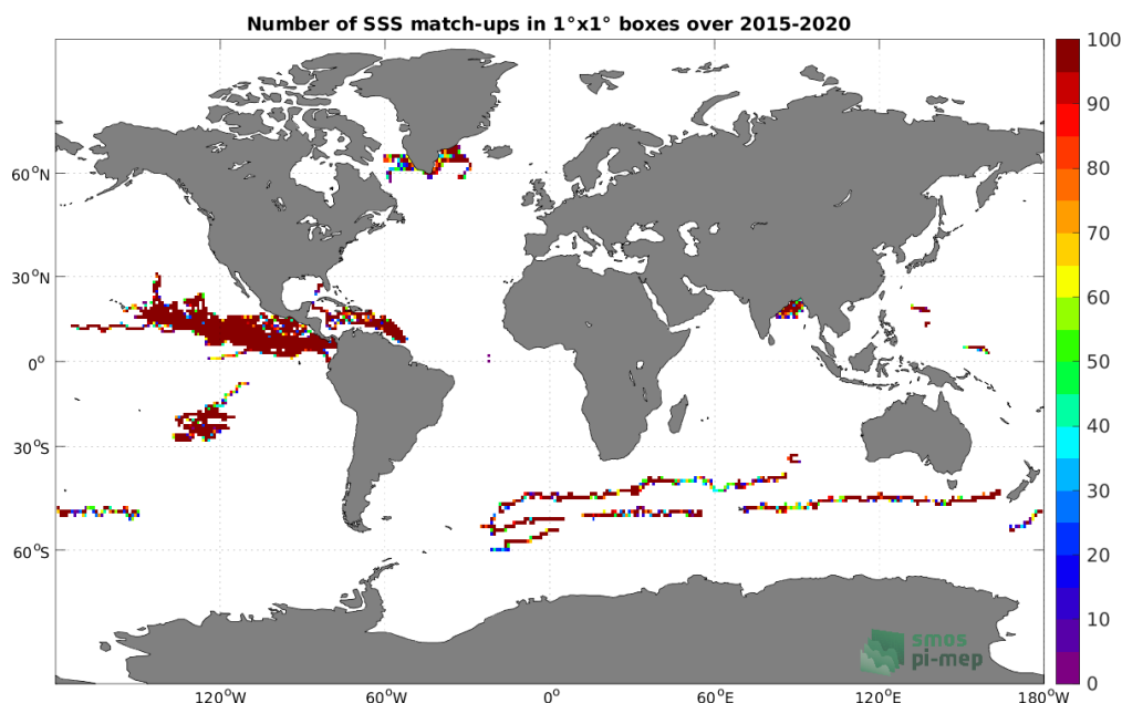
Figure 3: Number of SSS match-ups between Surface drifters SSS and the SMAP SSS L3 v5 - 8-Day running (RSS) SSS product for the Global Ocean Pi-MEP region over 1°x1° boxes and for the full satellite product period.
