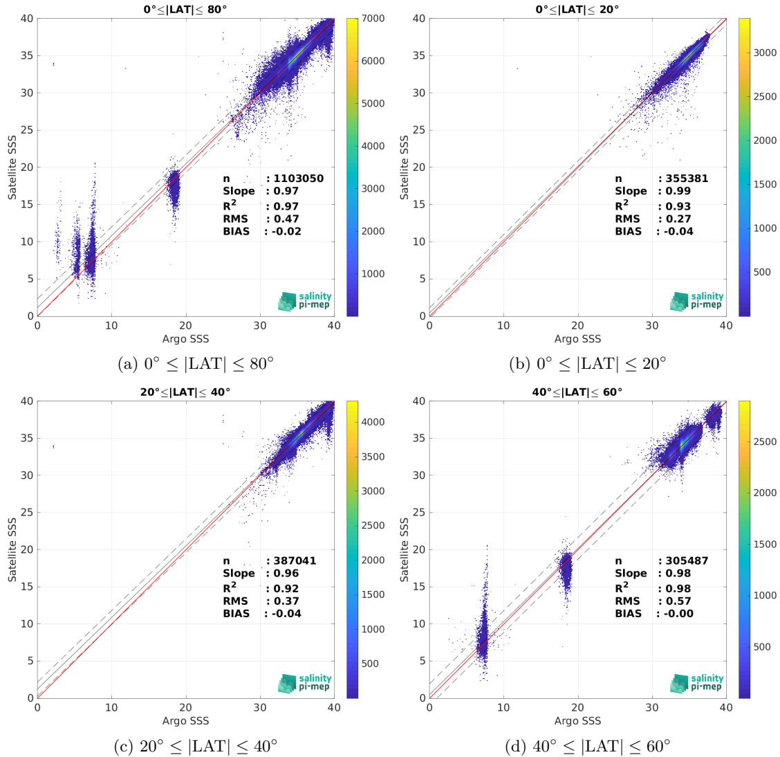
Figure 9: Contour maps of the concentration of SMAP SSS L3 v5 - 8-Day running (RSS) SSS (y-axis) versus Argo SSS (x-axis) at match-up pairs for different latitude bands. For each plot, the red line shows x=y . The black thin and dashed lines indicate a linear fit through the data cloud and the \pm 95\% confidence levels, respectively. The number match-up pairs n , the slope and R^2 coefficient of the linear fit, the root mean square (RMS) and the mean bias between satellite and in situ data are indicated for each latitude band in each plot.
