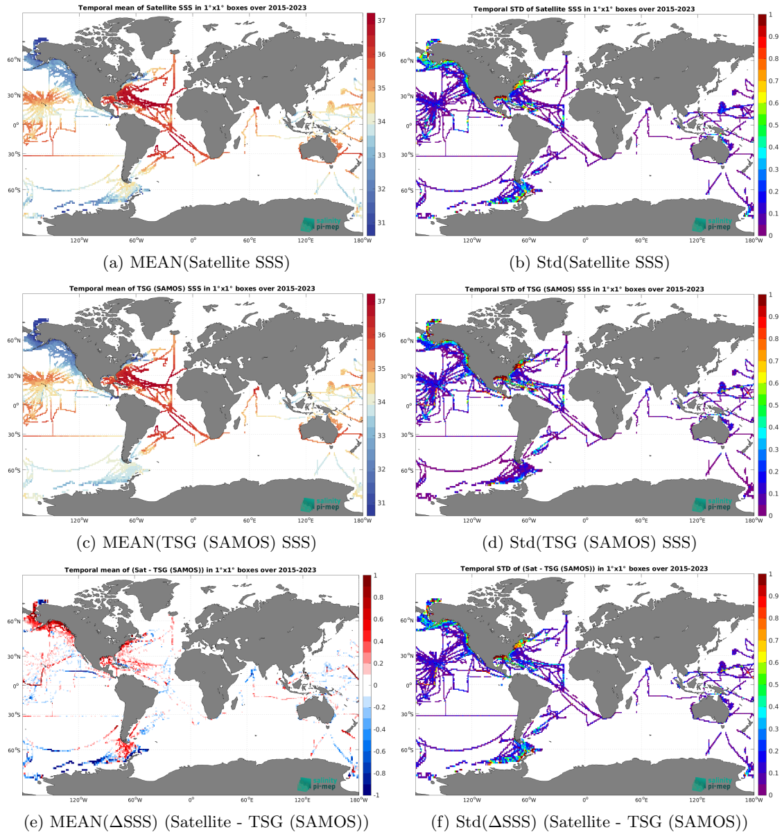
Figure 6: Temporal mean (left) and Std (right) of SSS from SMAP SSS L3 v5 - Monthly (RSS) (top), TSG (SAMOS) (middle), and of \Delta SSS (Satellite - TSG (SAMOS)). Only match-up pairs are used to generate these maps.
