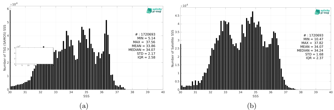
Figure 2: Histograms of SSS from TSG (SAMOS) (a) and SMAP SSS L3 v5 - Monthly (RSS) (b) considering all match-up pairs per bins of 0.1 over the Global Ocean Pi-MEP region and for the full satellite product period.
