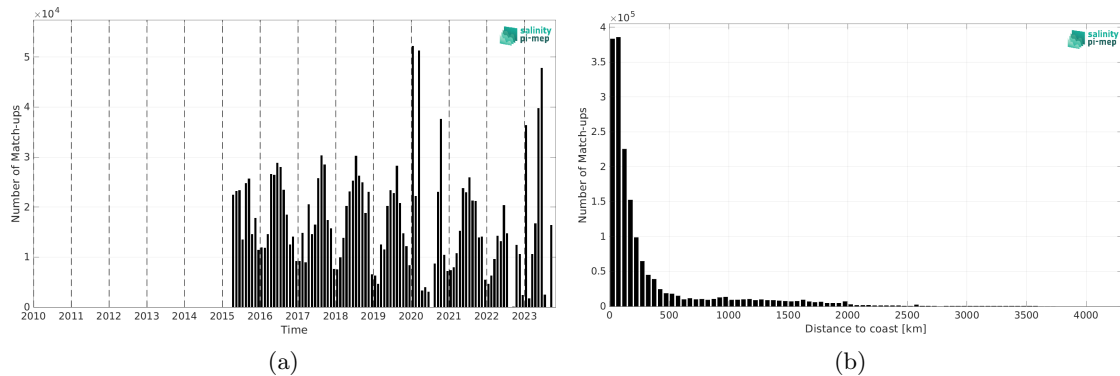
Figure 1: Number of match-ups between TSG (SAMOS) and SMAP SSS L3 v5 - Monthly (RSS) SSS as a function of time (a) and as function of the distance to coast (b) over the Global Ocean Pi-MEP region and for the full satellite product period.
