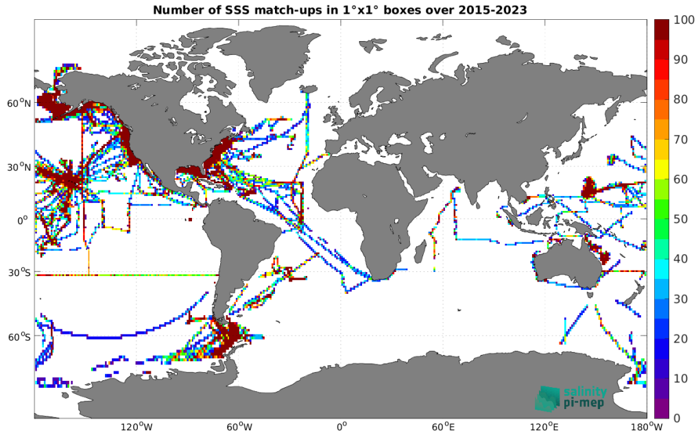
Figure 4: Number of SSS match-ups between TSG (SAMOS) SSS and the SMAP SSS L3 v5 - Monthly (RSS) SSS product for the Global Ocean Pi-MEP region over 1^\circ \times 1^\circ boxes and for the full satellite product period.
