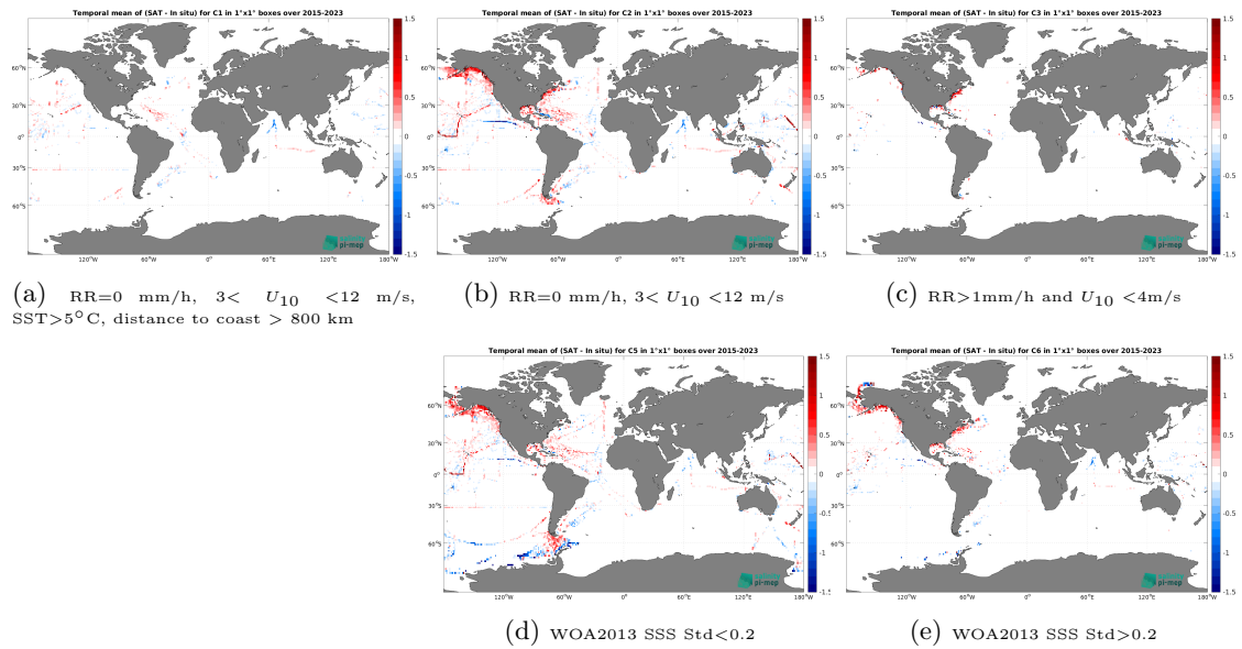
Figure 12: Temporal mean gridded over spatial boxes of size 1^\circ \times 1^\circ of \Delta SSS (SMAP SSS L3 v5 - Monthly (RSS) - TSG (SAMOS)) for 5 different subdatasets corresponding to:RR=0 mm/h, 3 < U_{10} < 12 m/s, SST >5^\circ C, distance to coast > 800 km (a), RR=0 mm/h, 3 < U_{10} < 12 m/s (b), RR >1 mm/h and U_{10} < 4 m/s (c), WOA2013 SSS Std <0.2 (d), WOA2013 SSS Std >0.2 (e).
