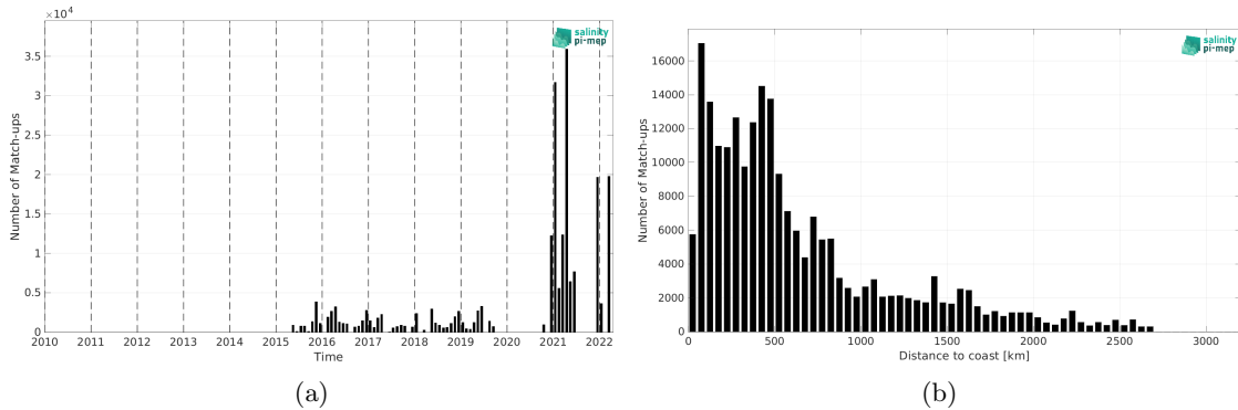
Figure 1: Number of match-ups between TSG (Polarstern) and SMAP SSS L3 v5 - Monthly (RSS) SSS as a function of time (a) and as function of the distance to coast (b) over the Global Ocean Pi-MEP region and for the full satellite product period.
