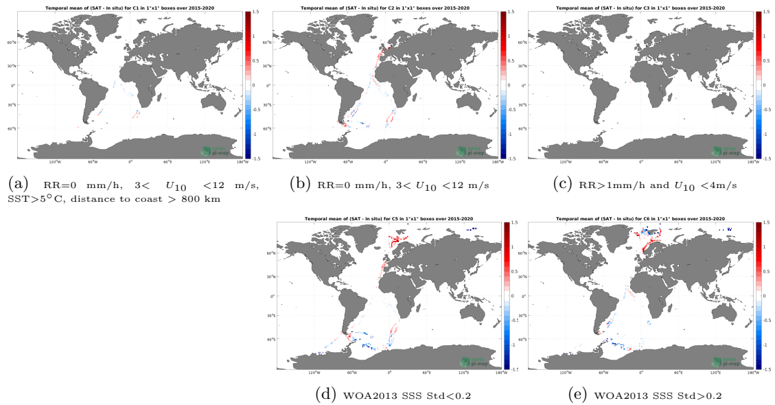
Figure 12: Temporal mean gridded over spatial boxes of size 1^\circ \times 1^\circ of \Delta SSS (SMAP SSS L3 v5 - Monthly (RSS) - TSG (Polarstern)) for 5 different subdatasets corresponding to:RR=0 mm/h, 3 < U_{10} < 12 m/s, SST >5^\circ C, distance to coast > 800 km (a), RR=0 mm/h, 3 < U_{10} < 12 m/s (b), RR >1 mm/h and U_{10} < 4 m/s (c), WOA2013 SSS Std <0.2 (d), WOA2013 SSS Std >0.2 (e).
