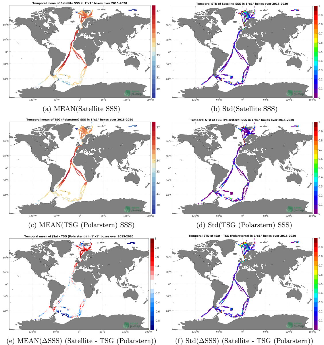
Figure 6: Temporal mean (left) and Std (right) of SSS from SMAP SSS L3 v5 - Monthly (RSS) (top), TSG (Polarstern) (middle), and of \Delta SSS (Satellite - TSG (Polarstern)). Only match-up pairs are used to generate these maps.
