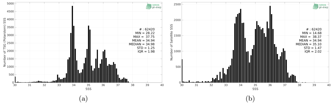
Figure 2: Histograms of SSS from TSG (Polarstern) (a) and SMAP SSS L3 v5 - Monthly (RSS) (b) considering all match-up pairs per bins of 0.1 over the Global Ocean Pi-MEP region and for the full satellite product period.
