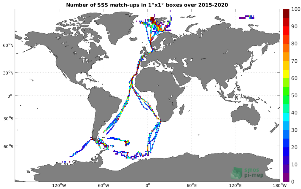
Figure 4: Number of SSS match-ups between TSG (Polarstern) SSS and the SMAP SSS L3 v5 - Monthly (RSS) SSS product for the Global Ocean Pi-MEP region over 1^\circ \times 1^\circ boxes and for the full satellite product period.
