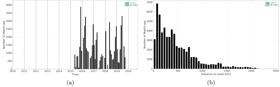
Figure 1: Number of match-ups between TSG (Polarstern) and SMAP SSS L3 v5 - Monthly (RSS) SSS as a function of time (a) and as function of the distance to coast (b) over the Global Ocean Pi-MEP region and for the full satellite product period.
