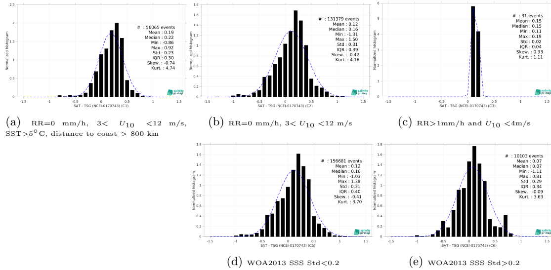
Figure 13: Normalized histogram of \Delta SSS (SMAP SSS L3 v5 - Monthly (RSS) - TSG (NCEI-0170743)) for 5 different subdatasets corresponding to: RR=0 mm/h, 3 < U_{10} < 12 m/s, SST>5°C, distance to coast > 800 km (a), RR=0 mm/h, 3 < U_{10} < 12 m/s (b), RR>1mm/h and U_{10} < 4 m/s (c), WOA2013 SSS Std<0.2 (d), WOA2013 SSS Std>0.2 (e).
