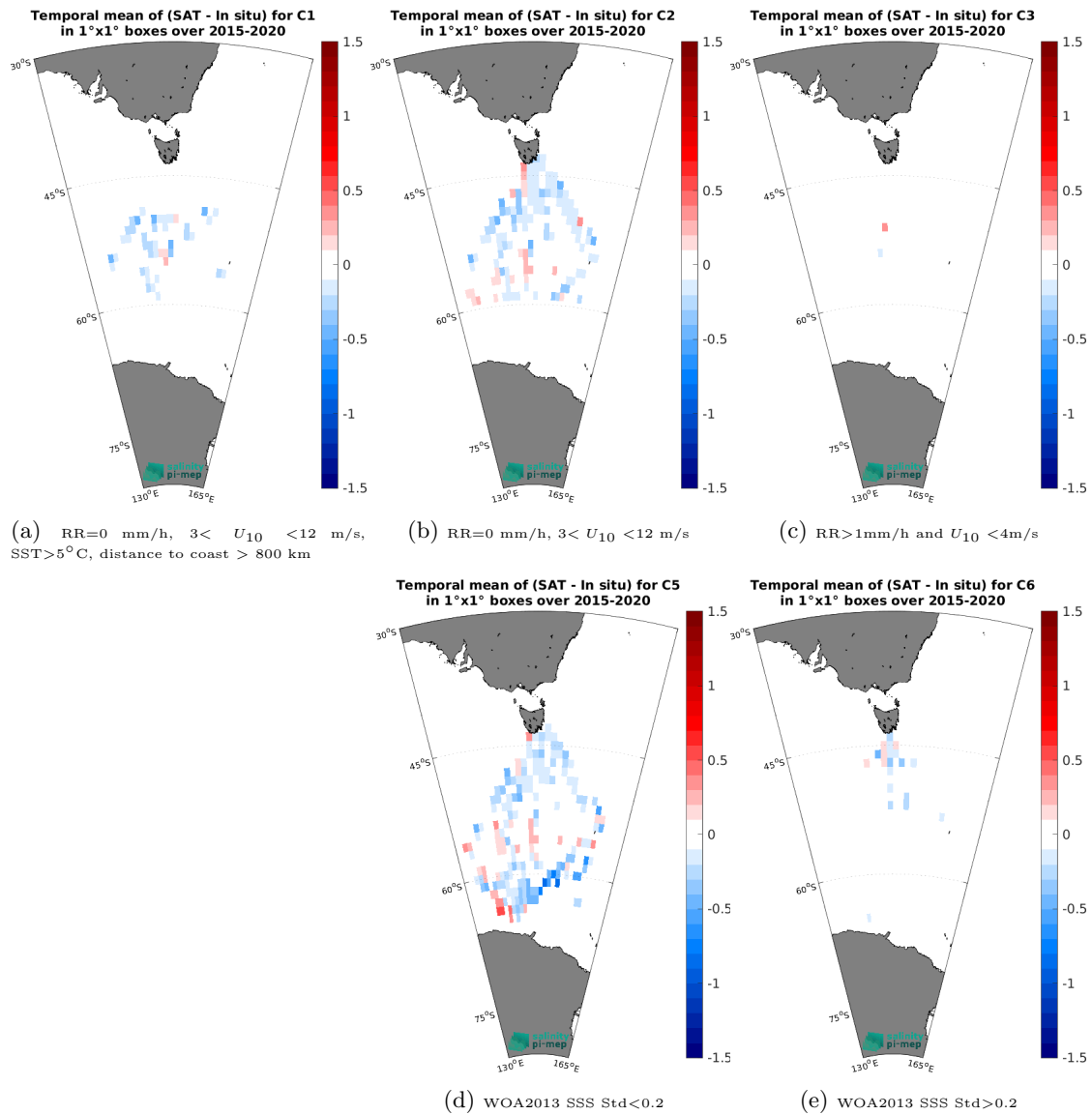
Figure 12: Temporal mean gridded over spatial boxes of size 1^\circ \times 1^\circ of \Delta\text{SSS} (SMAP SSS L3 v5 - Monthly (RSS) - TSG (LEGOS-Survostral)) for 5 different subdatasets corresponding to: RR=0 mm/h, 3 < U_{10} < 12 m/s, SST > 5^\circ\text{C} , distance to coast > 800 km (a), RR=0 mm/h, 3 < U_{10} < 12 m/s (b), RR > 1\text{mm/h} and U_{10} < 4\text{m/s} (c), WOA2013 SSS Std < 0.2 (d), WOA2013 SSS Std > 0.2 (e).
