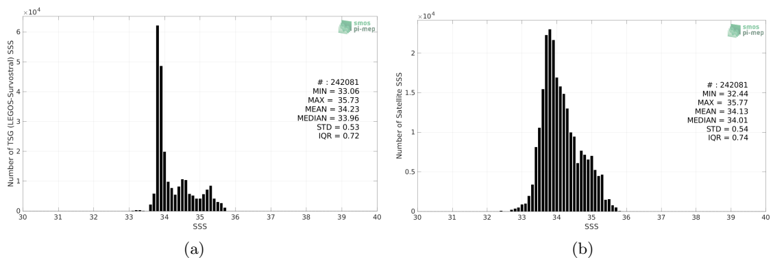
Figure 2: Histograms of SSS from TSG (LEGOS-Survostral) (a) and SMAP SSS L3 v5 - Monthly (RSS) (b) considering all match-up pairs per bins of 0.1 over the Global Ocean Pi-MEP region and for the full satellite product period.
