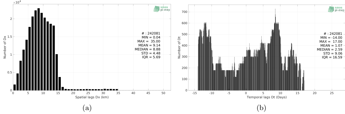
Figure 5: Histograms of the spatial (a) and temporal (b) lags between the location/time of the TSG (LEGOS-Survostral) measurement and the date of the corresponding SMAP SSS L3 v5 - Monthly (RSS) SSS pixel.
