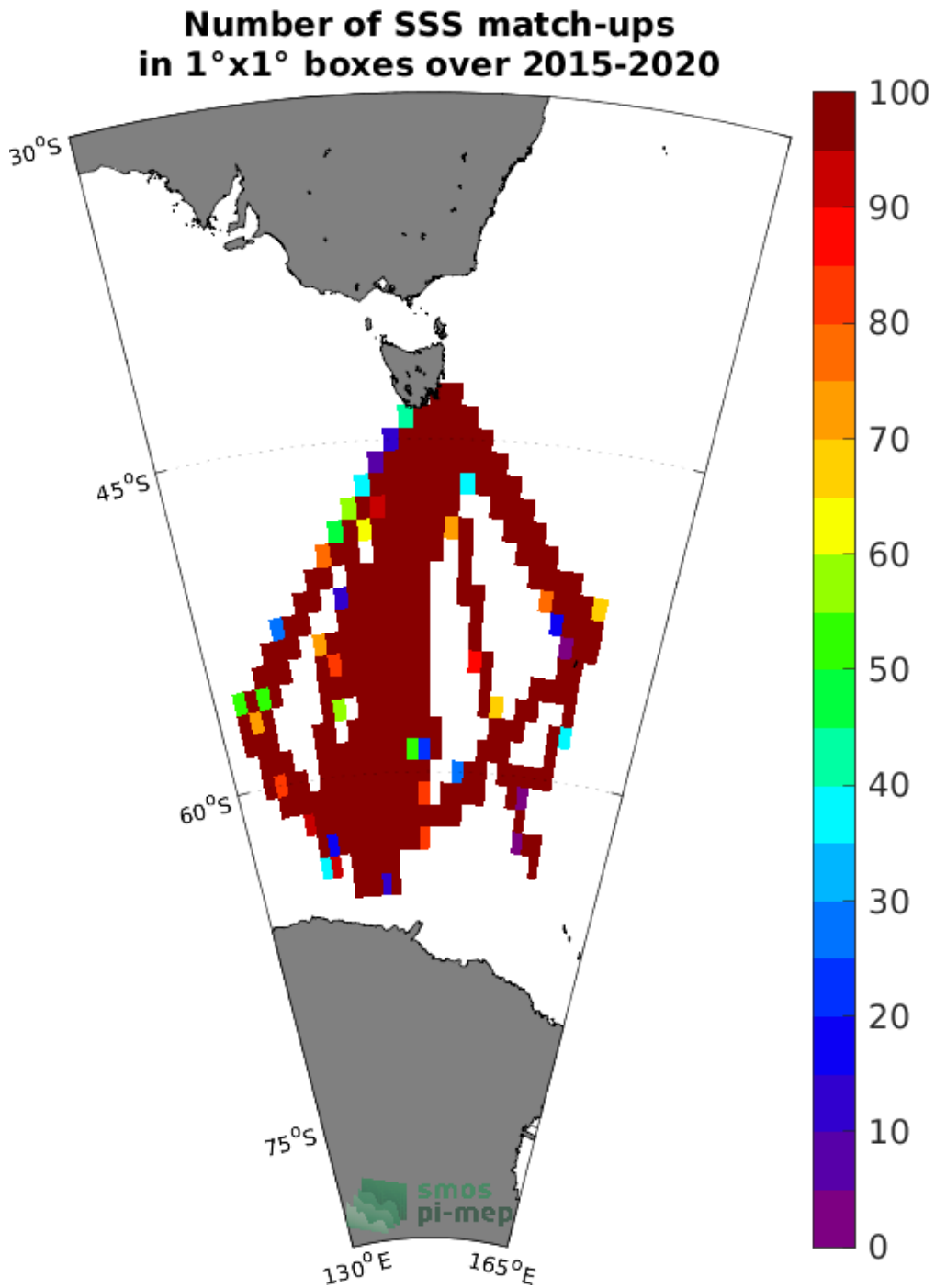
Figure 4: Number of SSS match-ups between TSG (LEGOS-Survostral) SSS and the SMAP SSS L3 v5 - Monthly (RSS) SSS product for the Global Ocean Pi-MEP region over 1°x1° boxes and for the full satellite product period.
