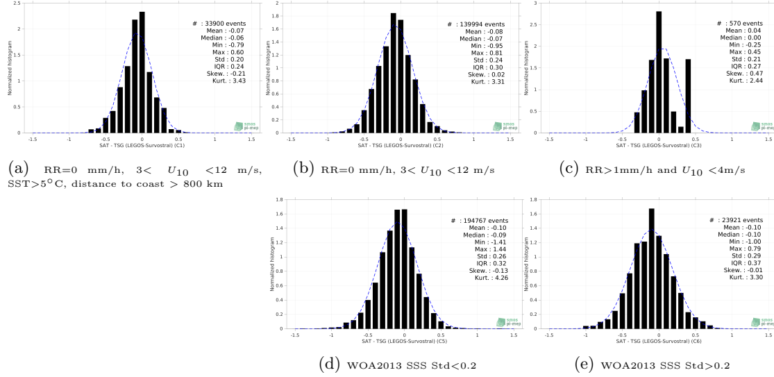
Figure 13: Normalized histogram of \Delta SSS (SMAP SSS L3 v5 - Monthly (RSS) - TSG (LEGOS-Survostral)) for 5 different subdatasets corresponding to: RR=0 mm/h, 3 < U_{10} < 12 m/s, SST > 5°C, distance to coast > 800 km (a), RR=0 mm/h, 3 < U_{10} < 12 m/s (b), RR > 1mm/h and U_{10} < 4 m/s (c), WOA2013 SSS Std < 0.2 (d), WOA2013 SSS Std > 0.2 (e).
