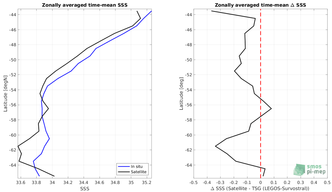
Figure 8: Left panel: Zonal mean SSS from SMAP SSS L3 v5 - Monthly (RSS) satellite product (black) and from TSG (LEGOS-Survostral) (blue). Right panel: Zonal mean of \Delta SSS (Satellite - TSG (LEGOS-Survostral)) for all the collected Pi-MEP match-up pairs estimated over the full satellite product period.
