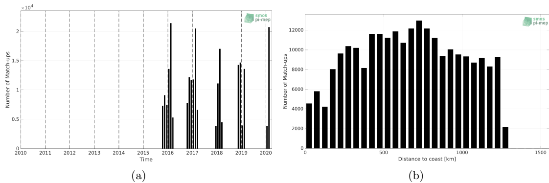
Figure 1: Number of match-ups between TSG (LEGOS-Survostral) and SMAP SSS L3 v5 - Monthly (RSS) SSS as a function of time (a) and as function of the distance to coast (b) over the Global Ocean Pi-MEP region and for the full satellite product period.
