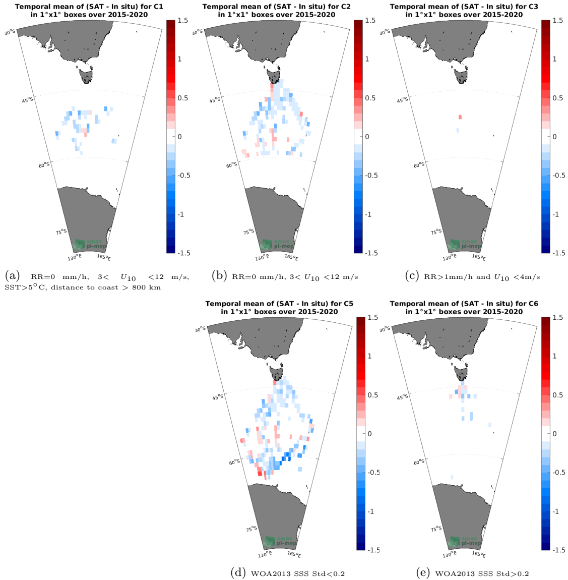
Figure 12: Temporal mean gridded over spatial boxes of size 1^\circ \times 1^\circ of \Delta SSS (SMAP SSS L3 v5 - Monthly (RSS) - TSG (LEGOS-Survostral)) for 5 different subdatasets corresponding to:RR=0 mm/h, 3 < U_{10} < 12 m/s, SST>5°C, distance to coast > 800 km (a), RR=0 mm/h, 3 < U_{10} < 12 m/s (b), RR>1mm/h and U_{10} < 4 m/s (c), WOA2013 SSS Std<0.2 (d), WOA2013 SSS Std>0.2 (e).
