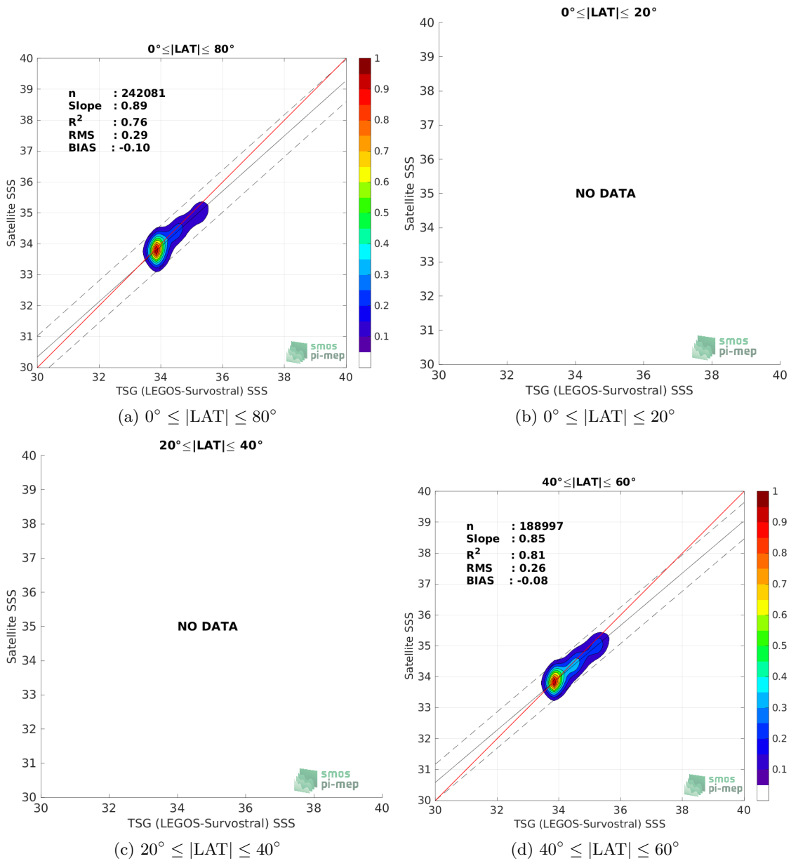
Figure 9: Contour maps of the concentration of SMAP SSS L3 v5 - Monthly (RSS) SSS (y-axis) versus TSG (LEGOS-Survostral) SSS (x-axis) at match-up pairs for different latitude bands. For each plot, the red line shows x=y . The black thin and dashed lines indicate a linear fit through the data cloud and the \pm 95\% confidence levels, respectively. The number match-up pairs n , the slope and R^2 coefficient of the linear fit, the root mean square (RMS) and the mean bias between satellite and in situ data are indicated for each latitude band in each plots.
