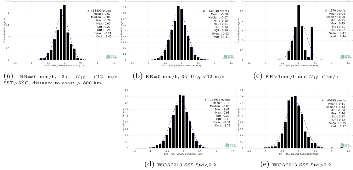
Figure 13: Normalized histogram of \Delta SSS (SMAP SSS L3 v5 - Monthly (RSS) - TSG (LEGOS-Survostral)) for 5 different subdatasets corresponding to: RR=0 mm/h, 3 < U_{10} < 12 m/s, SST > 5°C, distance to coast > 800 km (a), RR=0 mm/h, 3 < U_{10} < 12 m/s (b), RR > 1mm/h and U_{10} < 4 m/s (c), WOA2013 SSS Std < 0.2 (d), WOA2013 SSS Std > 0.2 (e).
