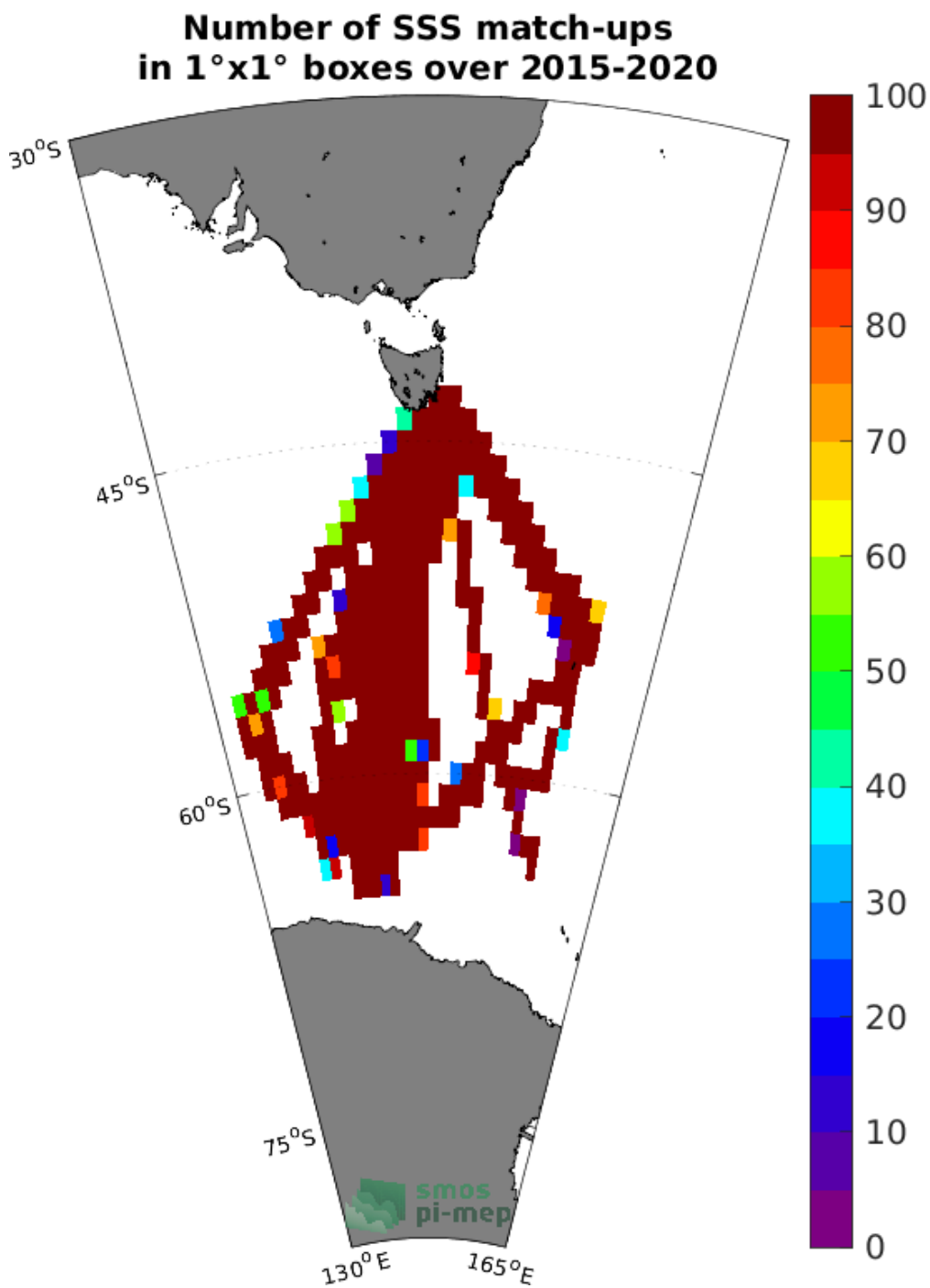
Figure 4: Number of SSS match-ups between TSG (LEGOS-Survostral) SSS and the SMAP SSS L3 v5 - Monthly (RSS) SSS product for the Global Ocean Pi-MEP region over 1°x1° boxes and for the full satellite product period.
