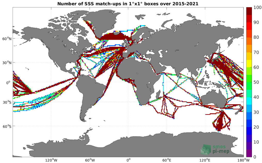
Figure 4: Number of SSS match-ups between TSG (LEGOS-DM) SSS and the SMAP SSS L3 v5 - Monthly (RSS) SSS product for the Global Ocean Pi-MEP region over 1^\circ \times 1^\circ boxes and for the full satellite product period.
