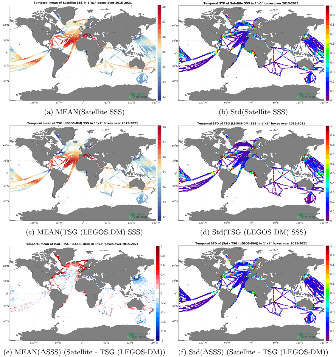
Figure 6: Temporal mean (left) and Std (right) of SSS from SMAP SSS L3 v5 - Monthly (RSS) (top), TSG (LEGOS-DM) (middle), and of \Delta SSS (Satellite - TSG (LEGOS-DM)). Only match-pair are used to generate these maps.
