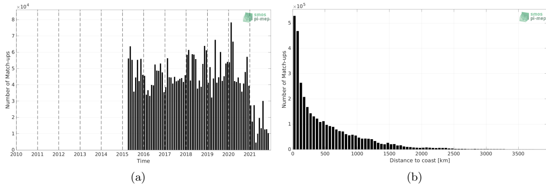
Figure 1: Number of match-ups between TSG (LEGOS-DM) and SMAP SSS L3 v5 - Monthly (RSS) SSS as a function of time (a) and as function of the distance to coast (b) over the Global Ocean Pi-MEP region and for the full satellite product period.
