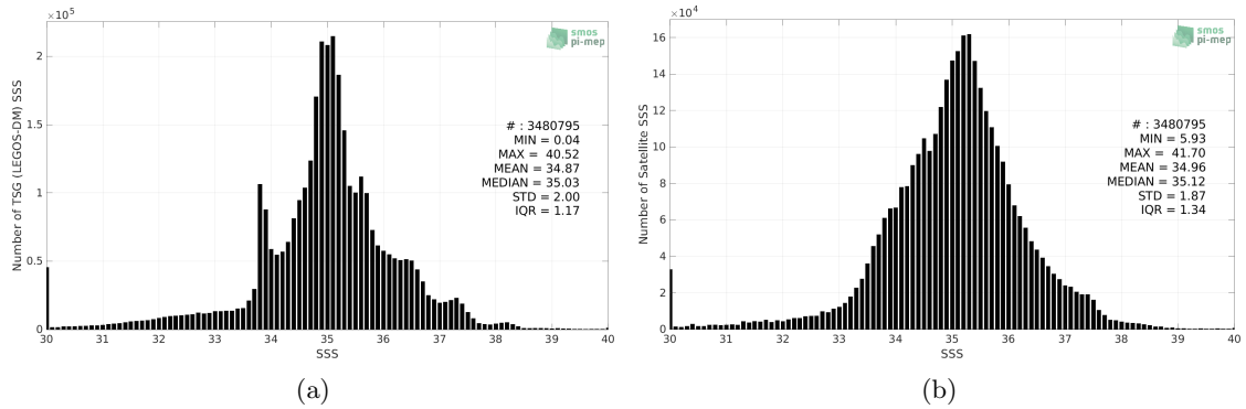
Figure 2: Histograms of SSS from TSG (LEGOS-DM) (a) and SMAP SSS L3 v5 - Monthly (RSS) (b) considering all match-up pairs per bins of 0.1 over the Global Ocean Pi-MEP region and for the full satellite product period.
