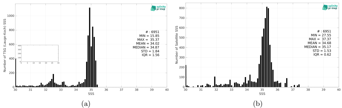
Figure 2: Histograms of SSS from TSG (Lauge-Koch) (a) and SMAP SSS L3 v5 - Monthly (RSS) (b) considering all match-up pairs per bins of 0.1 over the Global Ocean Pi-MEP region and for the full satellite product period.
