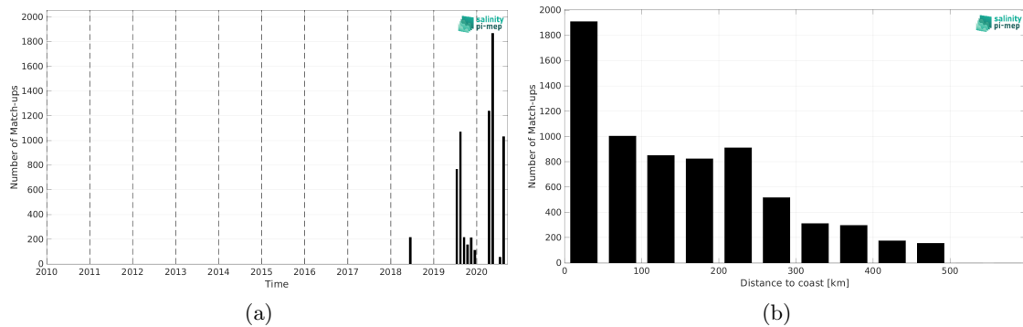
Figure 1: Number of match-ups between TSG (Lauge-Koch) and SMAP SSS L3 v5 - Monthly (RSS) SSS as a function of time (a) and as function of the distance to coast (b) over the Global Ocean Pi-MEP region and for the full satellite product period.
