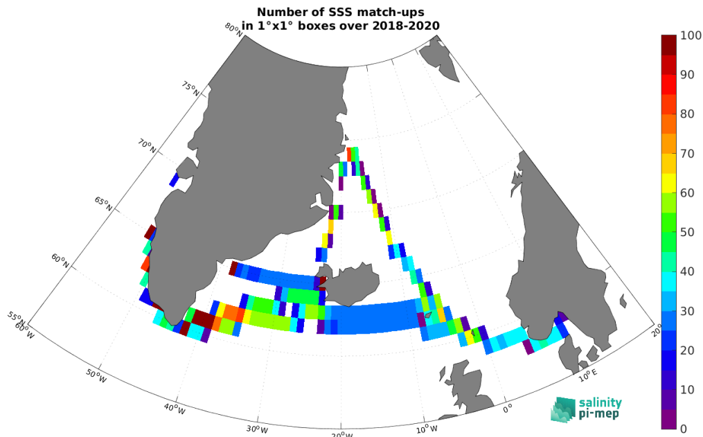
Figure 4: Number of SSS match-ups between TSG (Lauge-Koch) SSS and the SMAP SSS L3 v5 - Monthly (RSS) SSS product for the Global Ocean Pi-MEP region over 1^\circ \times 1^\circ boxes and for the full satellite product period.
