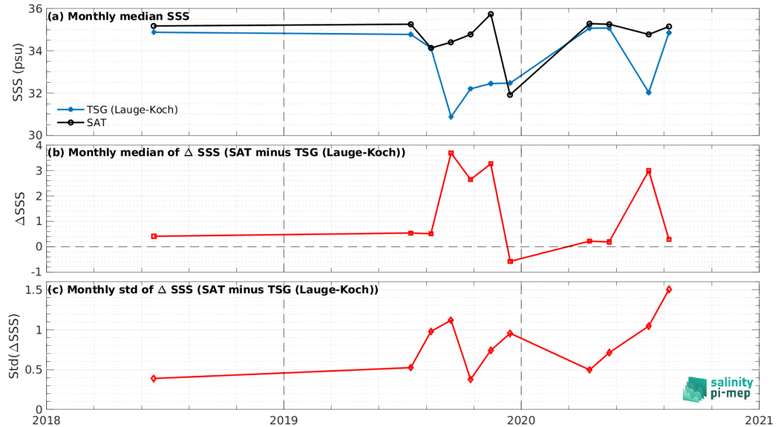
Figure 7: Time series of the monthly median SSS (top), median of \Delta\text{SSS} (Satellite - TSG (Lauge-Koch)) and Std of \Delta\text{SSS} (Satellite - TSG (Lauge-Koch)) over the Global Ocean Pi-MEP region considering all match-ups collected by the Pi-MEP.
