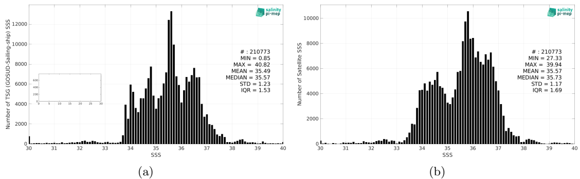
Figure 2: Histograms of SSS from TSG (GOSUD-Sailing-ship) (a) and SMAP SSS L3 v5 - Monthly (RSS) (b) considering all match-up pairs per bins of 0.1 over the Global Ocean Pi-MEP region and for the full satellite product period.
