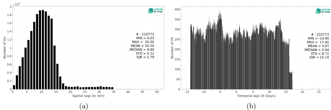
Figure 5: Histograms of the spatial (a) and temporal (b) lags between the location/time of the TSG (GOSUD-Sailing-ship) measurement and the date of the corresponding SMAP SSS L3 v5 - Monthly (RSS) SSS pixel.
