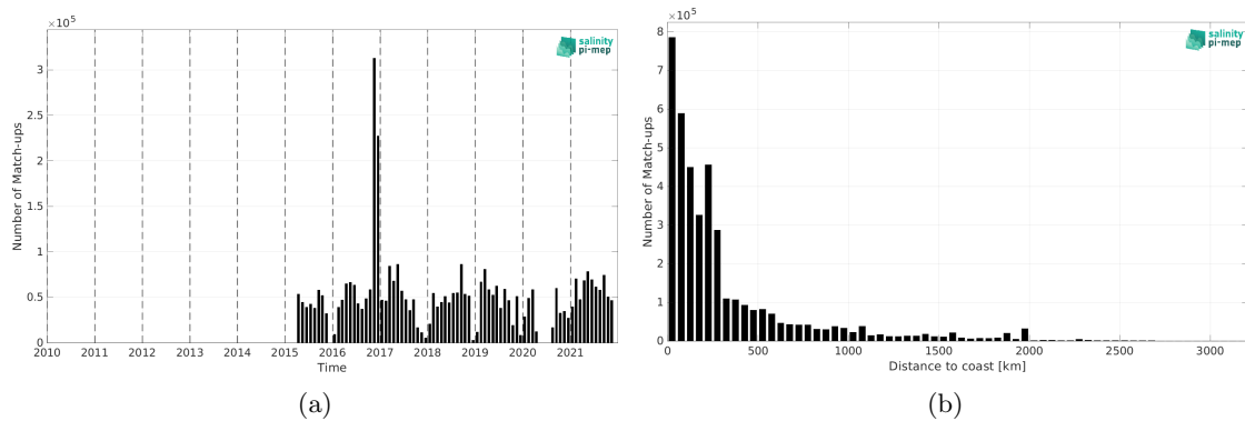
Figure 1: Number of match-ups between TSG (GOSUD-Research-vessel) and SMAP SSS L3 v5 - Monthly (RSS) SSS as a function of time (a) and as function of the distance to coast (b) over the Global Ocean Pi-MEP region and for the full satellite product period.
