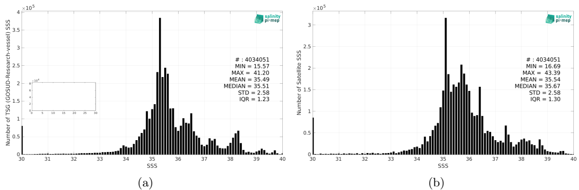
Figure 2: Histograms of SSS from TSG (GOSUD-Research-vessel) (a) and SMAP SSS L3 v5 - Monthly (RSS) (b) considering all match-up pairs per bins of 0.1 over the Global Ocean Pi-MEP region and for the full satellite product period.
