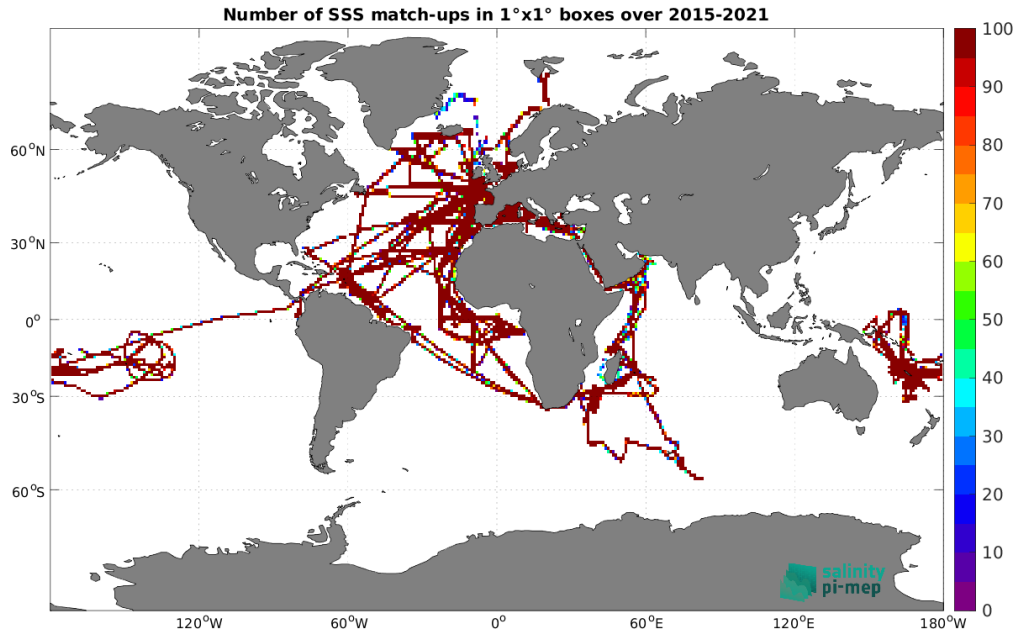
Figure 4: Number of SSS match-ups between TSG (GOSUD-Research-vessel) SSS and the SMAP SSS L3 v5 - Monthly (RSS) SSS product for the Global Ocean Pi-MEP region over 1^\circ \times 1^\circ boxes and for the full satellite product period.
