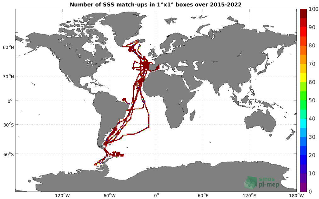
Figure 4: Number of SSS match-ups between TSG (CSIC-UTM) SSS and the SMAP SSS L3 v5 - Monthly (RSS) SSS product for the Global Ocean Pi-MEP region over 1°x1° boxes and for the full satellite product period.
