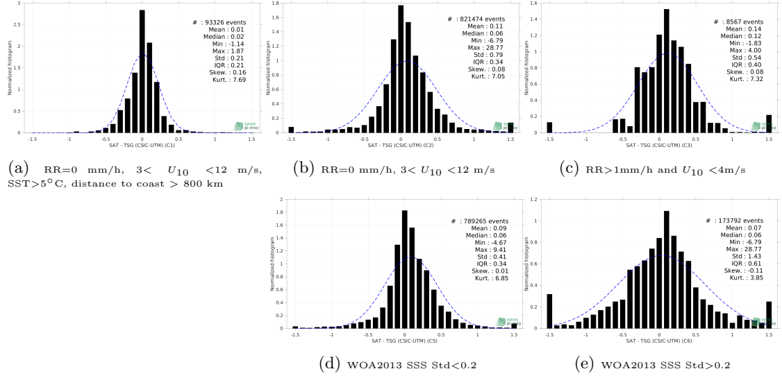
Figure 13: Normalized histogram of \Delta SSS (SMAP SSS L3 v5 - Monthly (RSS) - TSG (CSIC-UTM)) for 5 different subdatasets corresponding to: RR=0 mm/h, 3 < U_{10} < 12 m/s, SST>5°C, distance to coast > 800 km (a), RR=0 mm/h, 3 < U_{10} < 12 m/s (b), RR>1mm/h and U_{10} < 4 m/s (c), WOA2013 SSS Std<0.2 (d), WOA2013 SSS Std>0.2 (e).
