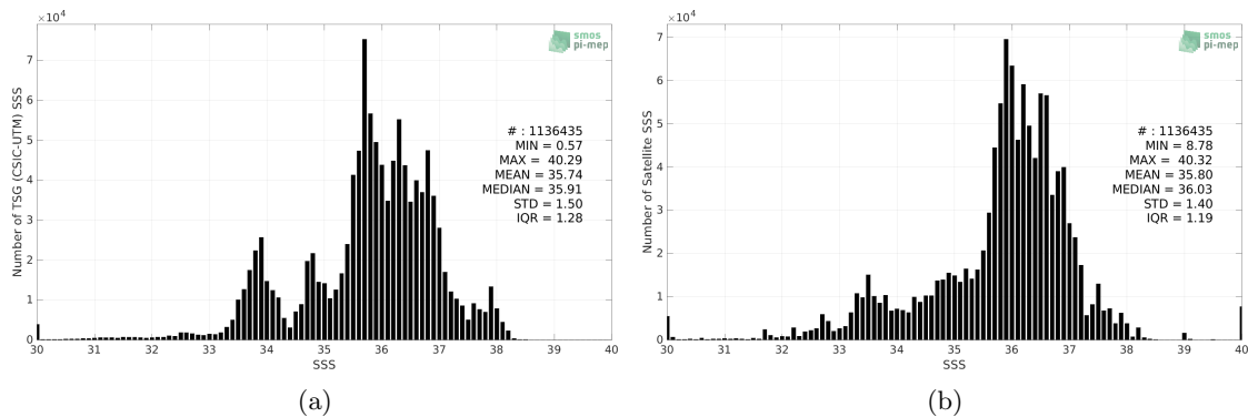
Figure 2: Histograms of SSS from TSG (CSIC-UTM) (a) and SMAP SSS L3 v5 - Monthly (RSS) (b) considering all match-up pairs per bins of 0.1 over the Global Ocean Pi-MEP region and for the full satellite product period.
