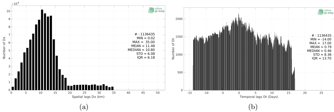
Figure 5: Histograms of the spatial (a) and temporal (b) lags between the location/time of the TSG (CSIC-UTM) measurement and the date of the corresponding SMAP SSS L3 v5 - Monthly (RSS) SSS pixel.
