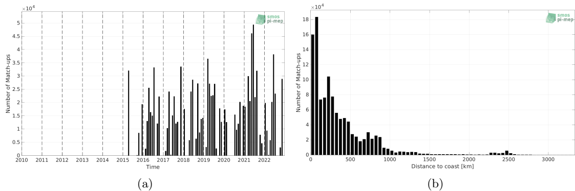
Figure 1: Number of match-ups between TSG (CSIC-UTM) and SMAP SSS L3 v5 - Monthly (RSS) SSS as a function of time (a) and as function of the distance to coast (b) over the Global Ocean Pi-MEP region and for the full satellite product period.
