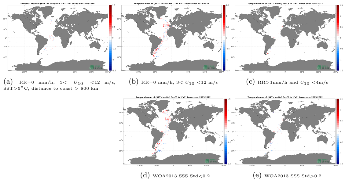
Figure 12: Temporal mean gridded over spatial boxes of size 1^\circ \times 1^\circ of \Delta SSS (SMAP SSS L3 v5 - Monthly (RSS) - TSG (CSIC-UTM)) for 5 different subdatasets corresponding to:RR=0 mm/h, 3 < U_{10} < 12 m/s, SST > 5^\circ\text{C} , distance to coast > 800 km (a), RR=0 mm/h, 3 < U_{10} < 12 m/s (b), RR > 1 mm/h and U_{10} < 4 m/s (c), WOA2013 SSS Std < 0.2 (d), WOA2013 SSS Std > 0.2 (e).
