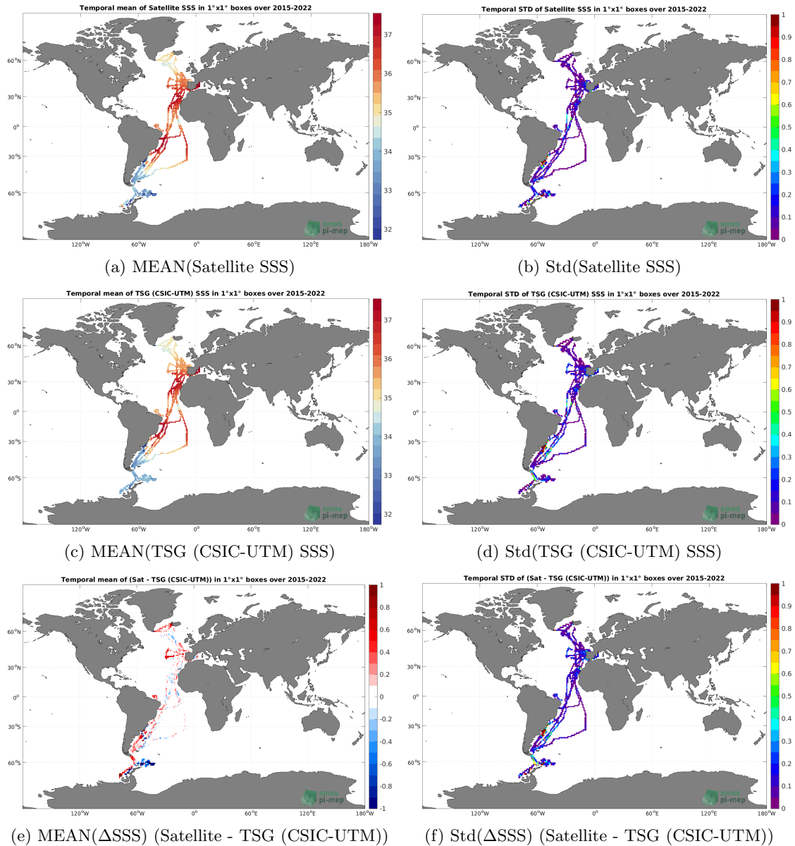
Figure 6: Temporal mean (left) and Std (right) of SSS from SMAP SSS L3 v5 - Monthly (RSS) (top), TSG (CSIC-UTM) (middle), and of \Delta SSS (Satellite - TSG (CSIC-UTM)). Only match-up pairs are used to generate these maps.
