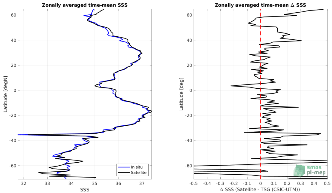
Figure 8: Left panel: Zonal mean SSS from SMAP SSS L3 v5 - Monthly (RSS) satellite product (black) and from TSG (CSIC-UTM) (blue). Right panel: Zonal mean of \Delta SSS (Satellite - TSG (CSIC-UTM)) for all the collected Pi-MEP match-up pairs estimated over the full satellite product period.
