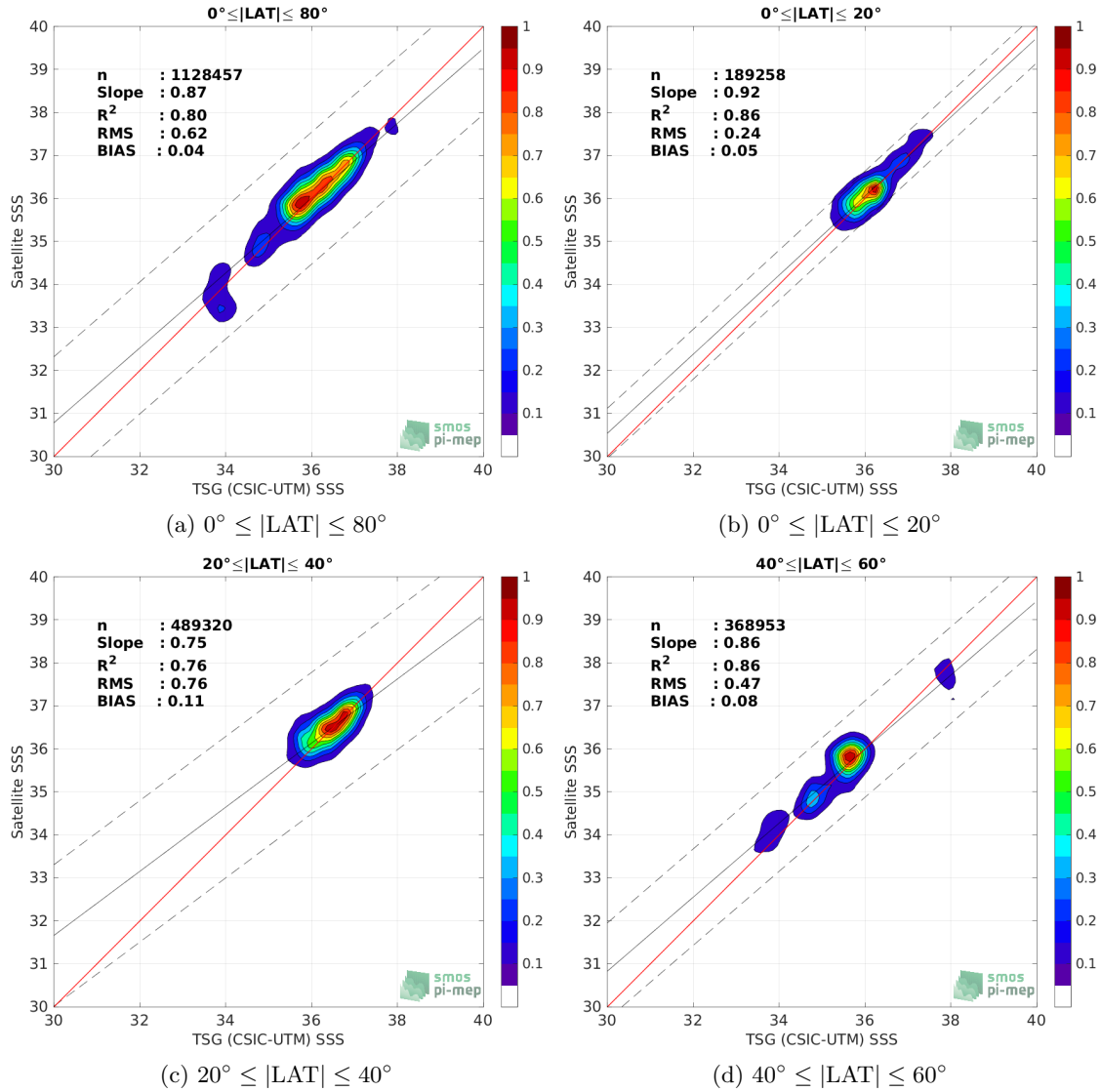
Figure 9: Contour maps of the concentration of SMAP SSS L3 v5 - Monthly (RSS) SSS (y-axis) versus TSG (CSIC-UTM) SSS (x-axis) at match-up pairs for different latitude bands. For each plot, the red line shows x=y . The black thin and dashed lines indicate a linear fit through the data cloud and the \pm 95\% confidence levels, respectively. The number match-up pairs n , the slope and R^2 coefficient of the linear fit, the root mean square (RMS) and the mean bias between satellite and in situ data are indicated for each latitude band in each plots.
