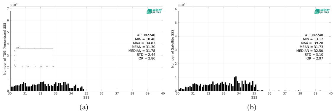
Figure 2: Histograms of SSS from TSG (Amundsen) (a) and SMAP SSS L3 v5 - Monthly (RSS) (b) considering all match-up pairs per bins of 0.1 over the Global Ocean Pi-MEP region and for the full satellite product period.
