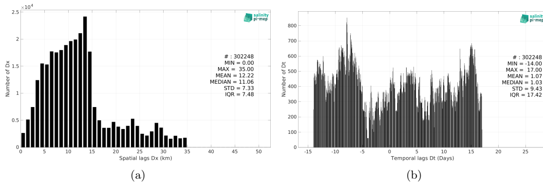
Figure 5: Histograms of the spatial (a) and temporal (b) lags between the location/time of the TSG (Amundsen) measurement and the date of the corresponding SMAP SSS L3 v5 - Monthly (RSS) SSS pixel.
