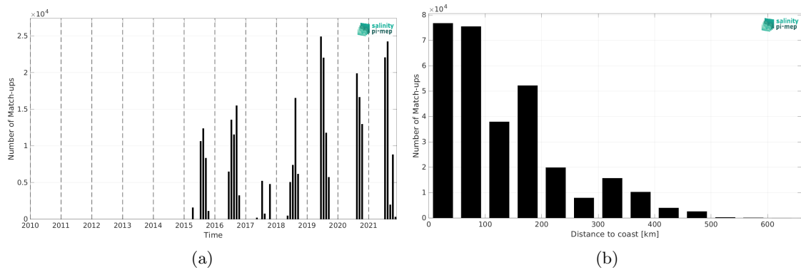
Figure 1: Number of match-ups between TSG (Amundsen) and SMAP SSS L3 v5 - Monthly (RSS) SSS as a function of time (a) and as function of the distance to coast (b) over the Global Ocean Pi-MEP region and for the full satellite product period.
