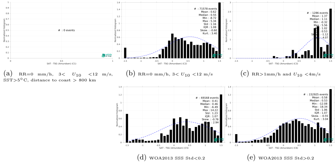
Figure 13: Normalized histogram of \Delta SSS (SMAP SSS L3 v5 - Monthly (RSS) - TSG (Amundsen)) for 5 different subdatasets corresponding to: RR=0 mm/h, 3 < U_{10} < 12 m/s, SST > 5°C, distance to coast > 800 km (a), RR=0 mm/h, 3 < U_{10} < 12 m/s (b), RR > 1mm/h and U_{10} < 4 m/s (c), WOA2013 SSS Std < 0.2 (d), WOA2013 SSS Std > 0.2 (e).
