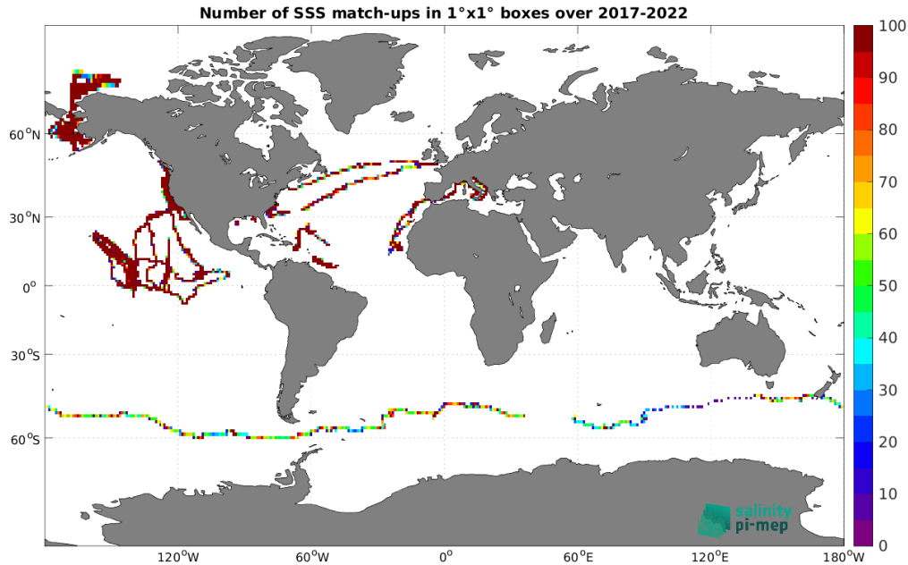
Figure 4: Number of SSS match-ups between Saildrone SSS and the SMAP SSS L3 v5 - Monthly (RSS) SSS product for the Global Ocean Pi-MEP region over 1^\circ \times 1^\circ boxes and for the full satellite product period.
