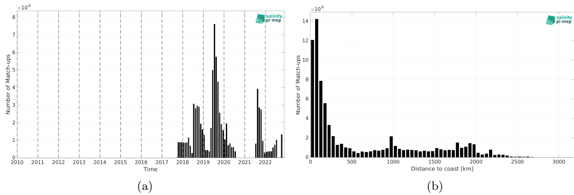
Figure 1: Number of match-ups between Sairdrone and SMAP SSS L3 v5 - Monthly (RSS) SSS as a function of time (a) and as function of the distance to coast (b) over the Global Ocean Pi-MEP region and for the full satellite product period.
