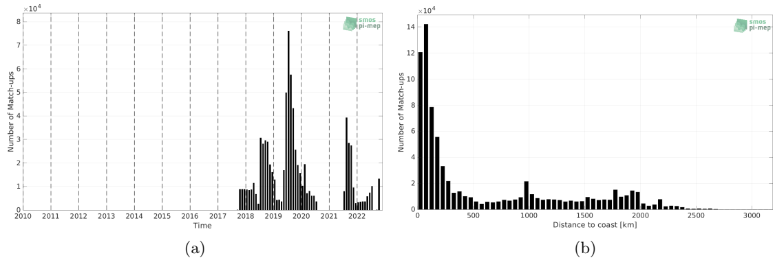
Figure 1: Number of match-ups between Saildrone and SMAP SSS L3 v5 - Monthly (RSS) SSS as a function of time (a) and as function of the distance to coast (b) over the Global Ocean Pi-MEP region and for the full satellite product period.
