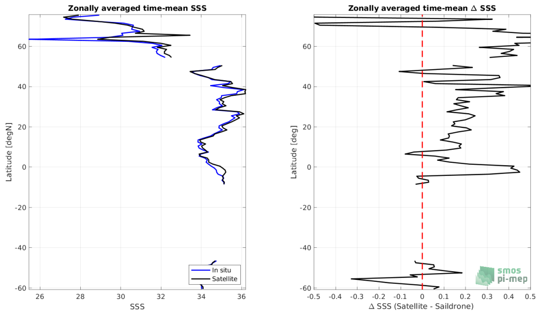
Figure 8: Left panel: Zonal mean SSS from SMAP SSS L3 v5 - Monthly (RSS) satellite product (black) and from Saildrone (blue). Right panel: Zonal mean of \Delta SSS (Satellite - Saildrone) for all the collected Pi-MEP match-up pairs estimated over the full satellite product period.
