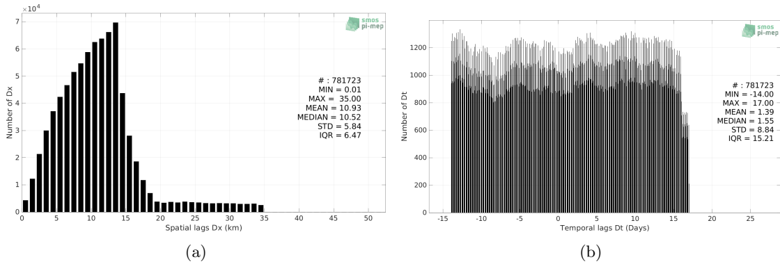
Figure 5: Histograms of the spatial (a) and temporal (b) lags between the location/time of the Sairdrone measurement and the date of the corresponding SMAP SSS L3 v5 - Monthly (RSS) SSS pixel.
