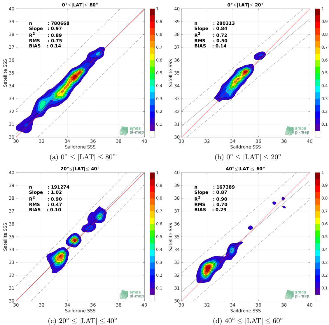
Figure 9: Contour maps of the concentration of SMAP SSS L3 v5 - Monthly (RSS) SSS (y-axis) versus Saildrone SSS (x-axis) at match-up pairs for different latitude bands. For each plot, the red line shows x=y . The black thin and dashed lines indicate a linear fit through the data cloud and the \pm 95\% confidence levels, respectively. The number match-up pairs n , the slope and R^2 coefficient of the linear fit, the root mean square (RMS) and the mean bias between satellite and in situ data are indicated for each latitude band in each plots.
