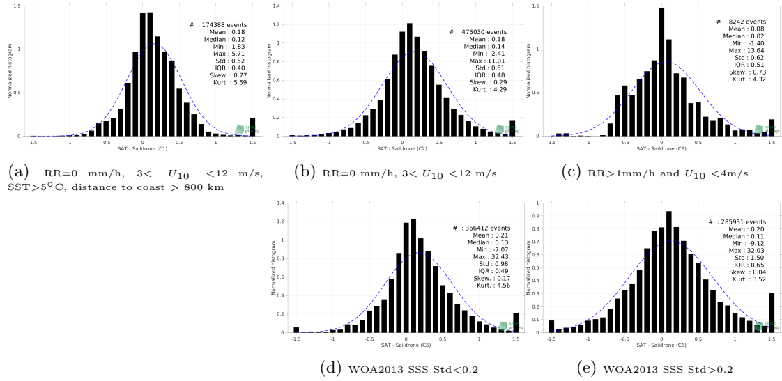
Figure 13: Normalized histogram of \Delta SSS (SMAP SSS L3 v5 - Monthly (RSS) - Saildrone) for 5 different subdatasets corresponding to: RR=0 mm/h, 3 < U_{10} < 12 m/s, SST>5°C, distance to coast > 800 km (a), RR=0 mm/h, 3 < U_{10} < 12 m/s (b), RR>1mm/h and U_{10} < 4 m/s (c), WOA2013 SSS Std<0.2 (d), WOA2013 SSS Std>0.2 (e).
