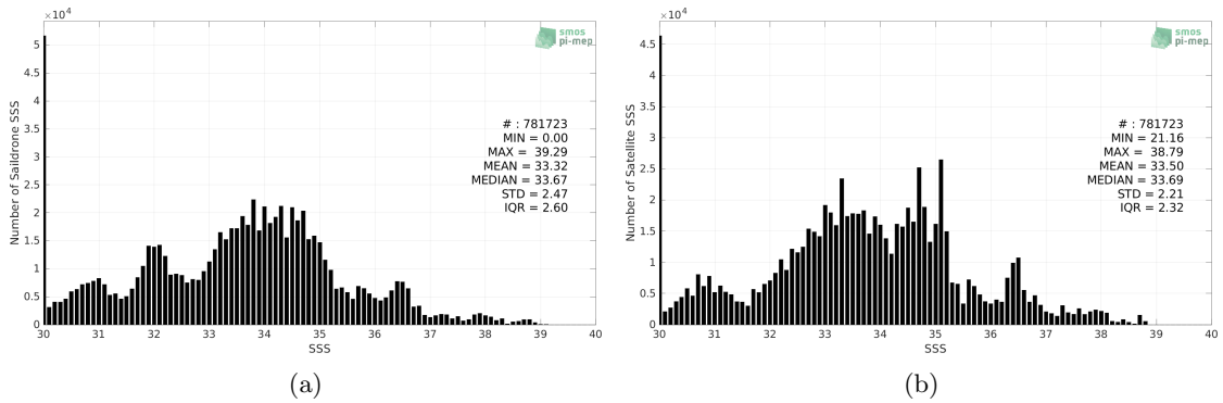
Figure 2: Histograms of SSS from Saildrone (a) and SMAP SSS L3 v5 - Monthly (RSS) (b) considering all match-up pairs per bins of 0.1 over the Global Ocean Pi-MEP region and for the full satellite product period.
