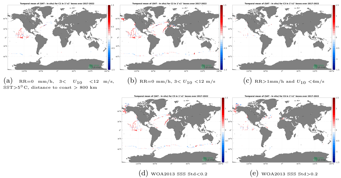
Figure 12: Temporal mean gridded over spatial boxes of size 1^\circ \times 1^\circ of \Delta SSS (SMAP SSS L3 v5 - Monthly (RSS) - Saildrone) for 5 different subdatasets corresponding to:RR=0 mm/h, 3 < U_{10} < 12 m/s, SST > 5^\circ\text{C} , distance to coast > 800 km (a), RR=0 mm/h, 3 < U_{10} < 12 m/s (b), RR > 1 mm/h and U_{10} < 4 m/s (c), WOA2013 SSS Std < 0.2 (d), WOA2013 SSS Std > 0.2 (e).
