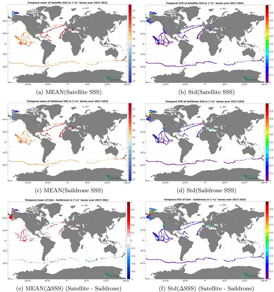
Figure 6: Temporal mean (left) and Std (right) of SSS from SMAP SSS L3 v5 - Monthly (RSS) (top), Saildrone (middle), and of \Delta SSS (Satellite - Saildrone). Only match-up pairs are used to generate these maps.
