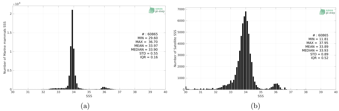
Figure 2: Histograms of SSS from Marine mammals (a) and SMAP SSS L3 v5 - Monthly (RSS) (b) considering all match-up pairs per bins of 0.1 over the Global Ocean Pi-MEP region and for the full satellite product period.
