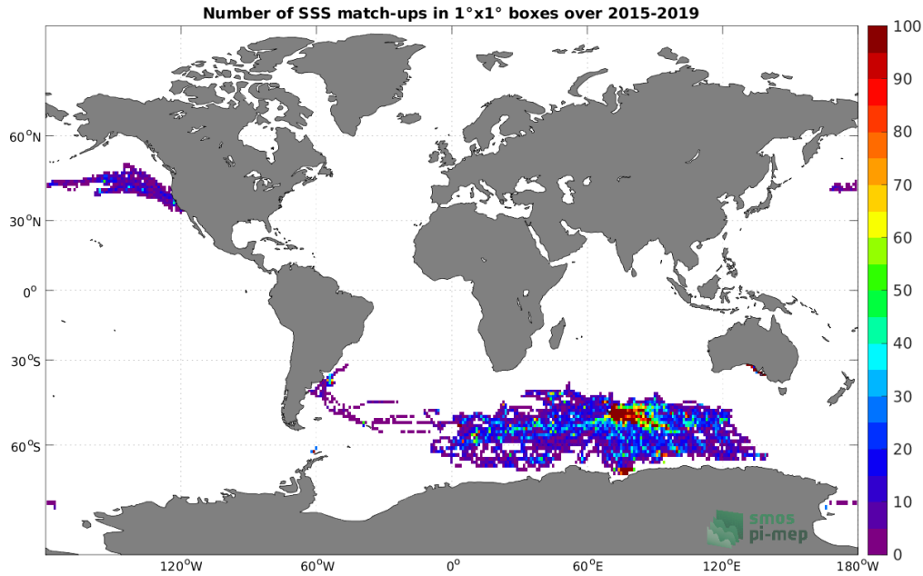
Figure 4: Number of SSS match-ups between Marine mammals SSS and the SMAP SSS L3 v5 - Monthly (RSS) SSS product for the Global Ocean Pi-MEP region over 1°×1° boxes and for the full satellite product period.
