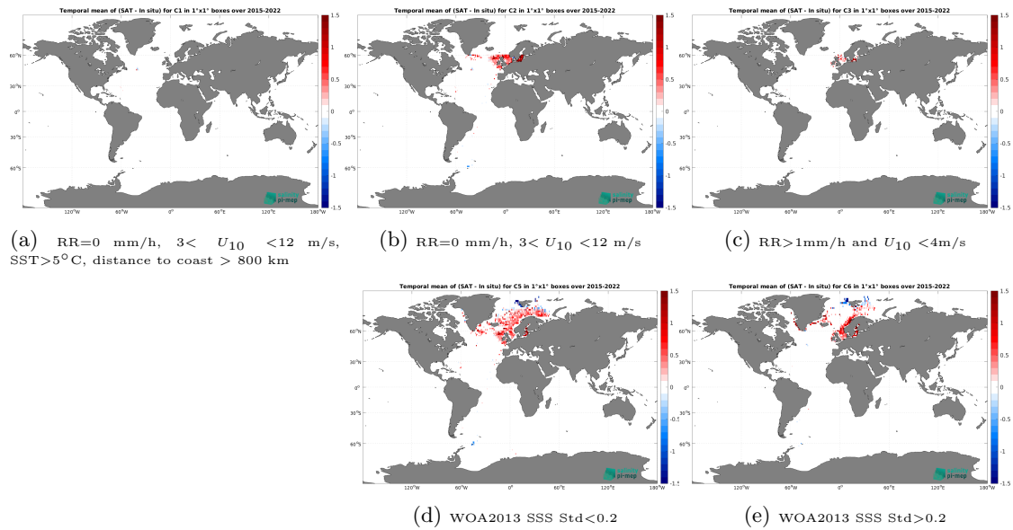
Figure 12: Temporal mean gridded over spatial boxes of size 1^\circ \times 1^\circ of \Delta SSS (SMAP SSS L3 v5 - Monthly (RSS) - ICES) for 5 different subdatasets corresponding to:RR=0 mm/h, 3 < U_{10} < 12 m/s, SST > 5^\circ\text{C} , distance to coast > 800 km (a), RR=0 mm/h, 3 < U_{10} < 12 m/s (b), RR > 1 mm/h and U_{10} < 4 m/s (c), WOA2013 SSS Std < 0.2 (d), WOA2013 SSS Std > 0.2 (e).
