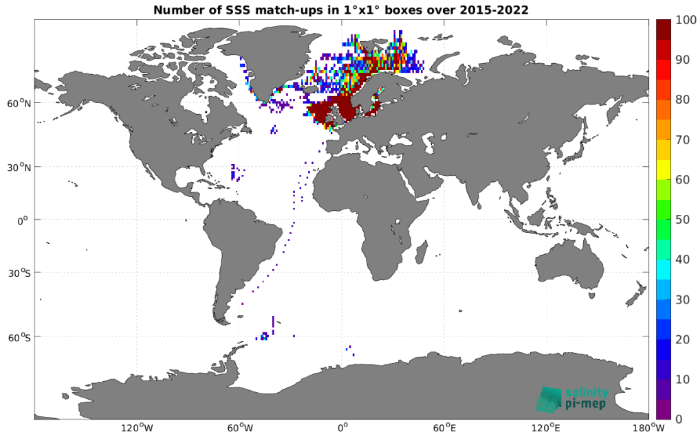
Figure 4: Number of SSS match-ups between ICES SSS and the SMAP SSS L3 v5 - Monthly (RSS) SSS product for the Global Ocean Pi-MEP region over 1^\circ \times 1^\circ boxes and for the full satellite product period.
