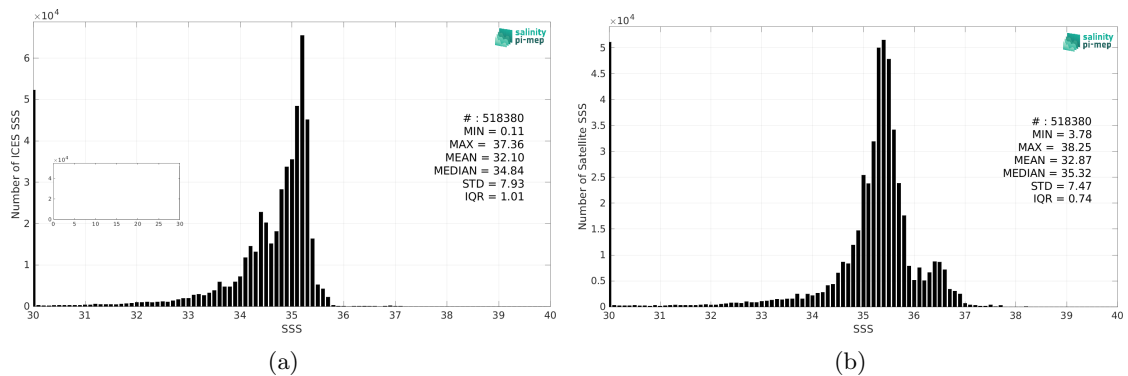
Figure 2: Histograms of SSS from ICES (a) and SMAP SSS L3 v5 - Monthly (RSS) (b) considering all match-up pairs per bins of 0.1 over the Global Ocean Pi-MEP region and for the full satellite product period.
