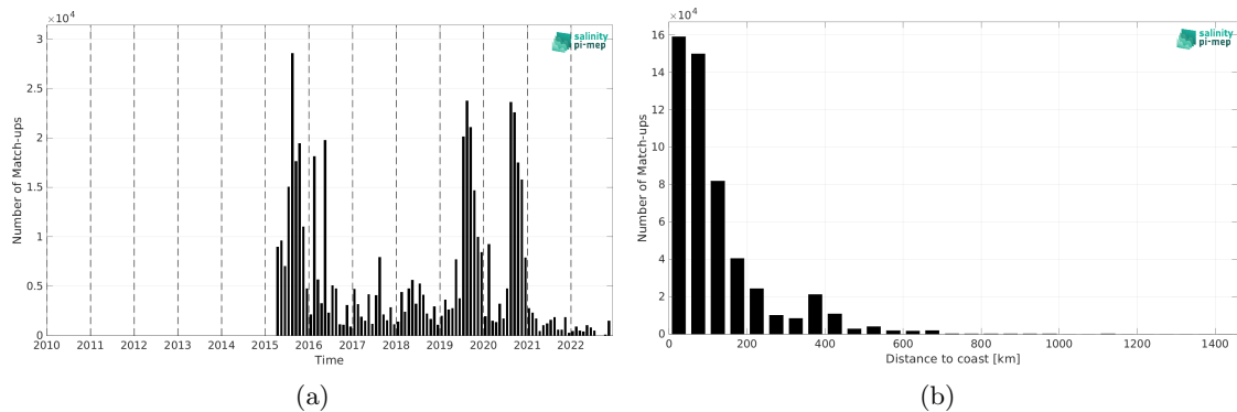
Figure 1: Number of match-ups between ICES and SMAP SSS L3 v5 - Monthly (RSS) SSS as a function of time (a) and as function of the distance to coast (b) over the Global Ocean Pi-MEP region and for the full satellite product period.
