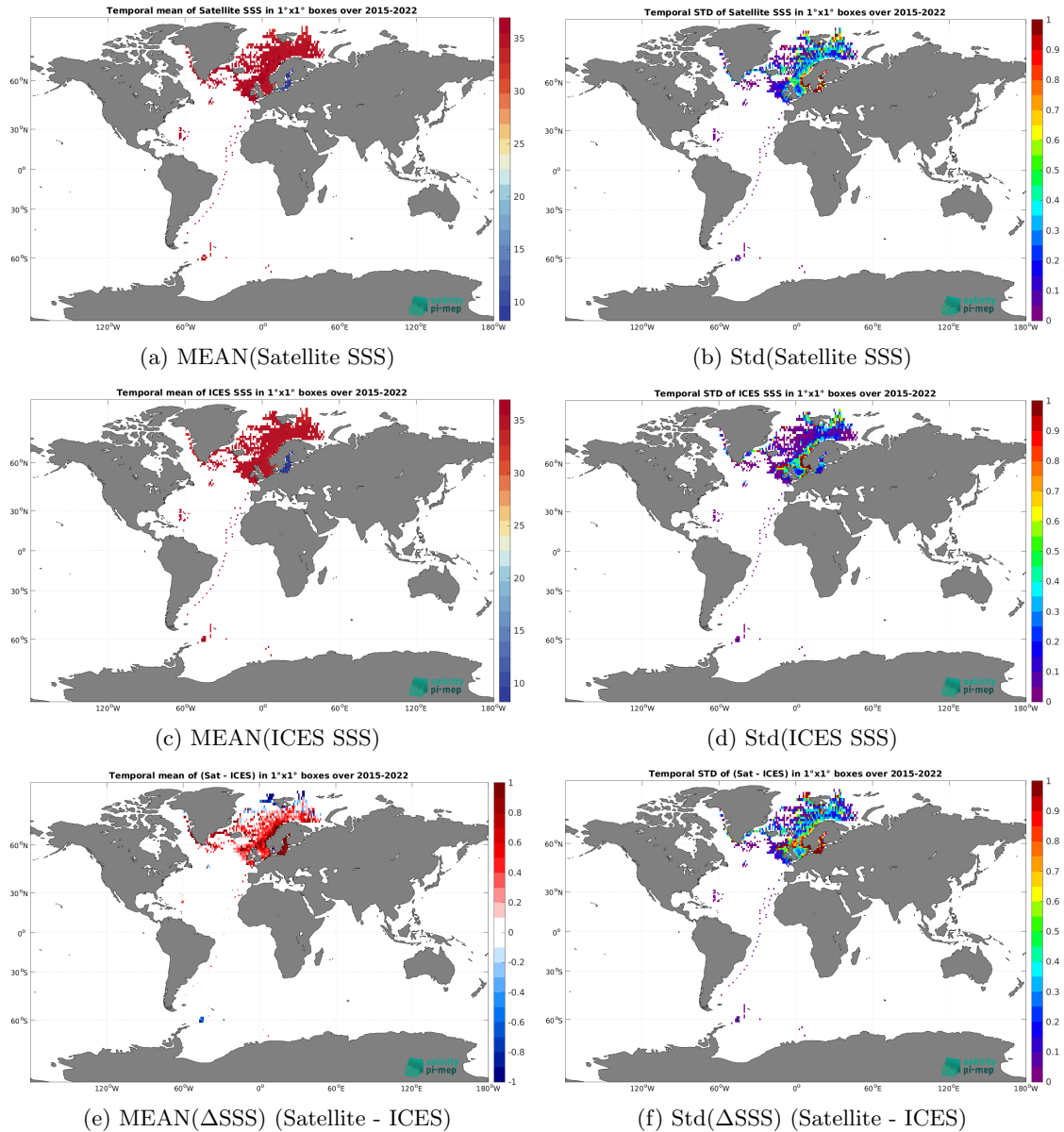
Figure 6: Temporal mean (left) and Std (right) of SSS from SMAP SSS L3 v5 - Monthly (RSS) (top), ICES (middle), and of \Delta SSS (Satellite - ICES). Only match-up pairs are used to generate these maps.
