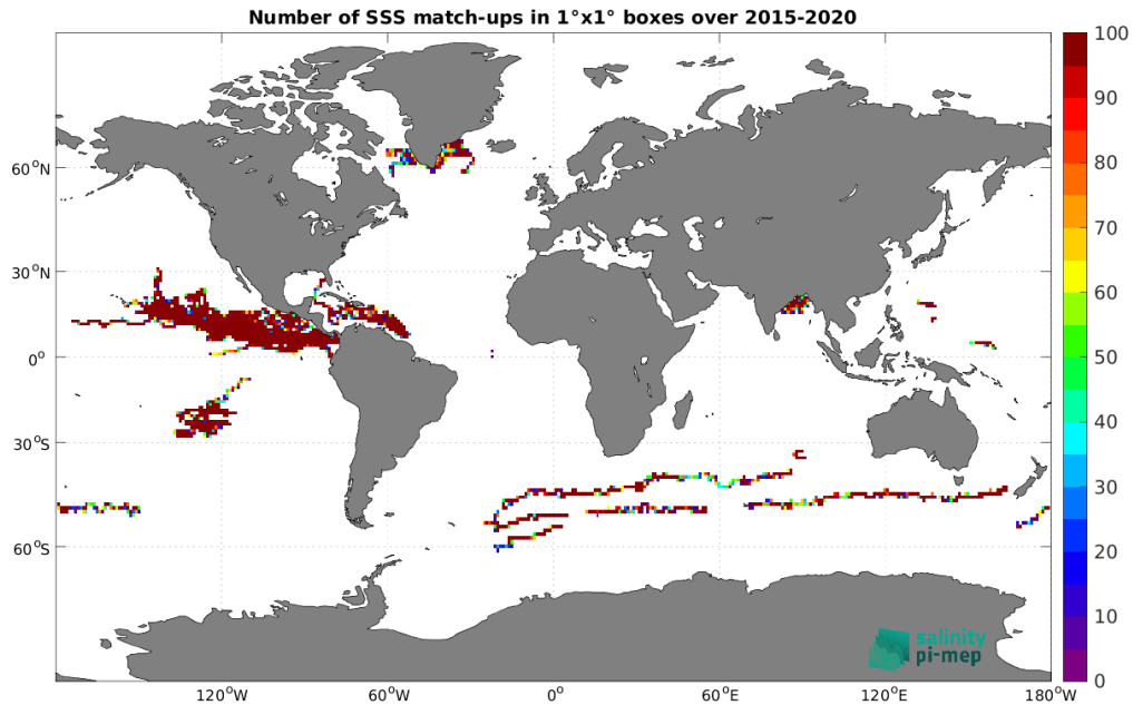
Figure 3: Number of SSS match-ups between Surface drifters SSS and the SMAP SSS L3 v5 - Monthly (RSS) SSS product for the Global Ocean Pi-MEP region over 1^\circ \times 1^\circ boxes and for the full satellite product period.
