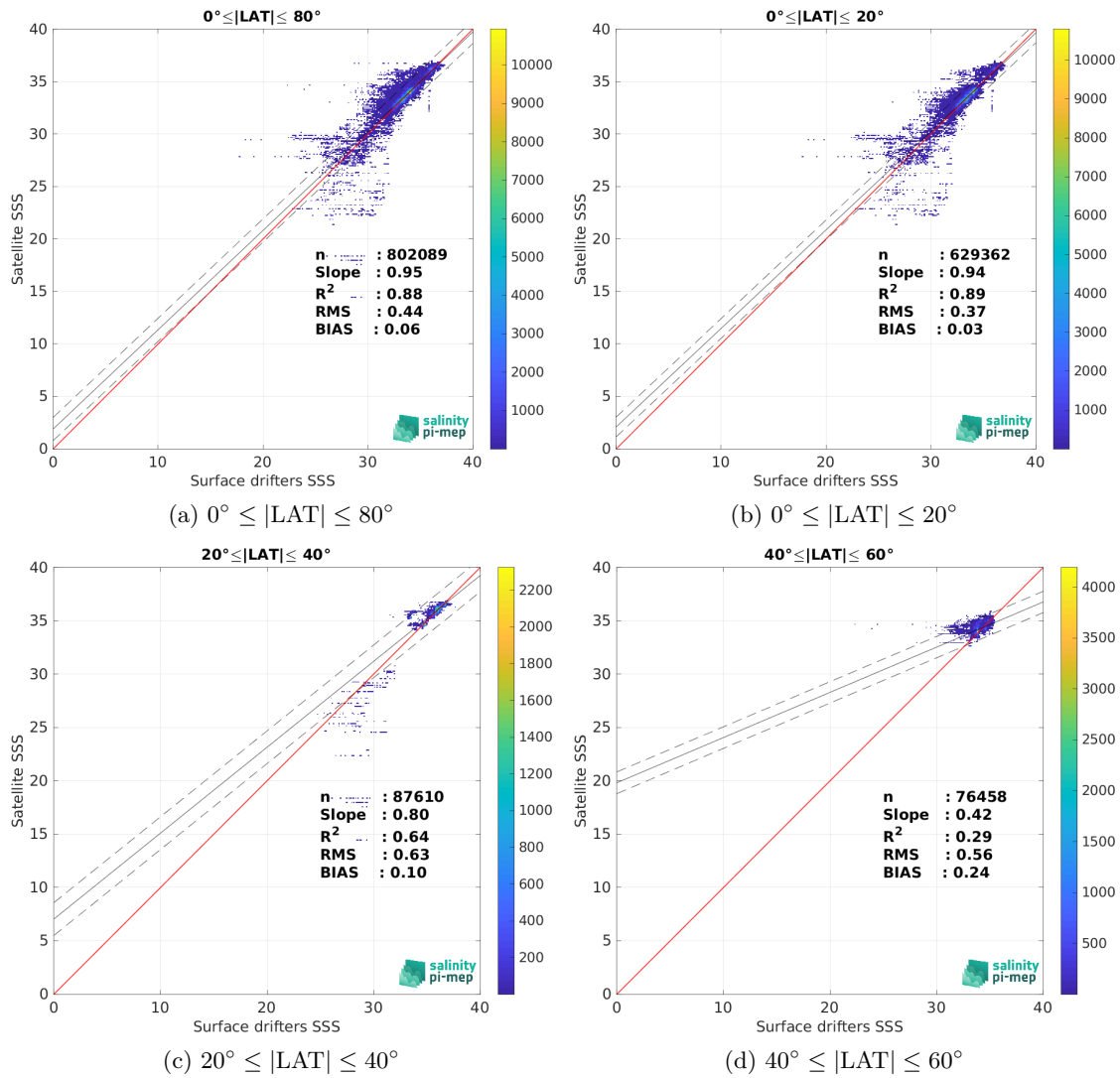
Figure 8: Contour maps of the concentration of SMAP SSS L3 v5 - Monthly (RSS) SSS (y-axis) versus Surface drifters SSS (x-axis) at match-up pairs for different latitude bands. For each plot, the red line shows x=y . The black thin and dashed lines indicate a linear fit through the data cloud and the \pm 95\% confidence levels, respectively. The number match-up pairs n , the slope and R^2 coefficient of the linear fit, the root mean square (RMS) and the mean bias between satellite and in situ data are indicated for each latitude band in each plots.
