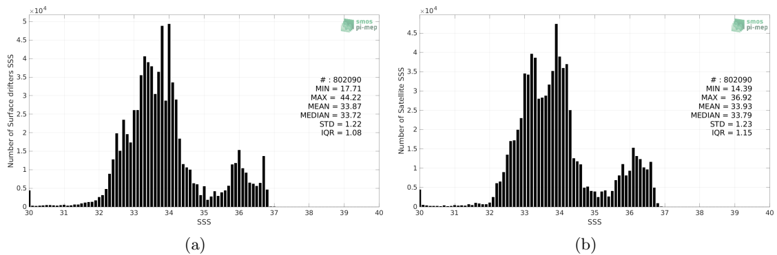
Figure 2: Histograms of SSS from Surface drifters (a) and SMAP SSS L3 v5 - Monthly (RSS) (b) considering all match-up pairs per bins of 0.1 over the Global Ocean Pi-MEP region and for the full satellite product period.
