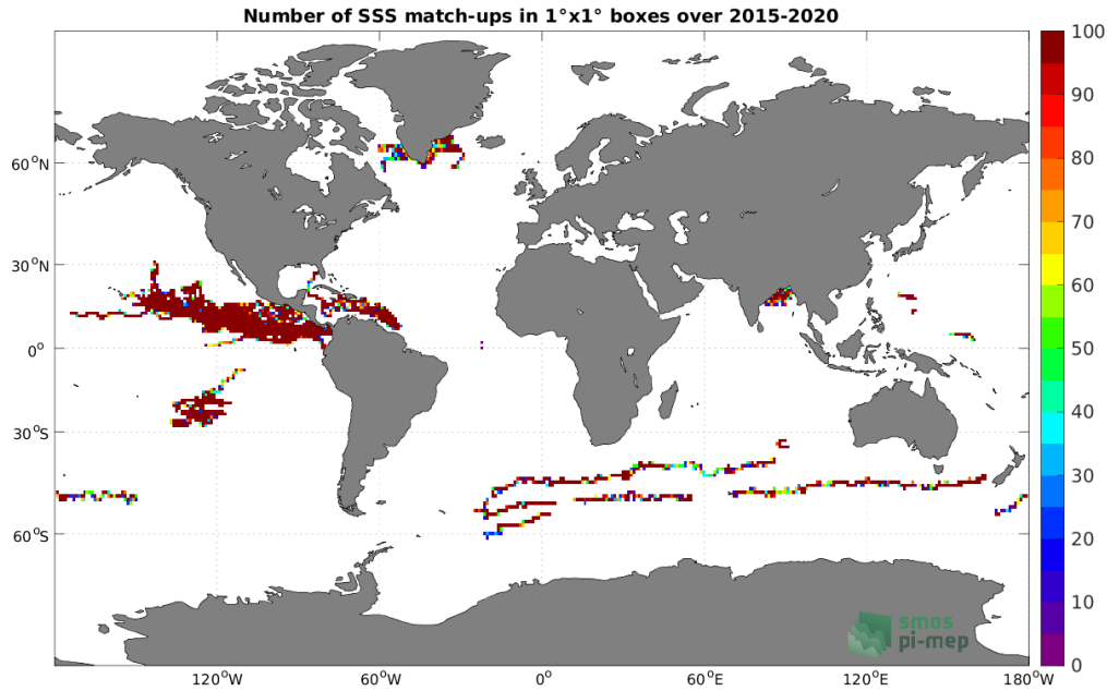
Figure 3: Number of SSS match-ups between Surface drifters SSS and the SMAP SSS L3 v5 - Monthly (RSS) SSS product for the Global Ocean Pi-MEP region over 1°×1° boxes and for the full satellite product period.
