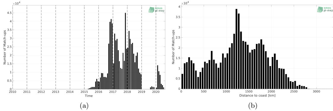
Figure 1: Number of match-ups between Surface drifters and SMAP SSS L3 v5 - Monthly (RSS) SSS as a function of time (a) and as function of the distance to coast (b) over the Global Ocean Pi-MEP region and for the full satellite product period.
