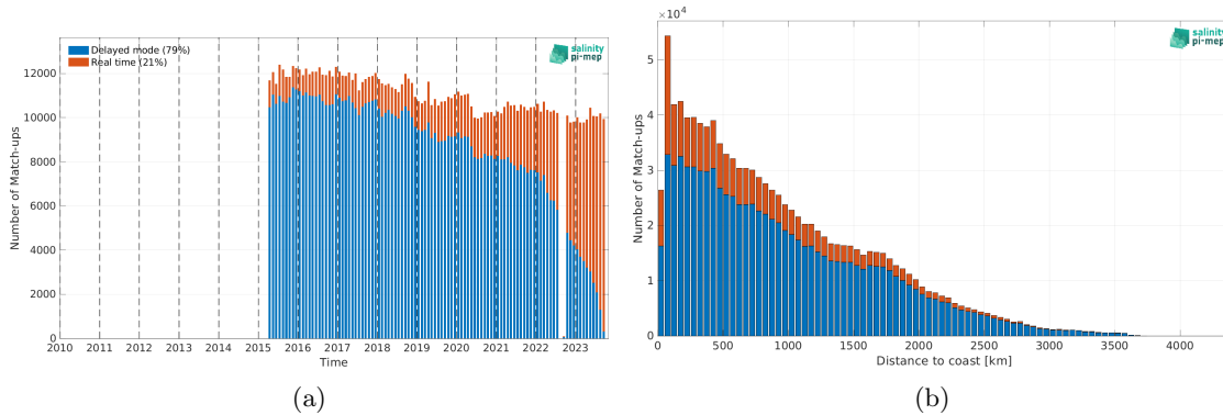
Figure 1: Number of match-ups between Argo and SMAP SSS L3 v5 - Monthly (RSS) SSS as a function of time (a) and as function of the distance to coast (b) over the Global Ocean Pi-MEP region and for the full satellite product period.
