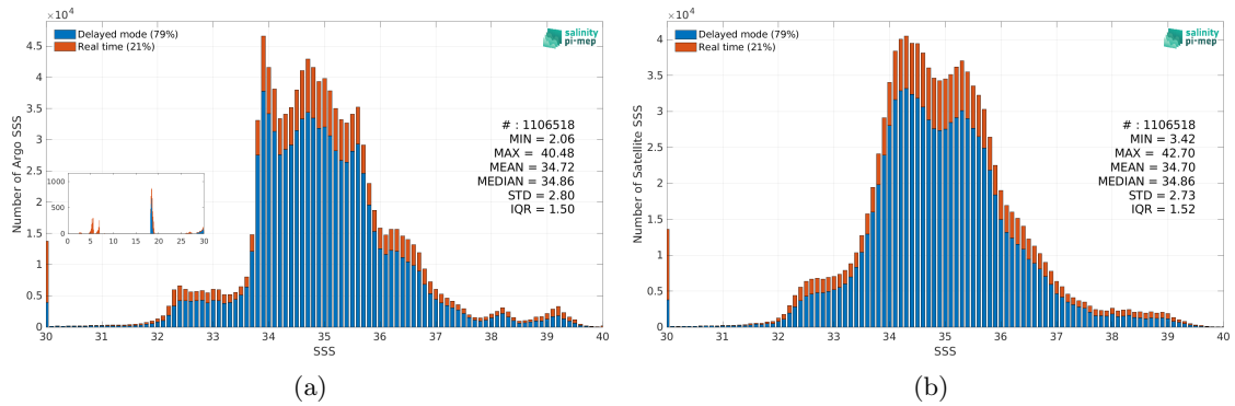
Figure 2: Histograms of SSS from Argo (a) and SMAP SSS L3 v5 - Monthly (RSS) (b) considering all match-up pairs per bins of 0.1 over the Global Ocean Pi-MEP region and for the full satellite product period.
