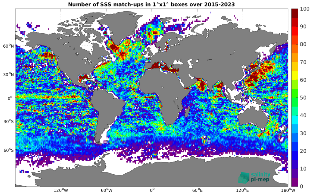
Figure 4: Number of SSS match-ups between Argo SSS and the SMAP SSS L3 v5 - Monthly (RSS) SSS product for the Global Ocean Pi-MEP region over 1^\circ \times 1^\circ boxes and for the full satellite product period.
