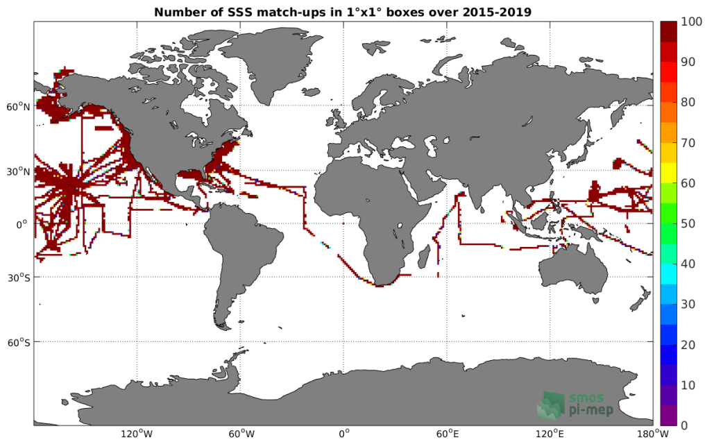
Figure 4: Number of SSS match-ups between TSG-SAMOS SSS and the SMAP-L3-RSS-V4-8DAY-RUNNING SSS product for the Global Ocean Pi-MEP region over 1^\circ \times 1^\circ boxes and for the full satellite product period.
