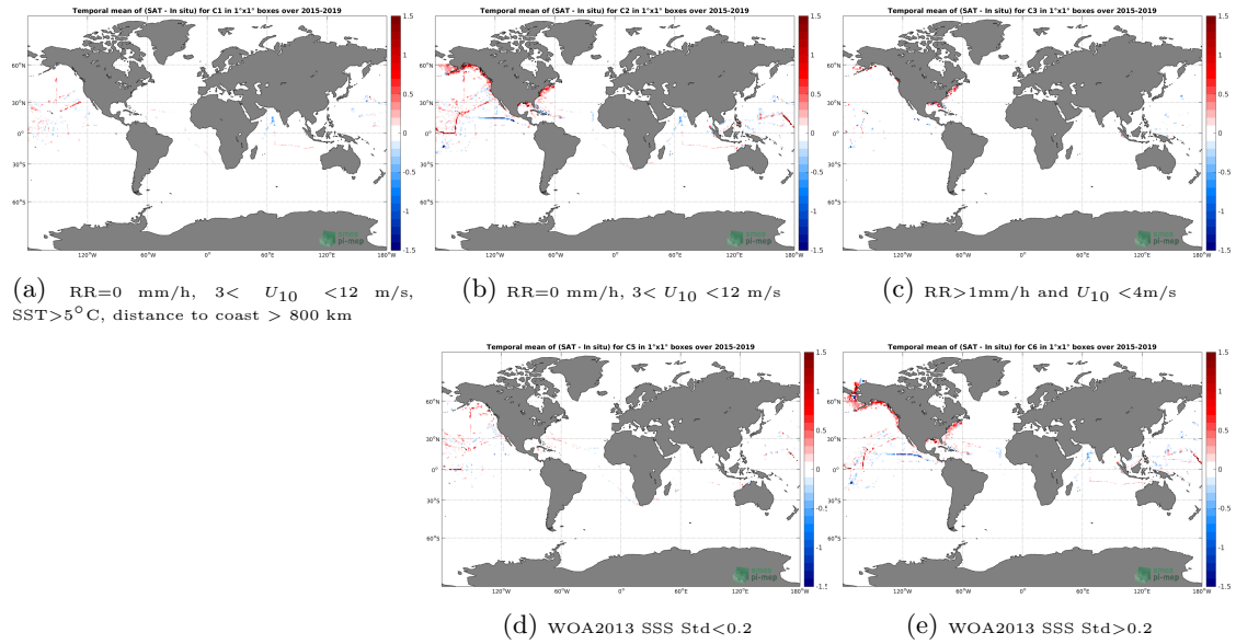
Figure 12: Temporal mean gridded over spatial boxes of size 1^\circ \times 1^\circ of \Delta SSS (SMAP-L3-RSS-V4-8DAY-RUNNING - TSG-SAMOS) for 5 different subdatasets corresponding to:RR=0 mm/h, 3 < U_{10} < 12 m/s, SST > 5^\circ\text{C} , distance to coast > 800 km (a), RR=0 mm/h, 3 < U_{10} < 12 m/s (b), RR > 1 mm/h and U_{10} < 4 m/s (c), WOA2013 SSS Std < 0.2 (d), WOA2013 SSS Std > 0.2 (e).
