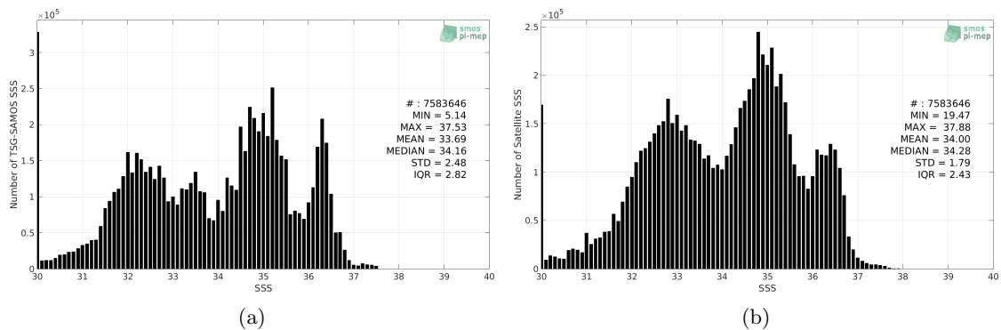
Figure 2: Histograms of SSS from TSG-SAMOS (a) and SMAP-L3-RSS-V4-8DAY-RUNNING (b) considering all match-up pairs per bins of 0.1 over the Global Ocean Pi-MEP region and for the full satellite product period.
