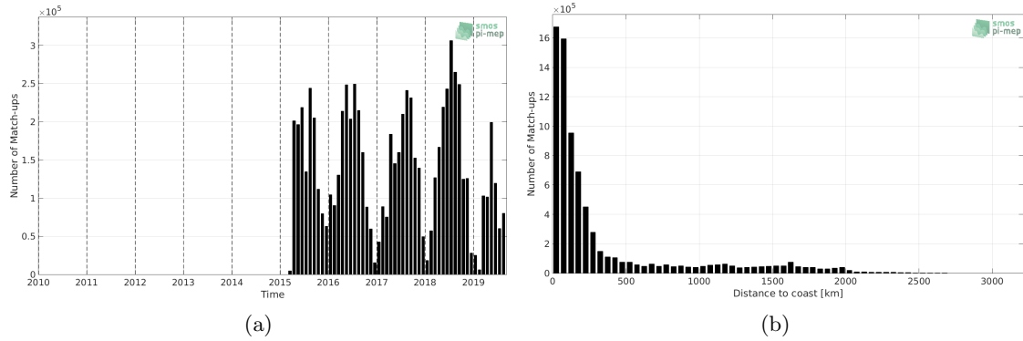
Figure 1: Number of match-ups between TSG-SAMOS and SMAP-L3-RSS-V4-8DAY-RUNNING SSS as a function of time (a) and as function of the distance to coast (b) over the Global Ocean Pi-MEP region and for the full satellite product period.
