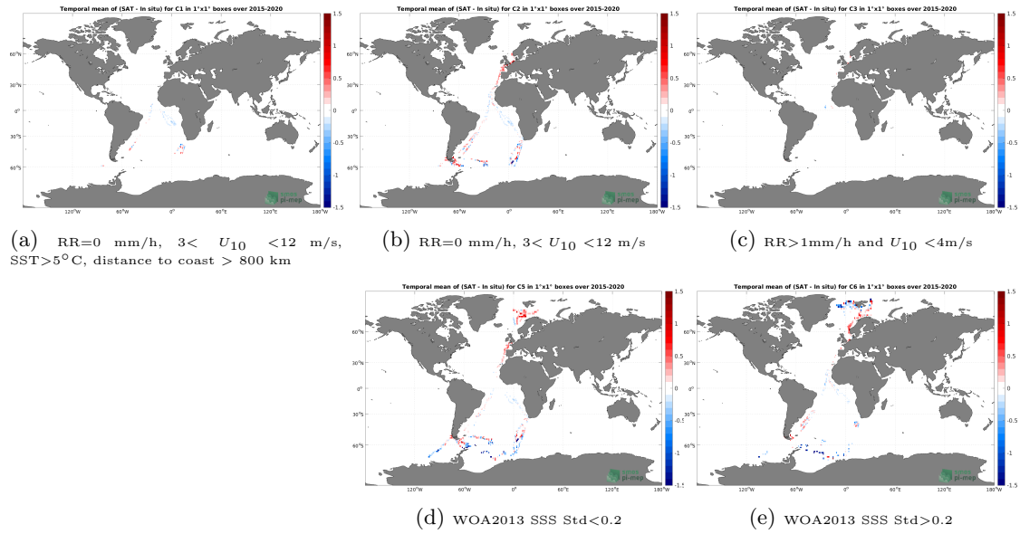
Figure 12: Temporal mean gridded over spatial boxes of size 1^\circ \times 1^\circ of \Delta SSS (SMAP SSS L3 v4 - 8-Day running (RSS) - TSG (Polarstern)) for 5 different subdatasets corresponding to:RR=0 mm/h, 3 < U_{10} < 12 m/s, SST >5^\circ C, distance to coast > 800 km (a), RR=0 mm/h, 3 < U_{10} < 12 m/s (b), RR >1 mm/h and U_{10} < 4 m/s (c), WOA2013 SSS Std <0.2 (d), WOA2013 SSS Std >0.2 (e).
