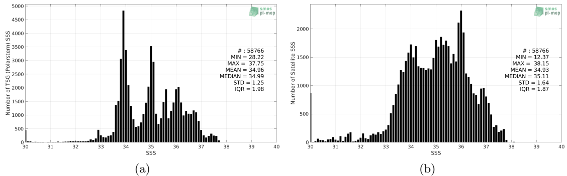
Figure 2: Histograms of SSS from TSG (Polarstern) (a) and SMAP SSS L3 v4 - 8-Day running (RSS) (b) considering all match-up pairs per bins of 0.1 over the Global Ocean Pi-MEP region and for the full satellite product period.
