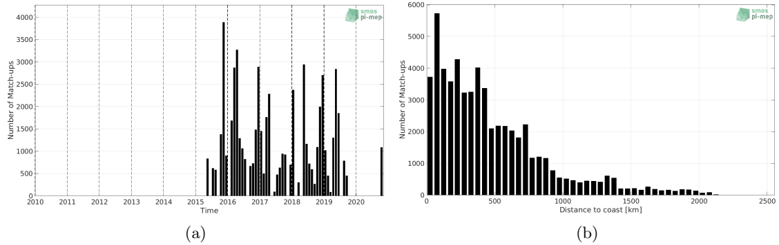
Figure 1: Number of match-ups between TSG (Polarstern) and SMAP SSS L3 v4 - 8-Day running (RSS) SSS as a function of time (a) and as function of the distance to coast (b) over the Global Ocean Pi-MEP region and for the full satellite product period.
