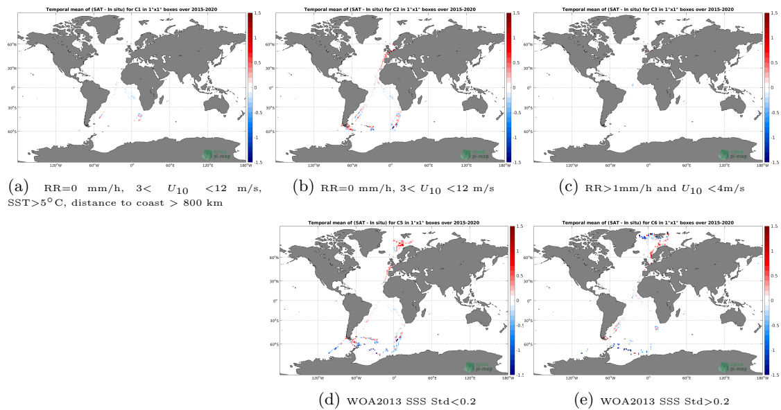
Figure 12: Temporal mean gridded over spatial boxes of size 1^\circ \times 1^\circ of \Delta\text{SSS} (SMAP SSS L3 v4 - 8-Day running (RSS) - TSG (Polarstern)) for 5 different subdatasets corresponding to:RR=0 mm/h, 3 < U_{10} < 12 m/s, SST > 5^\circ\text{C} , distance to coast > 800 km (a), RR=0 mm/h, 3 < U_{10} < 12 m/s (b), RR > 1 mm/h and U_{10} < 4 m/s (c), WOA2013 SSS Std < 0.2 (d), WOA2013 SSS Std > 0.2 (e).
