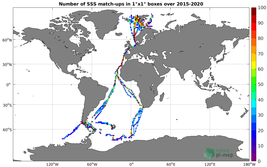
Figure 4: Number of SSS match-ups between TSG (Polarstern) SSS and the SMAP SSS L3 v4 - 8-Day running (RSS) SSS product for the Global Ocean Pi-MEP region over 1^\circ \times 1^\circ boxes and for the full satellite product period.
