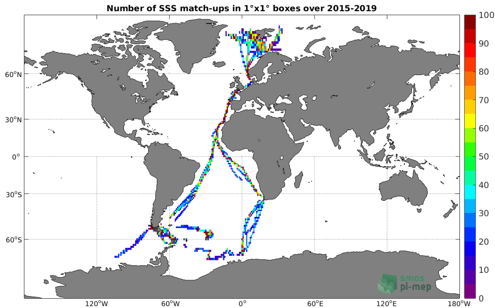
Figure 4: Number of SSS match-ups between TSG (Polarstern) SSS and the SMAP SSS L3 v4 - 8-Day running (RSS) SSS product for the Global Ocean Pi-MEP region over 1°x1° boxes and for the full satellite product period.
