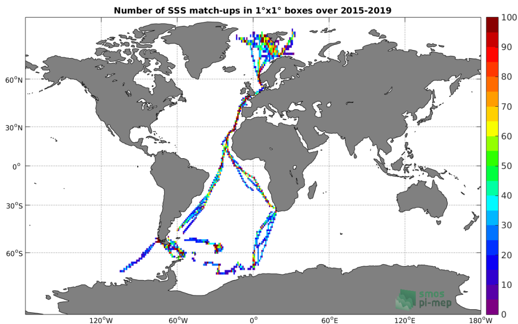
Figure 4: Number of SSS match-ups between TSG-POLARSTERN SSS and the SMAP-L3-RSS-V4-8DAY-RUNNING SSS product for the Global Ocean Pi-MEP region over 1^\circ \times 1^\circ boxes and for the full satellite product period.
