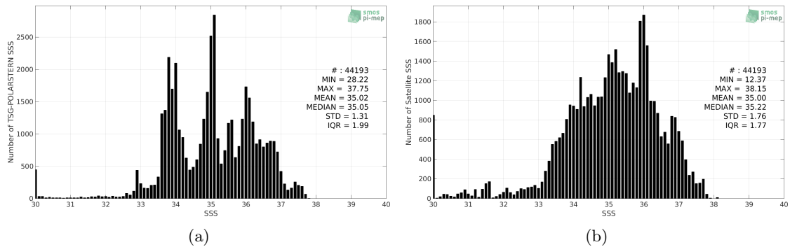
Figure 2: Histograms of SSS from TSG-POLARSTERN (a) and SMAP-L3-RSS-V4-8DAY-RUNNING (b) considering all match-up pairs per bins of 0.1 over the Global Ocean Pi-MEP region and for the full satellite product period.
