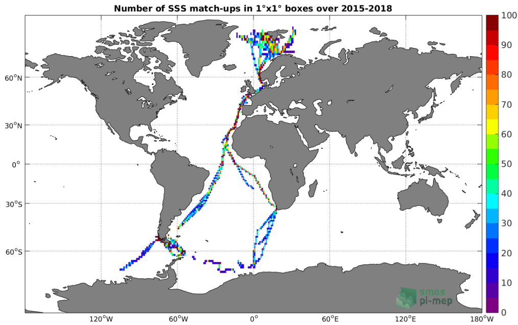
Figure 4: Number of SSS match-ups between TSG-POLARSTERN SSS and the SMAP-L3-RSS-V4-8DAY-RUNNING SSS product for the Global Ocean Pi-MEP region over 1°x1° boxes and for the full satellite product period.
