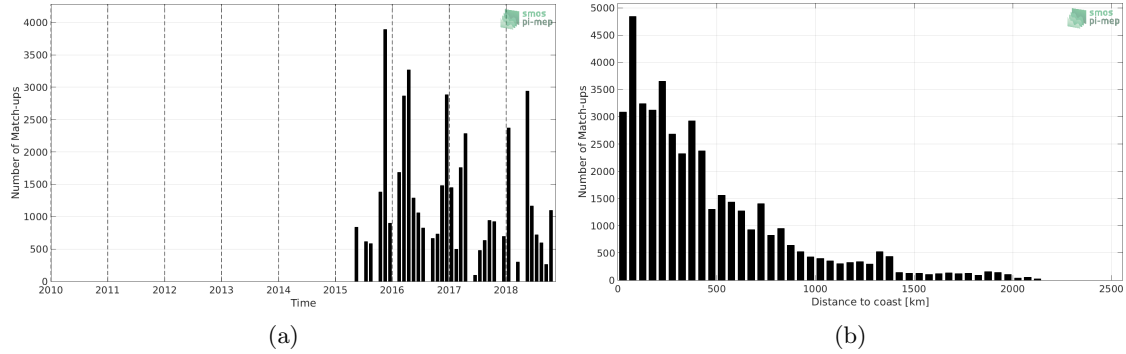
Figure 1: Number of match-ups between TSG-POLARSTERN and SMAP-L3-RSS-V4-8DAY-RUNNING SSS as a function of time (a) and as function of the distance to coast (b) over the Global Ocean Pi-MEP region and for the full satellite product period.
