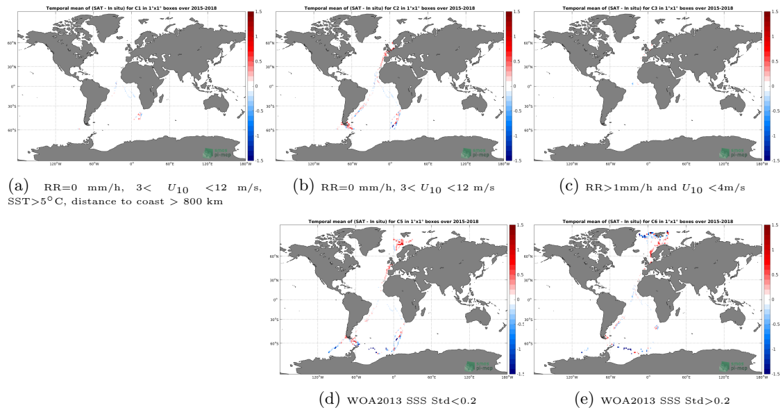
Figure 12: Temporal mean gridded over spatial boxes of size 1^\circ \times 1^\circ of \Delta SSS (SMAP-L3-RSS-V4-8DAY-RUNNING - TSG-POLARSTERN) for 5 different subdatasets corresponding to:RR=0 mm/h, 3 < U_{10} < 12 m/s, SST >5^\circ C, distance to coast > 800 km (a), RR=0 mm/h, 3 < U_{10} < 12 m/s (b), RR >1 mm/h and U_{10} < 4 m/s (c), WOA2013 SSS Std <0.2 (d), WOA2013 SSS Std >0.2 (e).
