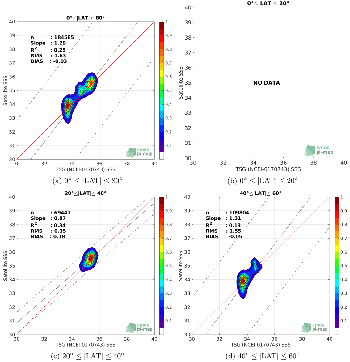
Figure 9: Contour maps of the concentration of SMAP SSS L3 v4 - 8-Day running (RSS) SSS (y-axis) versus TSG (NCEI-0170743) SSS (x-axis) at match-up pairs for different latitude bands. For each plot, the red line shows x=y . The black thin and dashed lines indicate a linear fit through the data cloud and the \pm 95\% confidence levels, respectively. The number match-up pairs n , the slope and R^2 coefficient of the linear fit, the root mean square (RMS) and the mean bias between satellite and in situ data are indicated for each latitude band in each plots.
