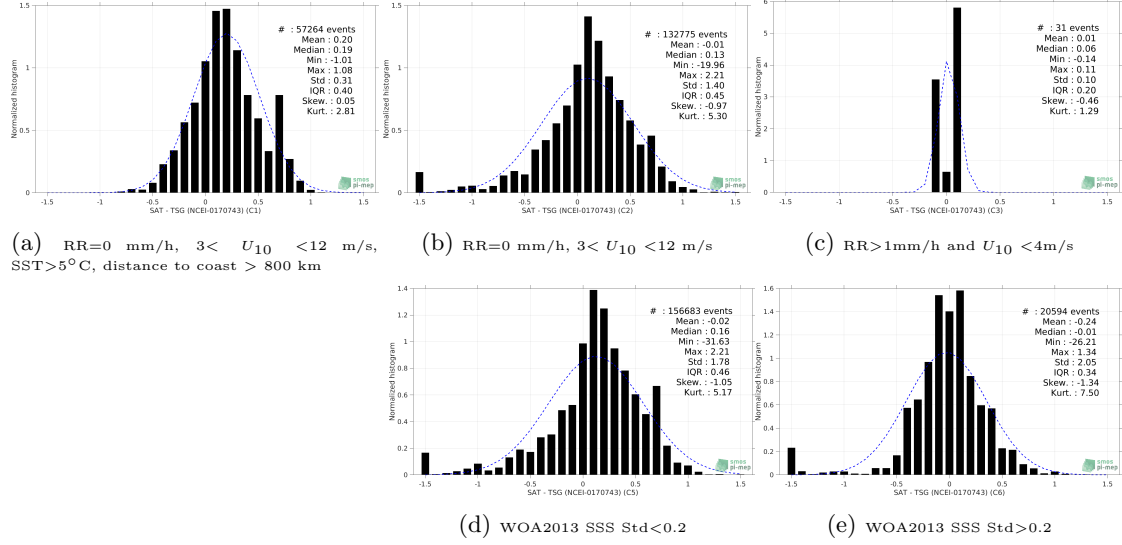
Figure 13: Normalized histogram of \Delta SSS (SMAP SSS L3 v4 - 8-Day running (RSS) - TSG (NCEI-0170743)) for 5 different subdatasets corresponding to: RR=0 mm/h, 3 < U_{10} < 12 m/s, SST>5°C, distance to coast > 800 km (a), RR=0 mm/h, 3 < U_{10} < 12 m/s (b), RR>1mm/h and U_{10} < 4 m/s (c), WOA2013 SSS Std<0.2 (d), WOA2013 SSS Std>0.2 (e).
