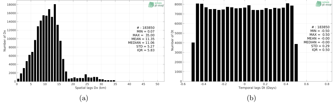
Figure 5: Histograms of the spatial (a) and temporal (b) lags between the time of the TSG (NCEI-0170743) measurements and the date of the corresponding SMAP SSS L3 v4 - 8-Day running (RSS) SSS product.
