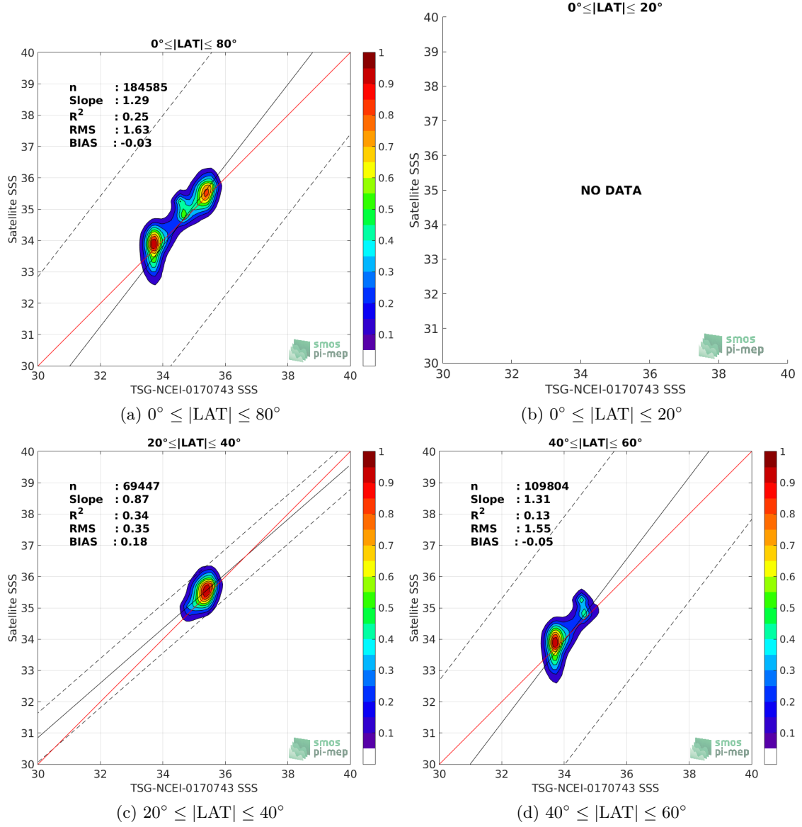
Figure 9: Contour maps of the concentration of SMAP-L3-RSS-V4-8DAY-RUNNING SSS (y-axis) versus TSG-NCEI-0170743 SSS (x-axis) at match-up pairs for different latitude bands. For each plot, the red line shows x=y . The black thin and dashed lines indicate a linear fit through the data cloud and the \pm 95\% confidence levels, respectively. The number match-up pairs n , the slope and R^2 coefficient of the linear fit, the root mean square (RMS) and the mean bias between satellite and in situ data are indicated for each latitude band in each plots.
