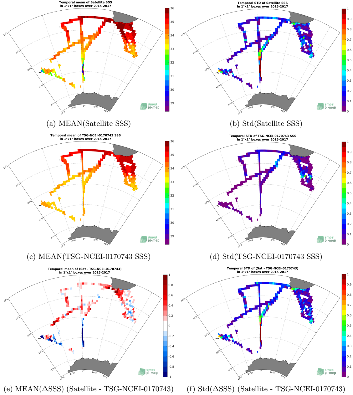
Figure 6: Temporal mean (left) and Std (right) of SSS from SMAP-L3-RSS-V4-8DAY-RUNNING (top), TSG-NCEI-0170743 (middle), and of \Delta SSS (Satellite - TSG-NCEI-0170743). Only match-up pairs are used to generate these maps.
