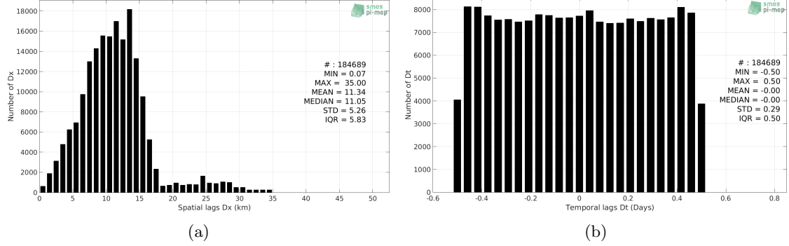
Figure 5: Histograms of the spatial (a) and temporal (b) lags between the time of the TSG-NCEI-0170743 measurements and the date of the corresponding SMAP-L3-RSS-V4-8DAY-RUNNING SSS product.
