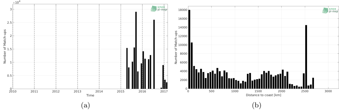
Figure 1: Number of match-ups between TSG-NCEI-0170743 and SMAP-L3-RSS-V4-8DAY-RUNNING SSS as a function of time (a) and as function of the distance to coast (b) over the Global Ocean Pi-MEP region and for the full satellite product period.
