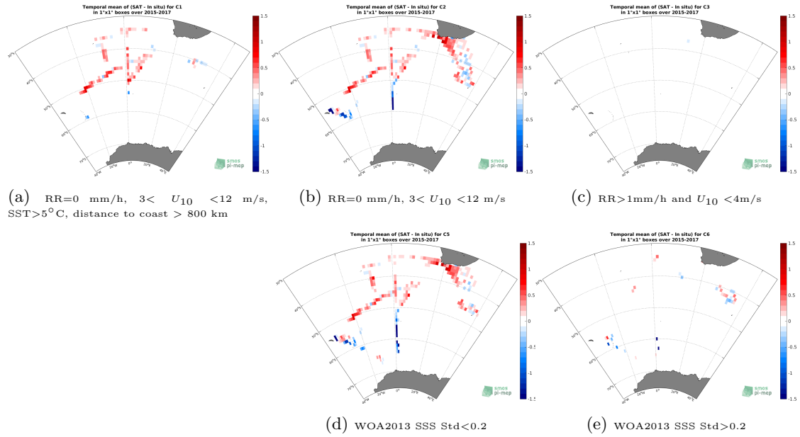
Figure 12: Temporal mean gridded over spatial boxes of size 1^\circ \times 1^\circ of \Delta SSS (SMAP-L3-RSS-V4-8DAY-RUNNING - TSG-NCEI-0170743) for 5 different subdatasets corresponding to: RR=0 mm/h, 3 < U_{10} < 12 m/s, SST >5^\circ C, distance to coast > 800 km (a), RR=0 mm/h, 3 < U_{10} < 12 m/s (b), RR >1 mm/h and U_{10} < 4 m/s (c), WOA2013 SSS Std <0.2 (d), WOA2013 SSS Std >0.2 (e).
