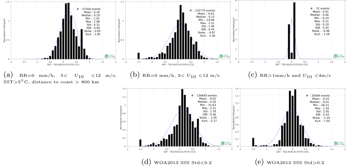
Figure 13: Normalized histogram of \Delta SSS (SMAP-L3-RSS-V4-8DAY-RUNNING - TSG-NCEI-0170743) for 5 different subdatasets corresponding to: RR=0 mm/h, 3 < U_{10} < 12 m/s, SST>5°C, distance to coast > 800 km (a), RR=0 mm/h, 3 < U_{10} < 12 m/s (b), RR>1mm/h and U_{10} < 4 m/s (c), WOA2013 SSS Std<0.2 (d), WOA2013 SSS Std>0.2 (e).
