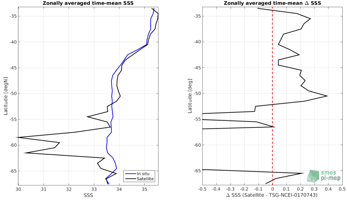
Figure 8: Left panel: Zonal mean SSS from SMAP-L3-RSS-V4-8DAY-RUNNING satellite product (black) and from TSG-NCEI-0170743 (blue). Right panel: Zonal mean of \Delta SSS (Satellite - TSG-NCEI-0170743) for all the collected Pi-MEP match-up pairs estimated over the full satellite product period.
