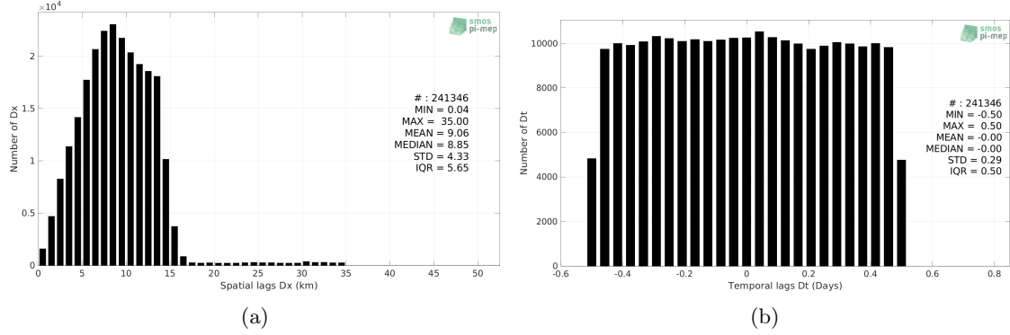
Figure 5: Histograms of the spatial (a) and temporal (b) lags between the location/time of the TSG (LEGOS-Survostral) measurement and the date of the corresponding SMAP SSS L3 v4 - 8-Day running (RSS) SSS pixel.
