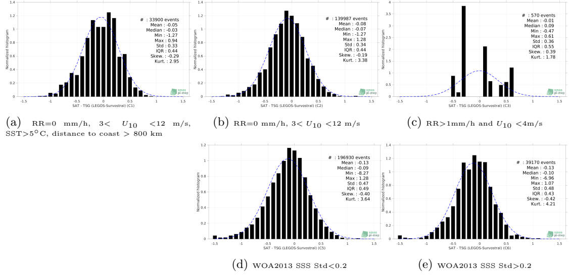
Figure 13: Normalized histogram of \Delta SSS (SMAP SSS L3 v4 - 8-Day running (RSS) - TSG (LEGOS-Survostral)) for 5 different subdatasets corresponding to: RR=0 mm/h, 3 < U_{10} < 12 m/s, SST > 5°C, distance to coast > 800 km (a), RR=0 mm/h, 3 < U_{10} < 12 m/s (b), RR > 1mm/h and U_{10} < 4 m/s (c), WOA2013 SSS Std < 0.2 (d), WOA2013 SSS Std > 0.2 (e).
