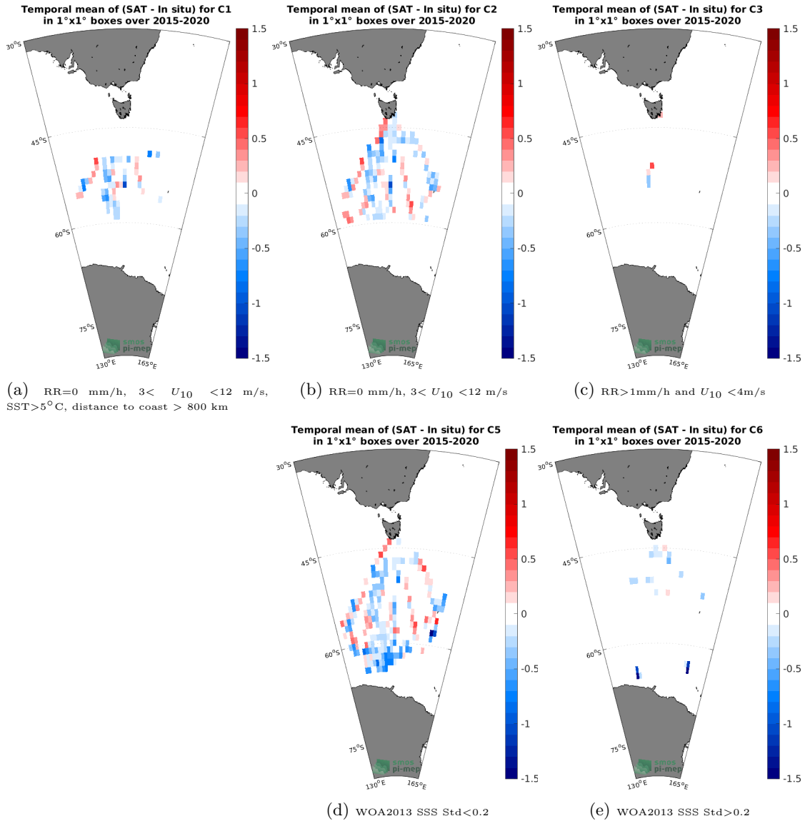
Figure 12: Temporal mean gridded over spatial boxes of size 1^\circ \times 1^\circ of \Delta SSS (SMAP SSS L3 v4 - 8-Day running (RSS) - TSG (LEGOS-Survostral)) for 5 different subdatasets corresponding to:RR=0 mm/h, 3 < U_{10} < 12 m/s, SST>5°C, distance to coast > 800 km (a), RR=0 mm/h, 3 < U_{10} < 12 m/s (b), RR>1mm/h and U_{10} < 4 m/s (c), WOA2013 SSS Std<0.2 (d), WOA2013 SSS Std>0.2 (e).
