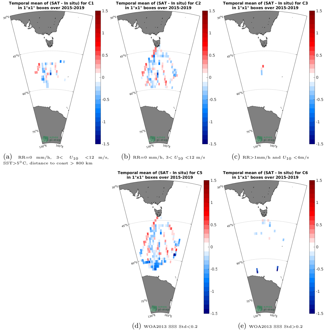
Figure 12: Temporal mean gridded over spatial boxes of size 1^\circ \times 1^\circ of \Delta\text{SSS} (SMAP-L3-RSS-V4-8DAY-RUNNING - TSG-LEGOS-Survostral) for 5 different subdatasets corresponding to: RR=0 mm/h, 3 < U_{10} < 12 m/s, SST > 5^\circ\text{C} , distance to coast > 800 km (a), RR=0 mm/h, 3 < U_{10} < 12 m/s (b), RR > 1\text{mm/h} and U_{10} < 4\text{m/s} (c), WOA2013 SSS Std < 0.2 (d), WOA2013 SSS Std > 0.2 (e).
