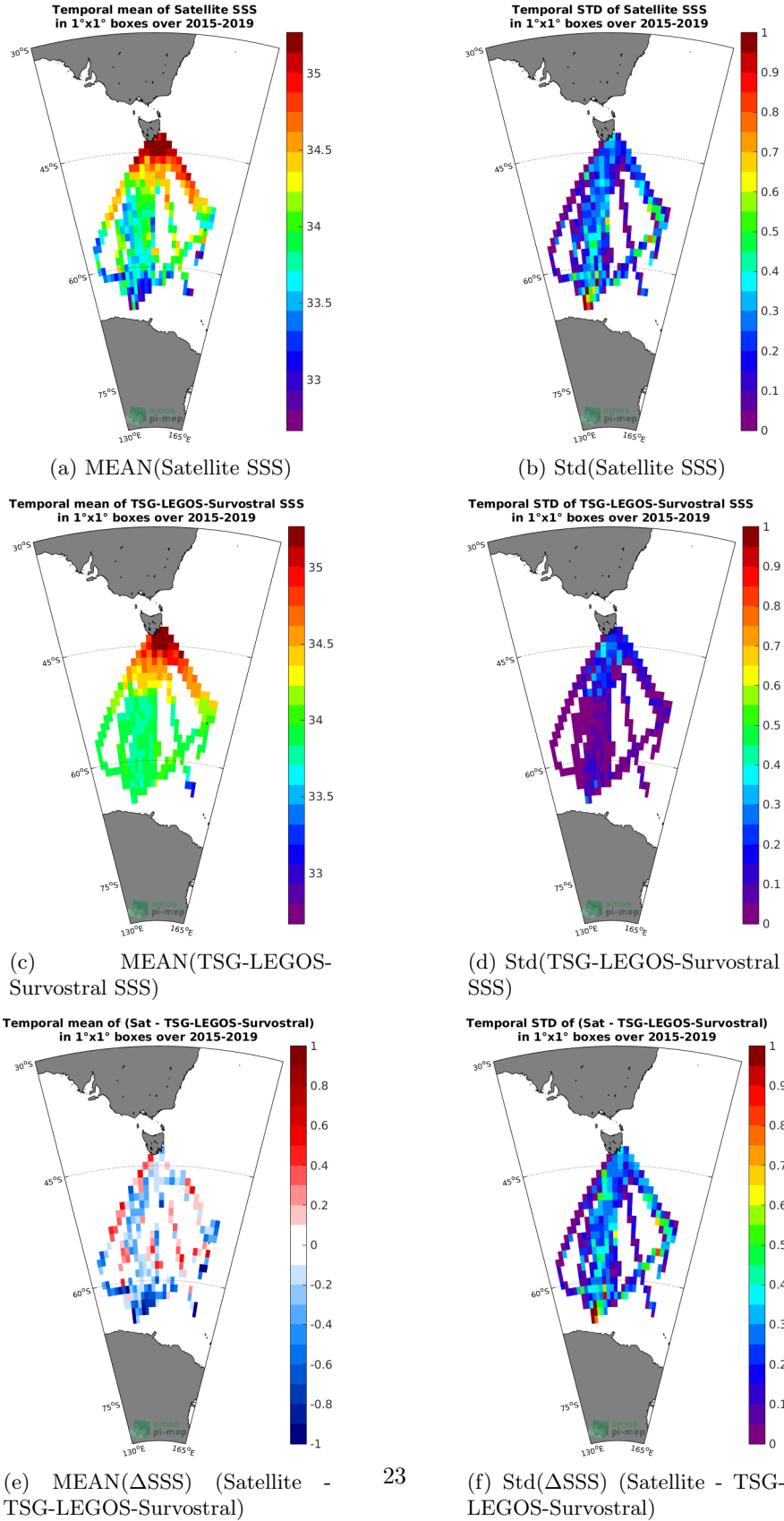
Figure 6: Temporal mean (left) and Std (right) of SSS from SMAP-L3-RSS-V4-8DAY-RUNNING (top), TSG-LEGOS-Survostral (middle), and of \Delta SSS (Satellite - TSG-LEGOS-Survostral). Only match-up pairs are used to generate these maps.
