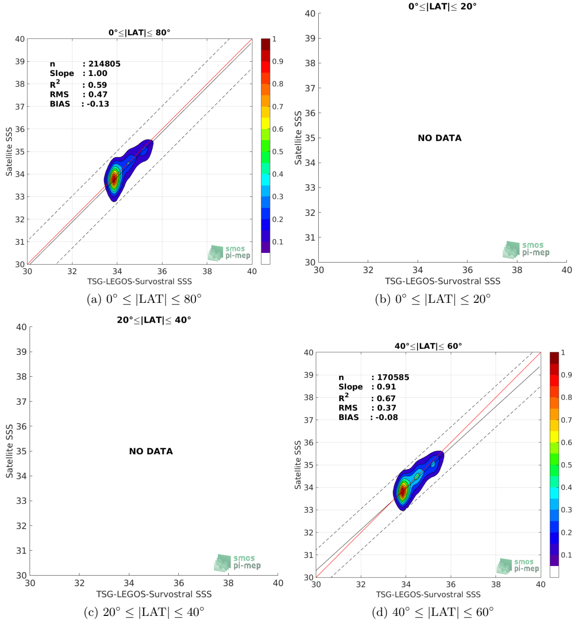
Figure 9: Contour maps of the concentration of SMAP-L3-RSS-V4-8DAY-RUNNING SSS (y-axis) versus TSG-LEGOS-Survostral SSS (x-axis) at match-up pairs for different latitude bands. For each plot, the red line shows x=y . The black thin and dashed lines indicate a linear fit through the data cloud and the \pm 95\% confidence levels, respectively. The number match-up pairs n , the slope and R^2 coefficient of the linear fit, the root mean square (RMS) and the mean bias between satellite and in situ data are indicated for each latitude band in each plots.
