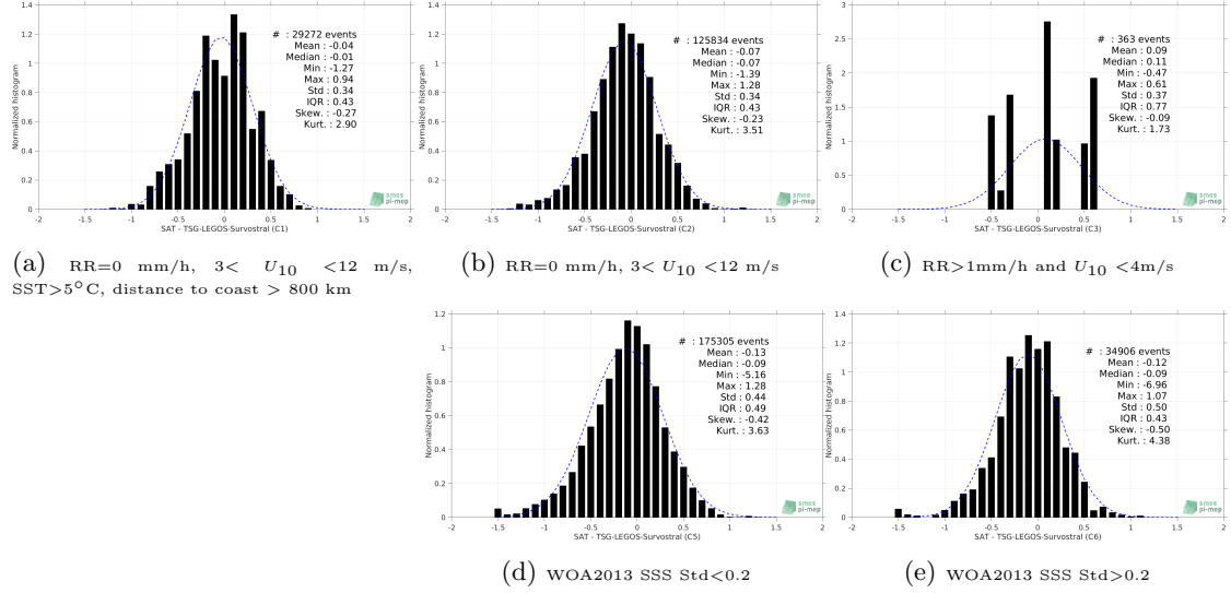
Figure 13: Normalized histogram of \Delta SSS (SMAP-L3-RSS-V4-8DAY-RUNNING - TSG-LEGOS-Survostral) for 5 different subdatasets corresponding to: RR=0 mm/h, 3 < U_{10} < 12 m/s, SST > 5°C, distance to coast > 800 km (a), RR=0 mm/h, 3 < U_{10} < 12 m/s (b), RR > 1mm/h and U_{10} < 4 m/s (c), WOA2013 SSS Std < 0.2 (d), WOA2013 SSS Std > 0.2 (e).
