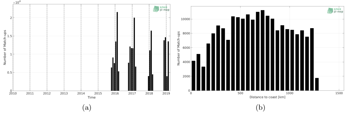
Figure 1: Number of match-ups between TSG-LEGOS-Survostral and SMAP-L3-RSS-V4-8DAY-RUNNING SSS as a function of time (a) and as function of the distance to coast (b) over the Global Ocean Pi-MEP region and for the full satellite product period.
