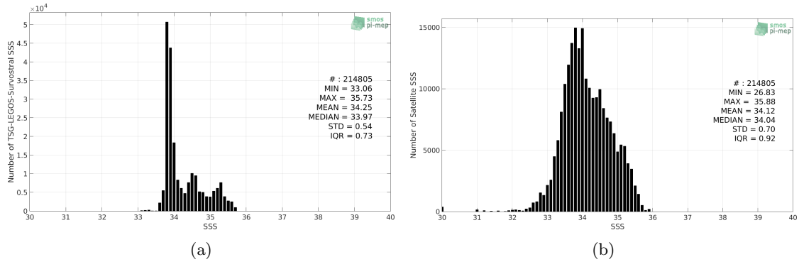
Figure 2: Histograms of SSS from TSG-LEGOS-Survostral (a) and SMAP-L3-RSS-V4-8DAY-RUNNING (b) considering all match-up pairs per bins of 0.1 over the Global Ocean Pi-MEP region and for the full satellite product period.
