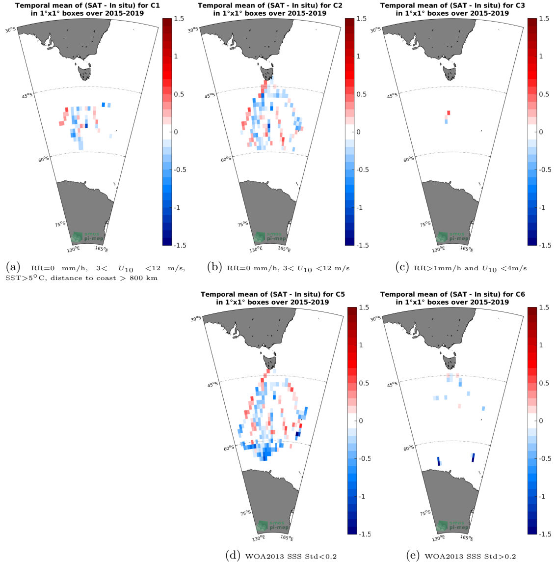
Figure 12: Temporal mean gridded over spatial boxes of size 1°x1° of \Delta\text{SSS} (SMAP-L3-RSS-V4-8DAY-RUNNING - TSG-LEGOS-Survostral) for 5 different subdatasets corresponding to: RR=0 mm/h, 3 < U_{10} < 12 m/s, SST > 5^\circ\text{C} , distance to coast > 800 km (a), RR=0 mm/h, 3 < U_{10} < 12 m/s (b), RR > 1\text{mm/h} and U_{10} < 4\text{m/s} (c), WOA2013 SSS Std < 0.2 (d), WOA2013 SSS Std > 0.2 (e).
