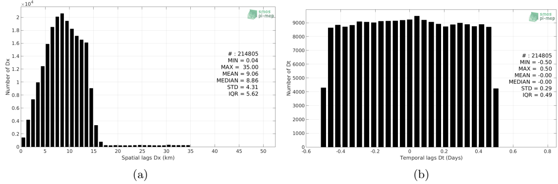
Figure 5: Histograms of the spatial (a) and temporal (b) lags between the time of the TSG-LEGOS-Survostral measurements and the date of the corresponding SMAP-L3-RSS-V4-8DAY-RUNNING SSS product.
