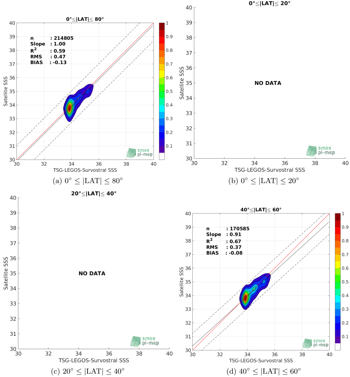
Figure 9: Contour maps of the concentration of SMAP-L3-RSS-V4-8DAY-RUNNING SSS (y-axis) versus TSG-LEGOS-Survostral SSS (x-axis) at match-up pairs for different latitude bands. For each plot, the red line shows x=y . The black thin and dashed lines indicate a linear fit through the data cloud and the \pm 95\% confidence levels, respectively. The number match-up pairs n , the slope and R^2 coefficient of the linear fit, the root mean square (RMS) and the mean bias between satellite and in situ data are indicated for each latitude band in each plots.
